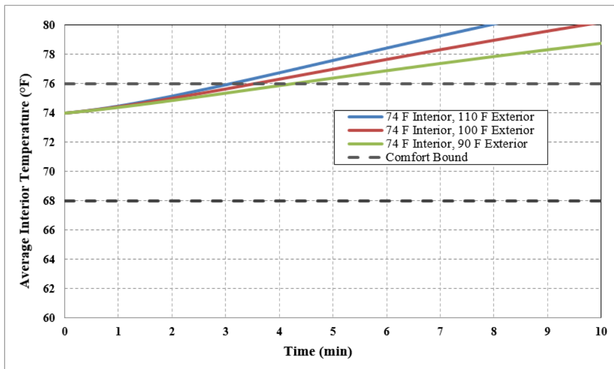
Figure 2.11. Time to increase interior temperature out of comfort zone in cooling season with 74 °F initial interior temperature
