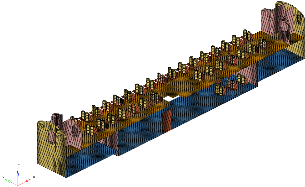
Figure 2.8. Isometric view of the car interior
