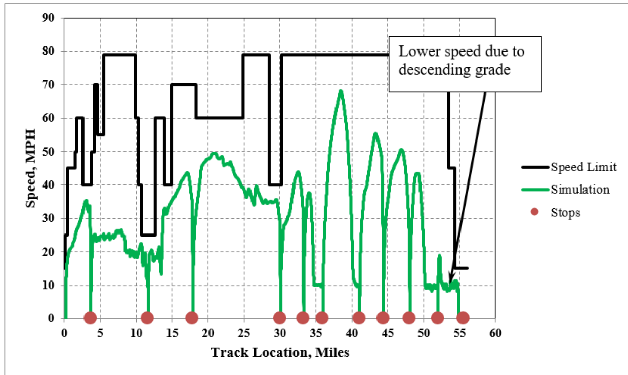
Figure 2.5. Commuter route speed limit and simulated speed
