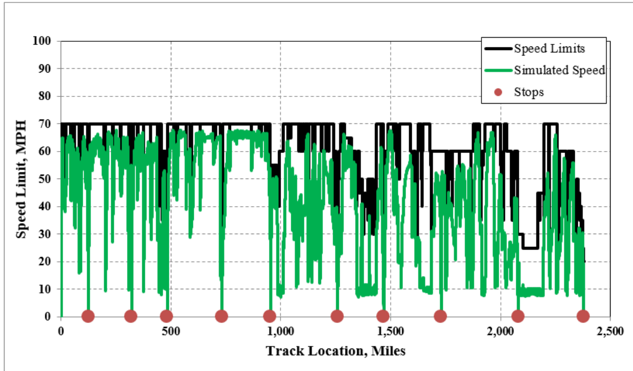
Figure 2.6. Long-haul route speed limit and simulated speed
