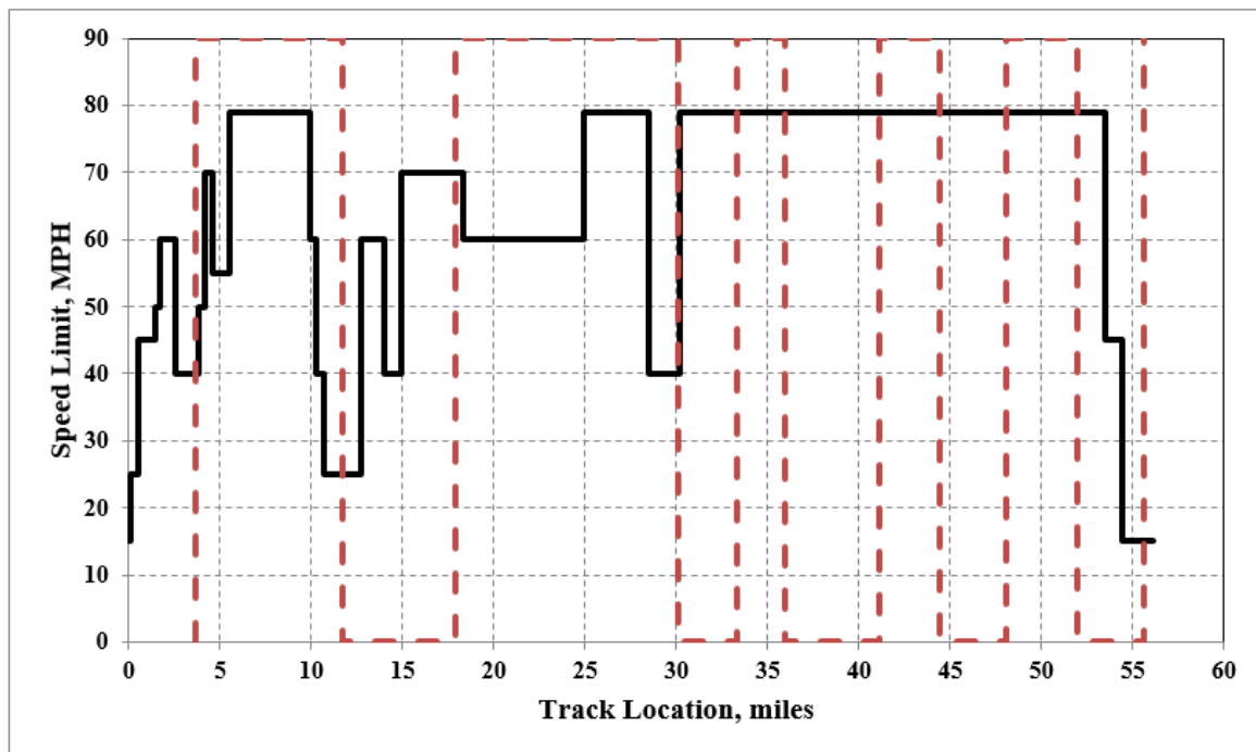
Figure 2.2. Commuter route speed limit locations
