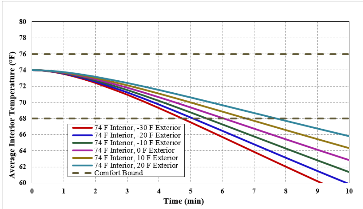
Figure 2.14. Time to decrease interior temperature out of comfort zone in heating season with 74 °F initial interior temperature
