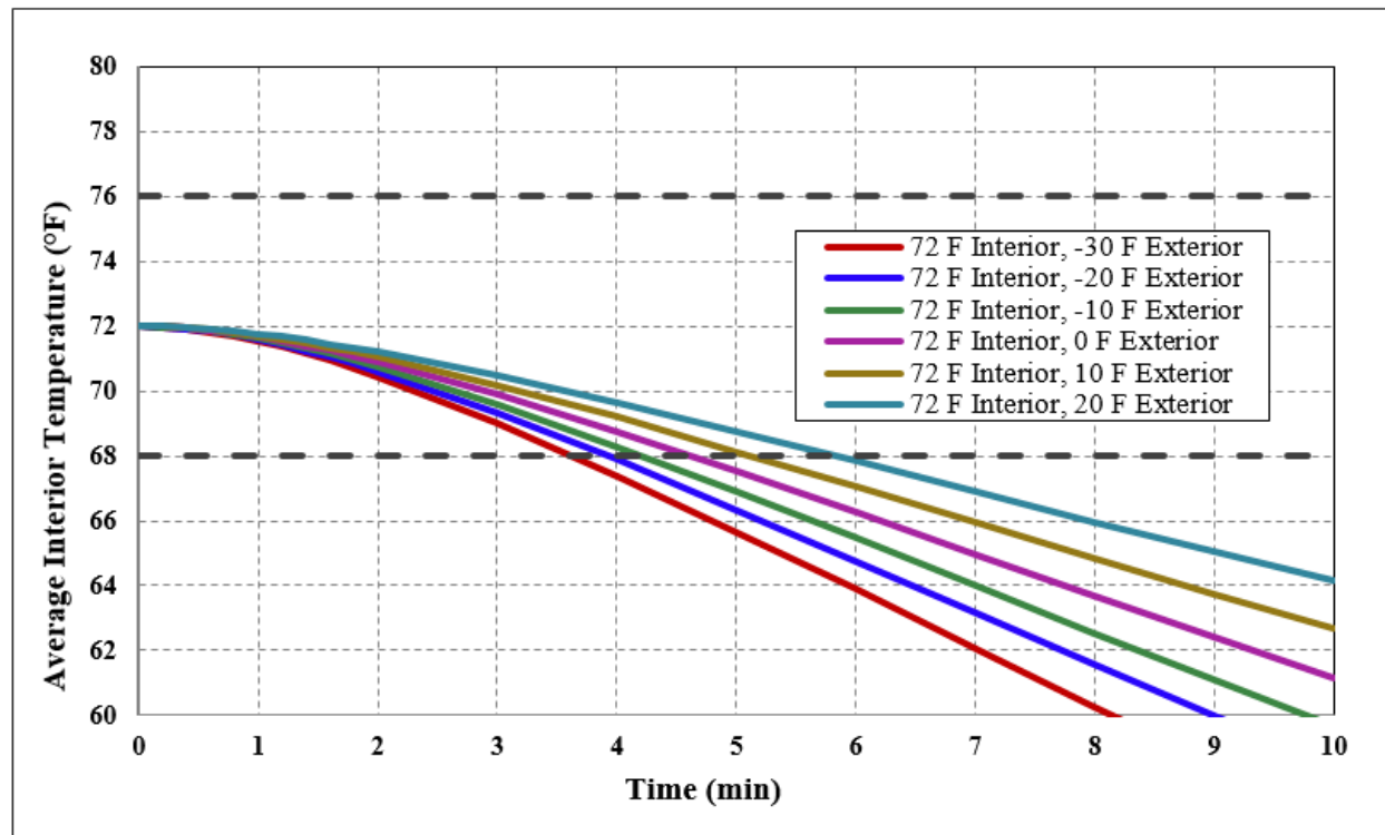
Figure 2.13. Time to decrease interior temperature out of comfort zone in heating season with 74 °F initial interior temperature
