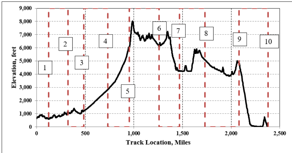
Figure 2.3. Long-haul route elevation profile, including the stops along the route
