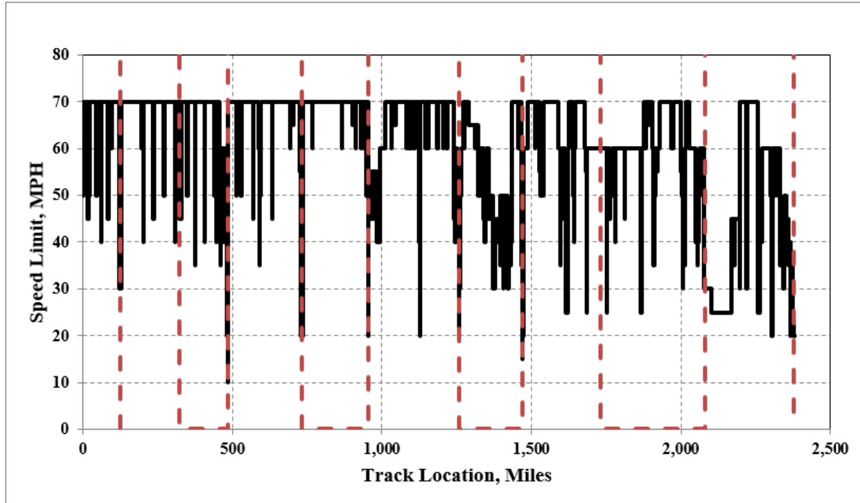
Figure 2.4. Long-haul route speed limit profile
