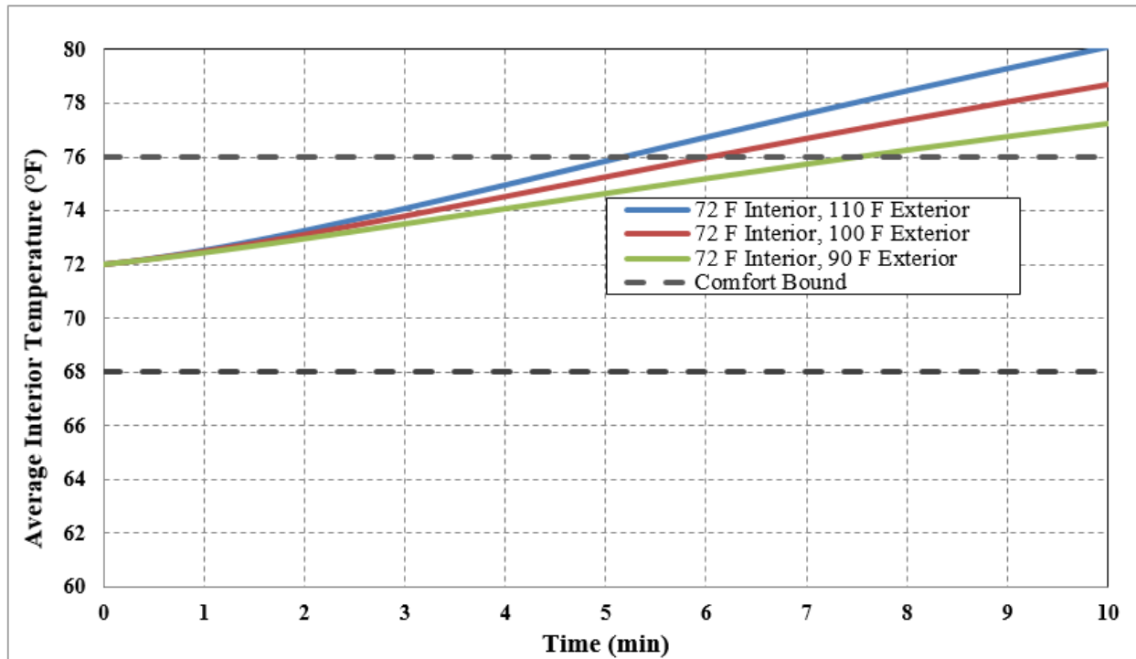
Figure 2.12. Time to increase interior temperature out of comfort zone in cooling season with 72 °F initial interior temperature
