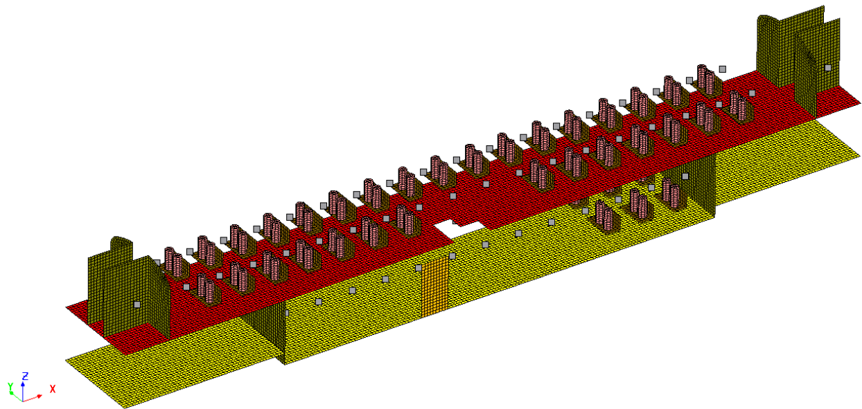
Figure 2.9. Representation of the interior air fluid nodes of the passenger car model in RadTherm
