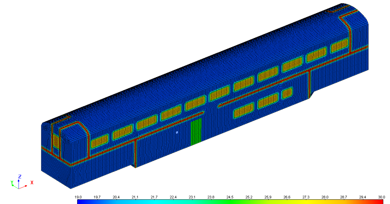
Figure 2.10. Temperature mapping of car exterior obtained after 10 minutes of HVAC deactivation simulation during winter at midnight (initial inside and outside temperature 72 °F and 20 °F, respectively)
