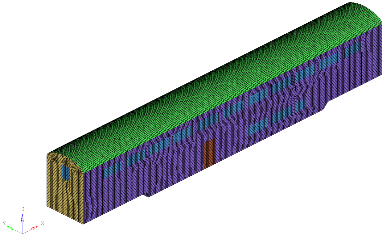
Figure 2.7. Isometric view of the bi-level passenger car
