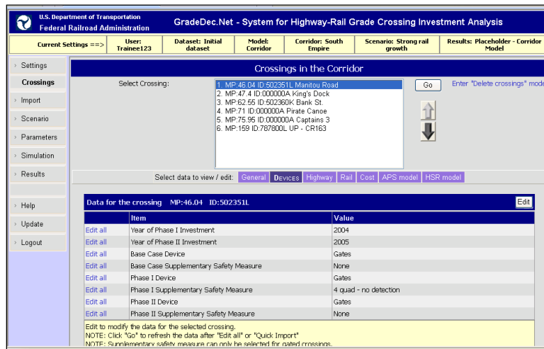
Figure 9 View of Crossings Page, with Corridor Model and Capital Programming, Devices Displayed
