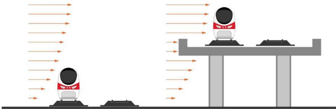
Figure 6-8. Trains exposed to stronger winds on viaducts due to greater distance from the ground
