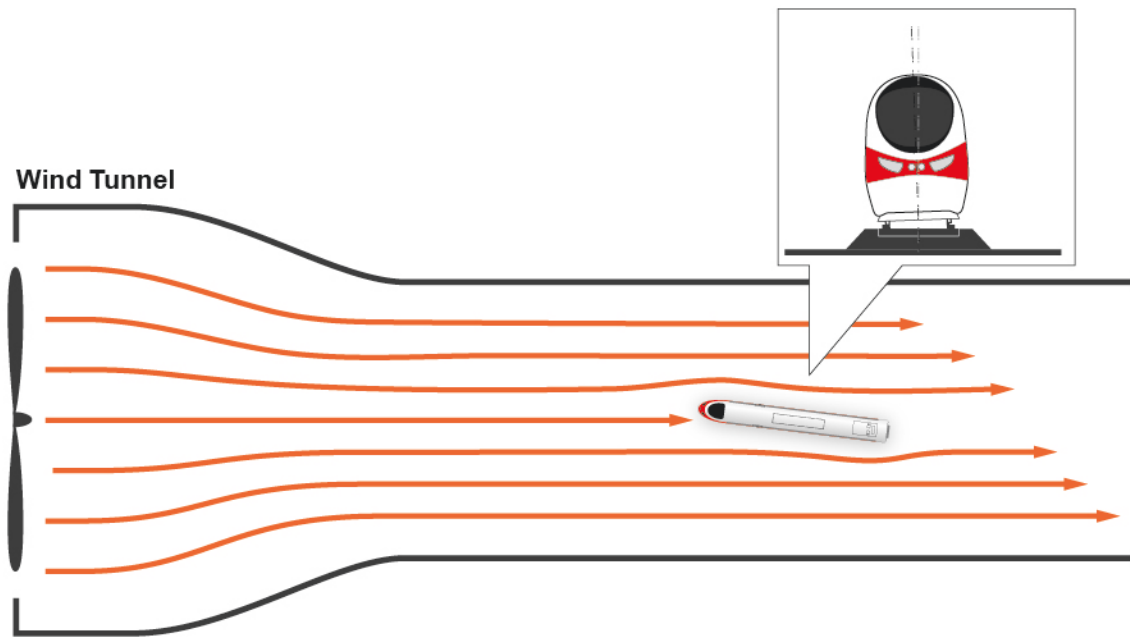
Figure 6-12. Wind tunnel test setup for measuring aerodynamic coefficients relevant to crosswind stability
