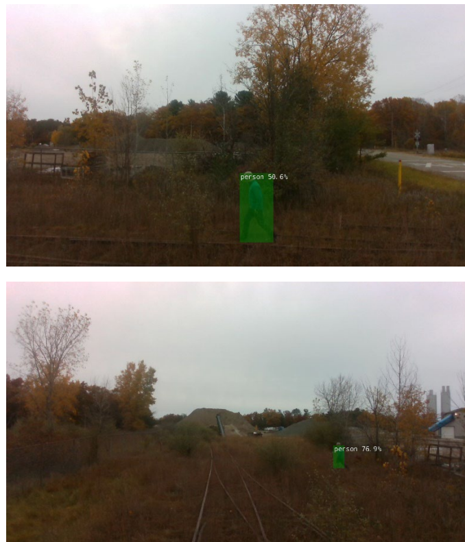
Figure 12. Representative outputs from UAV-based trespasser detection system
