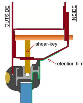
Down-Selected Glazing Retention System for Emergency Egress Windows
