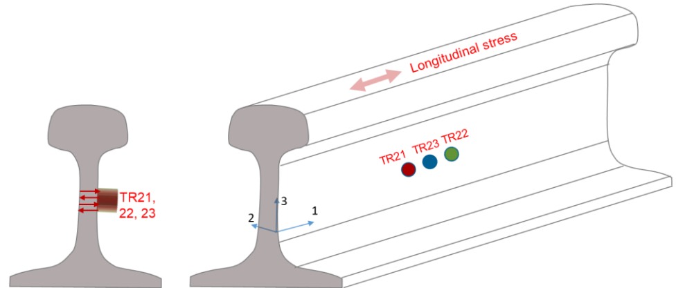
Measure three wave velocities through web thickness
