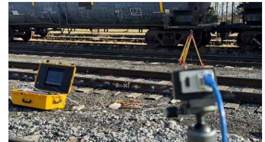
Beam on Elastic Foundation (BoEF) response from multi-point, digital image correlation (DIC) measurements
