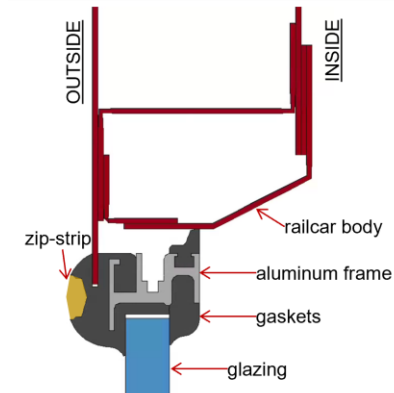
Existing Glazing Retention System
