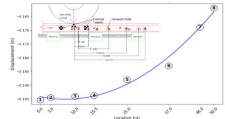
Beam on Elastic Foundation (BoEF) response from multi-point, digital image correlation (DIC) measurements
