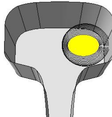
Detail Fracture Growth Simulation
