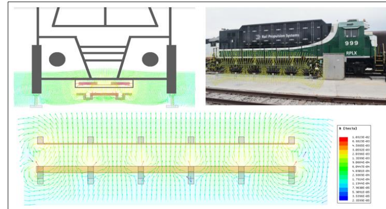
IWPT system magnetic flux distribution
