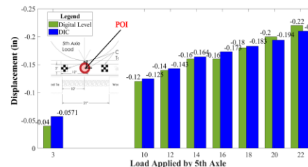
Vertical Deflection Measured by DIC and Digital Level
