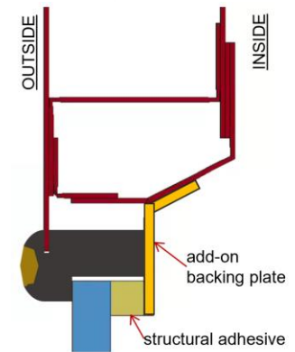
Down-Selected Glazing Retention System for Non-Emergency Windows
