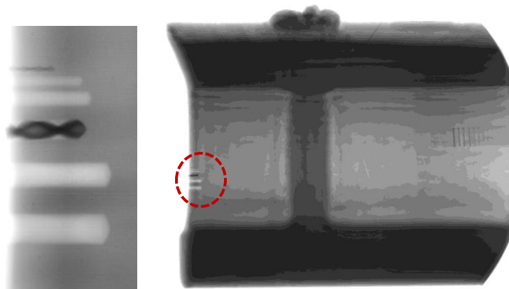
Processed radiograph a flash-butt with a zoomed-in view (left) highlighting the machined holes to represent flaws with diameters of 0.5 mm (tungsten impurity), 1 mm, 1.5 mm, 2 mm, 2.5 mm, and 3 mm (top to bottom)
