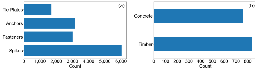
Figure 4. Example inventory of HTL Section 3 (a) number and type of hold-down devices (b) and number and type of crossies
