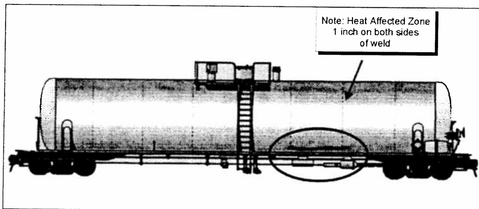
Figure 8. Rail Dent
