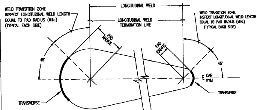
DOUBLE SIDED CIRCULAR PAD
