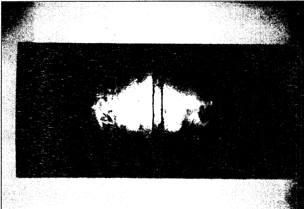
Figure 28. Master Gage Standard #1 Located in the Defect Library
