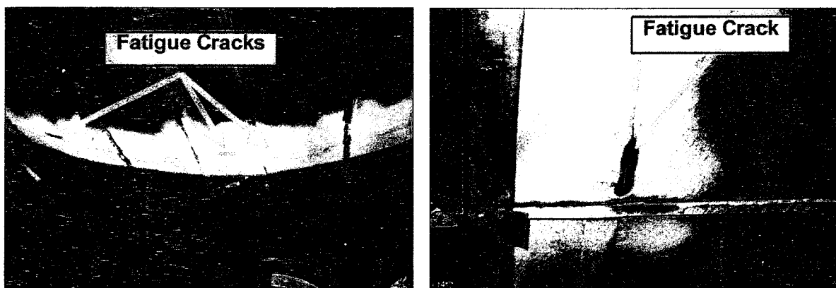
Figure 39. Fluorescent Liquid Penetrant Crack Indications on Tank Car Test Panels
