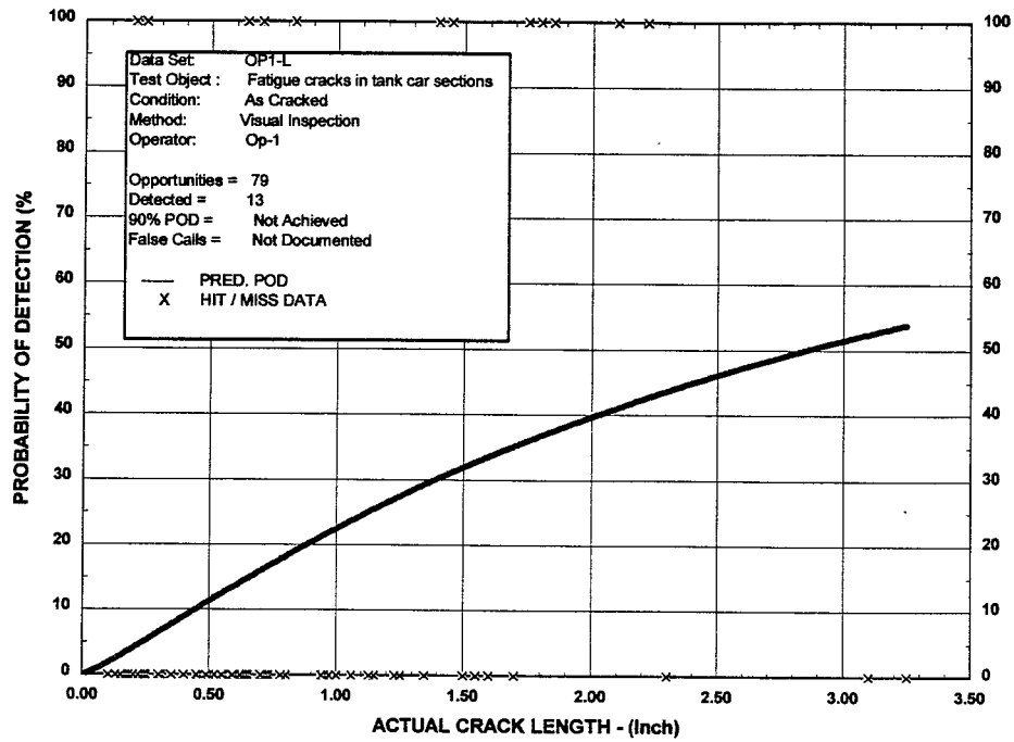
Figure 58. Optically Aided Visual POD Curve for Operator Number 1
