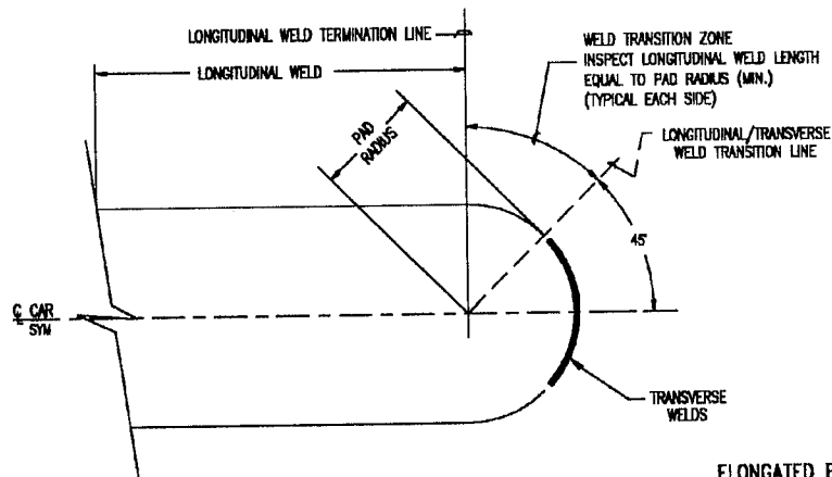
ELONGATED PAD
