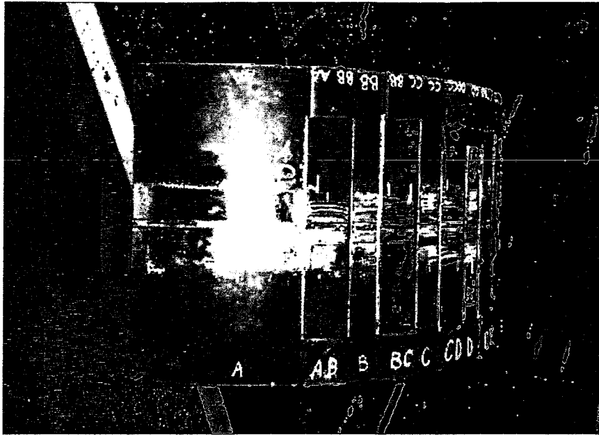
Figure 15. Fatigue Crack Test Panel during Preparation for Fatigue Initiation
