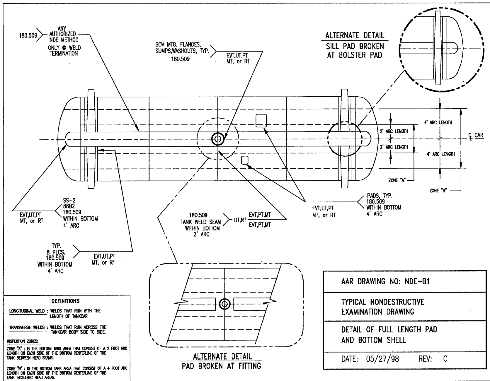
Figure 9. AAR Drawing No. NDE-B1 Detailing the Full Length Pad and Bottom Shell
