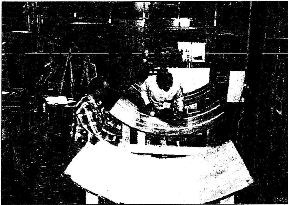
Figure 27. Transverse Butt Weld Test Panels Included in the Defect Library
