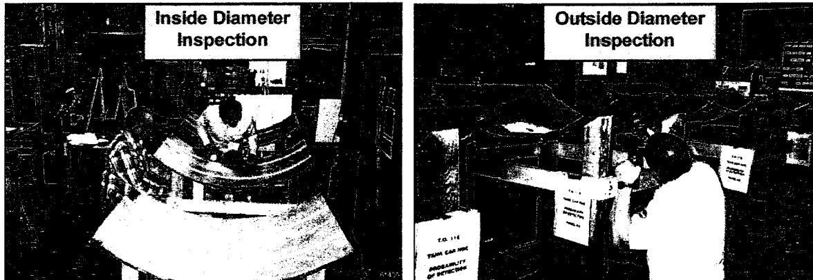
Figure 57. Optically Aided Visual Inspection on the Inside and Outside Diameters of the Tank Car Test Panels
