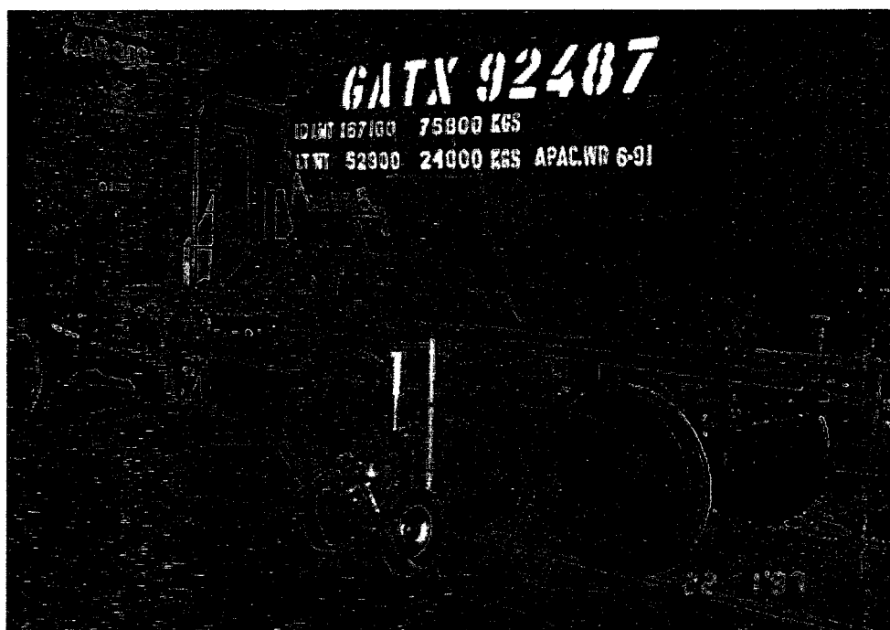
Figure 30. AE Jacking Test Setup on Baseline Tank Car
