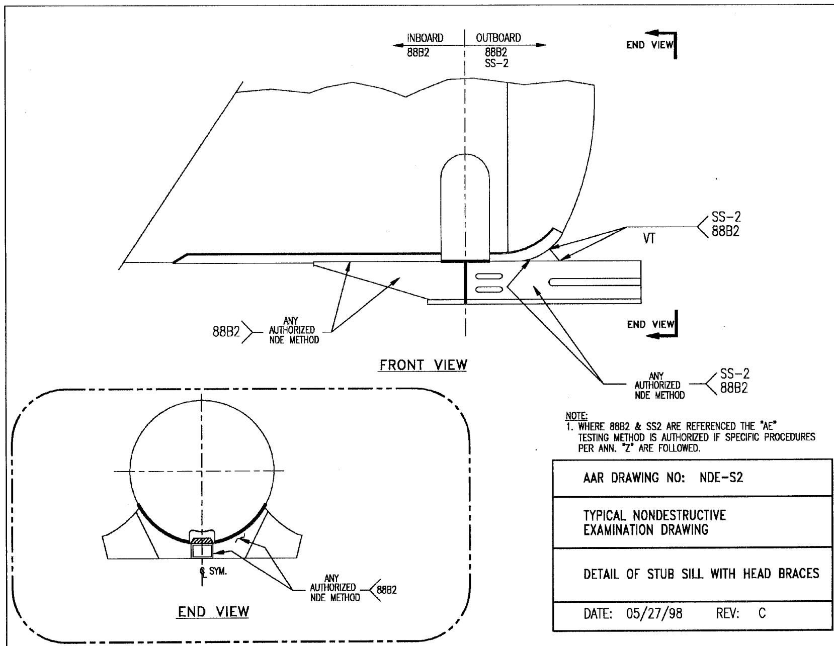
Figure 7. AAR Drawing No. NDE-S2 Detailing the Stub Sill with Head Braces
