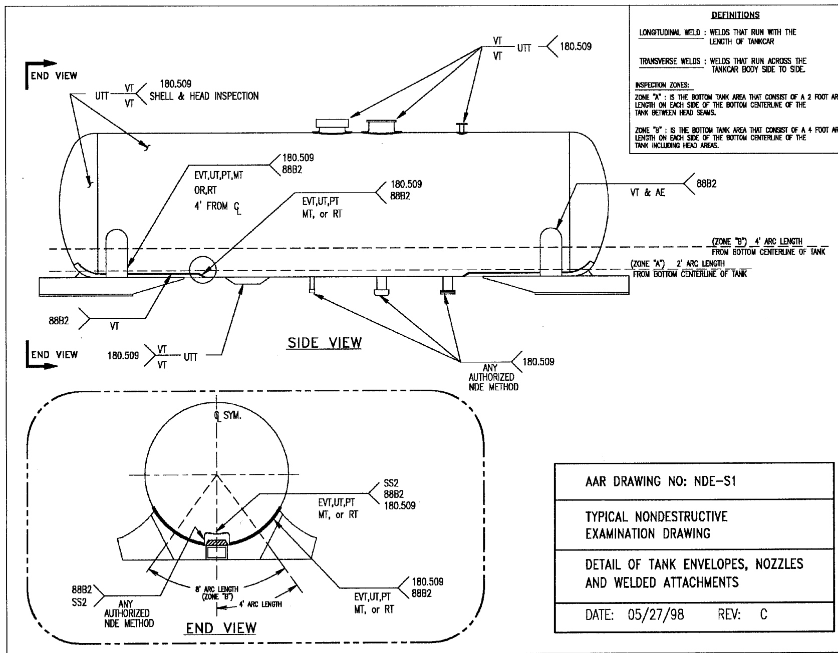
Figure 6. AAR Drawing No. NDE-S1 Detailing Tank Envelopes, Nozzles and Welded Attachments
