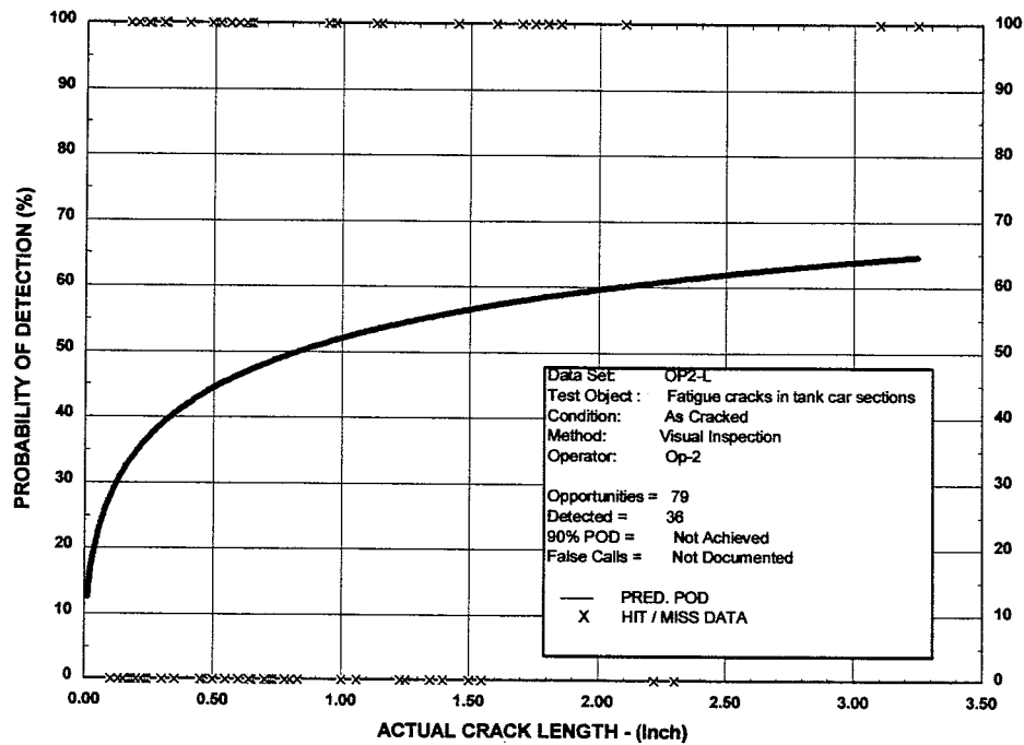
Figure 59. Optically aided Visual POD Curve for Operator Number 2
