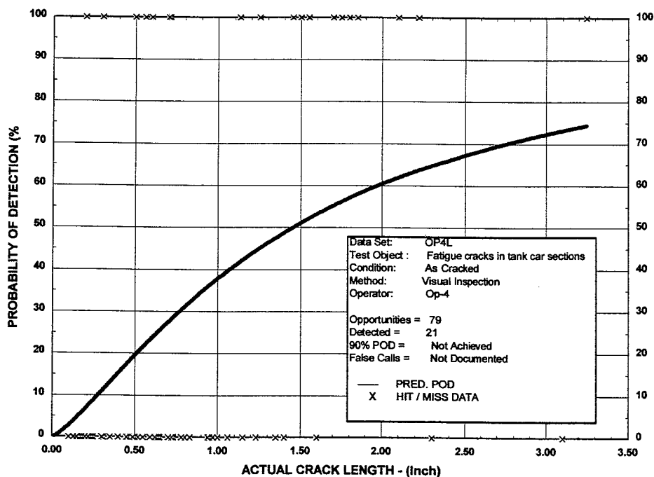
Figure 61. Optically Aided Visual POD Curve for Operator Number 4
