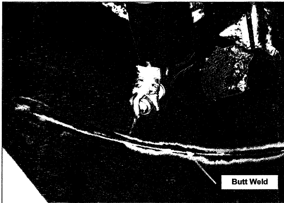
Figure 33. Liquid Penetrant Inspection of Transverse Butt Weld from the Interior of the Tank Car
