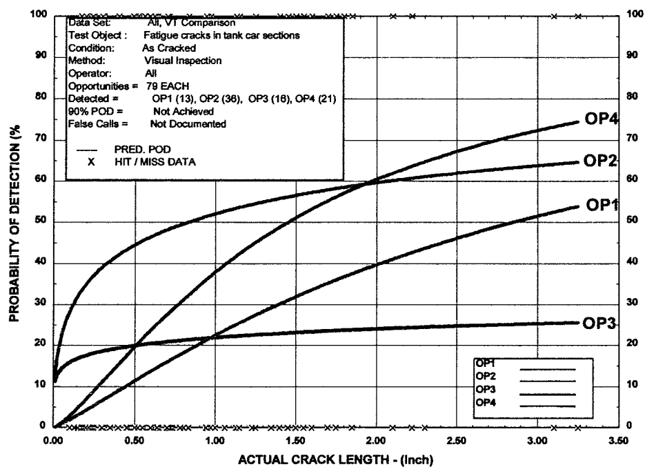
Figure 62. Optically Aided Visual POD Curve Comparison for all Operators
