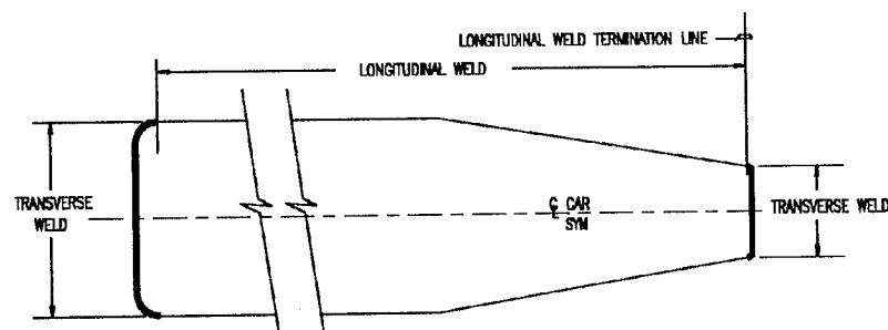
SQUARE END TAPERED PAD
