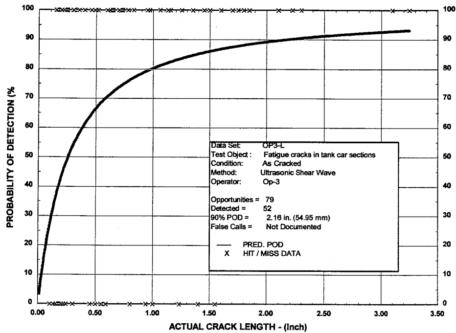
Figure 54. Shear Wave Ultrasonics POD Curve for Operator Number 3
