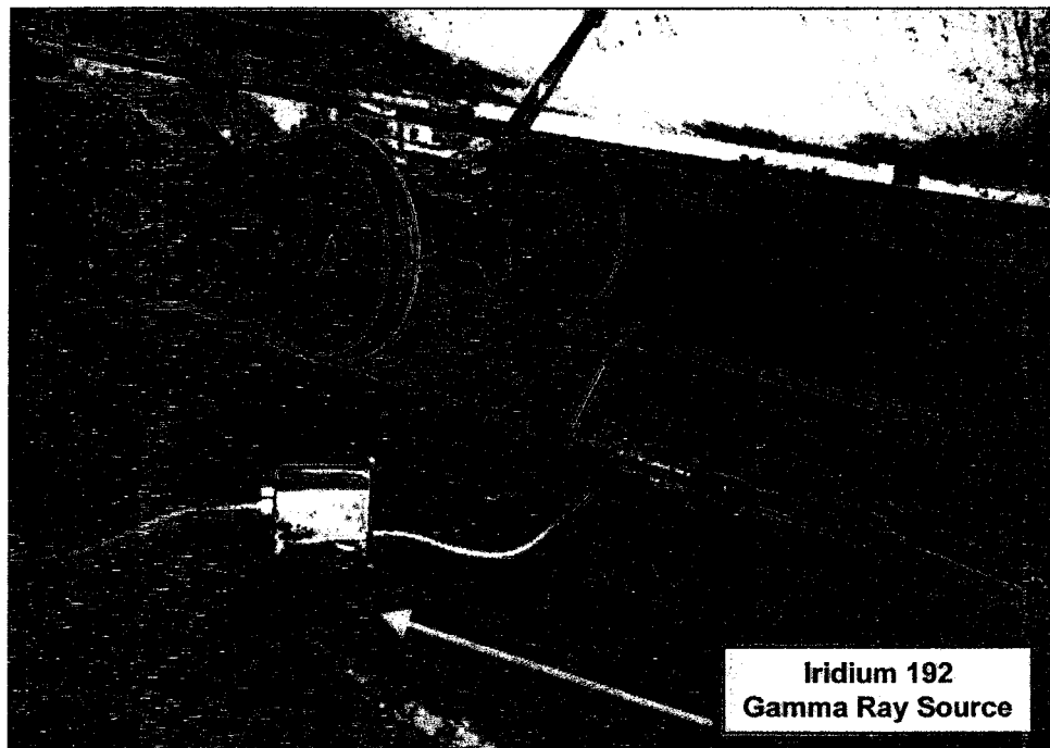
Figure 37. Gamma Ray Source Location for Transverse Butt Weld Inspection with Source at the Exterior of the Tank
