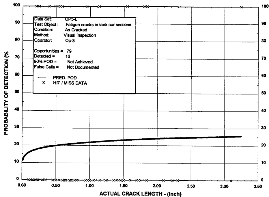
Figure 60. Optically Aided Visual POD Curve for Operator Number 3
