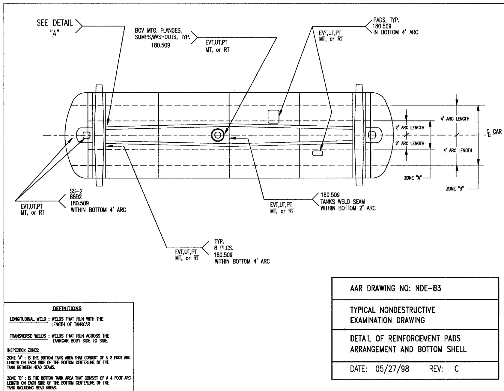
Figure 11. AAR Drawing No. NDE-B3 Detailing the Reinforcement Pad Arrangement and Bottom Shell
