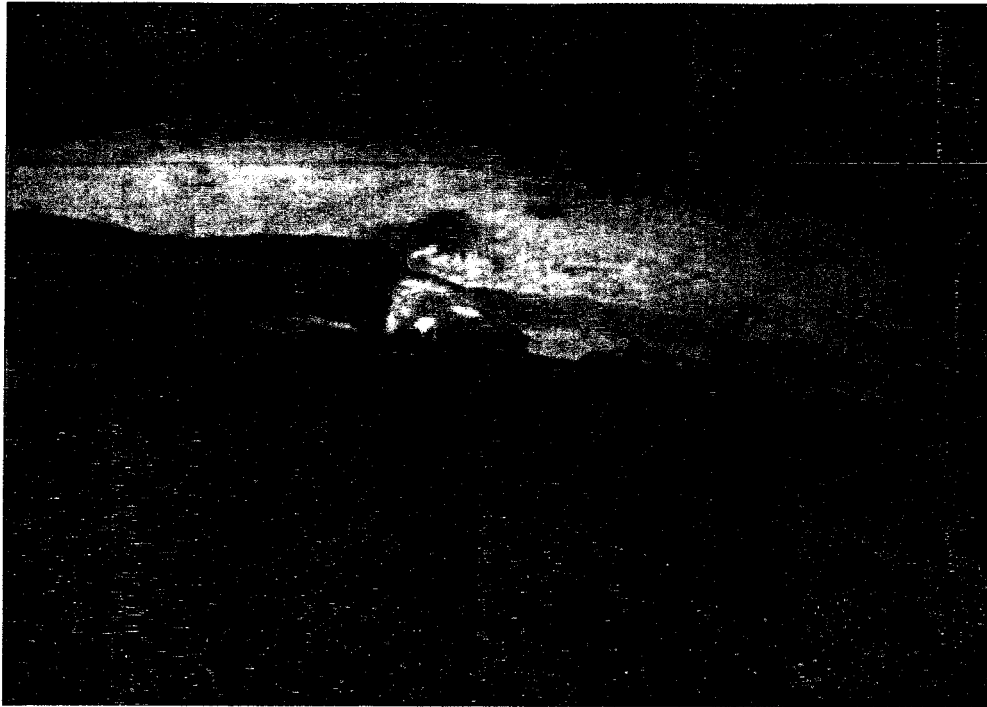
Figure 34. Liquid Penetrant Inspection Showing 0.050-inch Crack at Fillet Weld Termination of the Sill Bearing Plate
