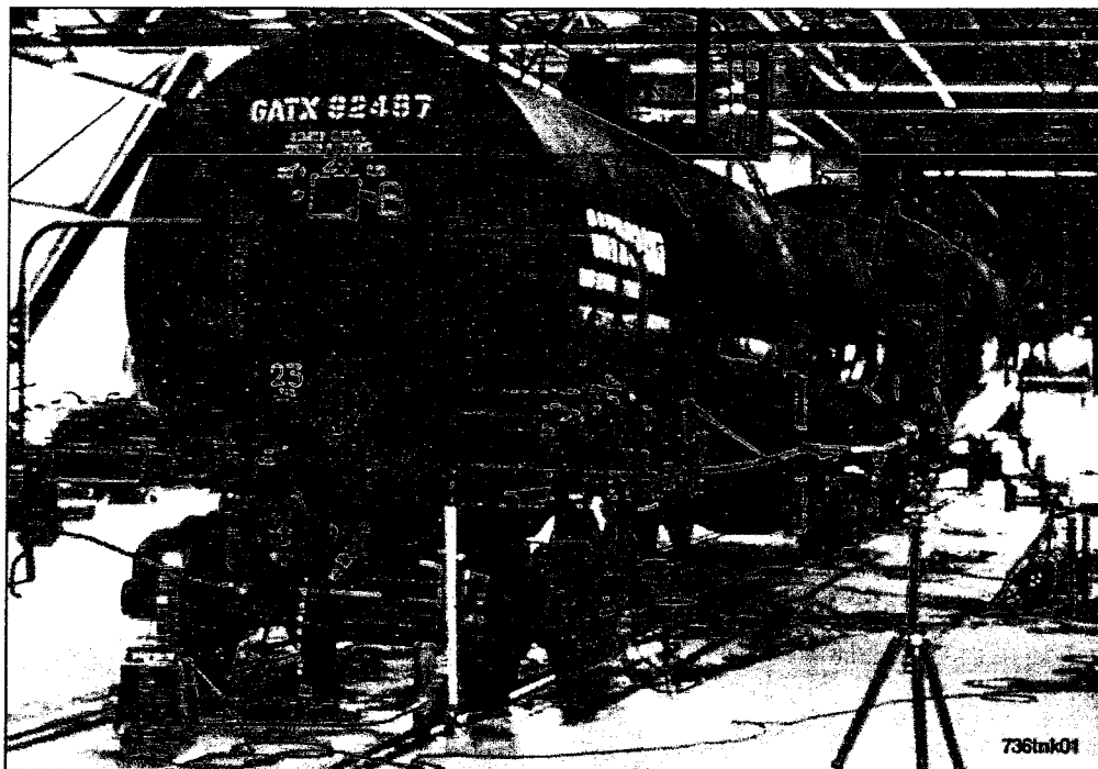
Figure 1. General Service Jacketed Tank Car Used in Baseline Evaluations
