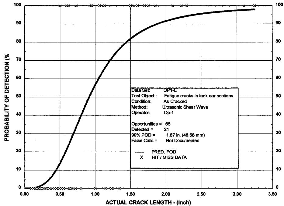
Figure 52. Shear Wave Ultrasonics POD Curve for Operator Number 1
