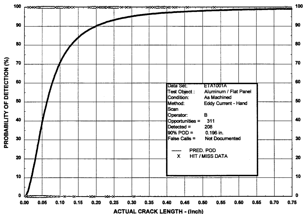
Figure 14. Typical Probability of Detection (POD) Curve
