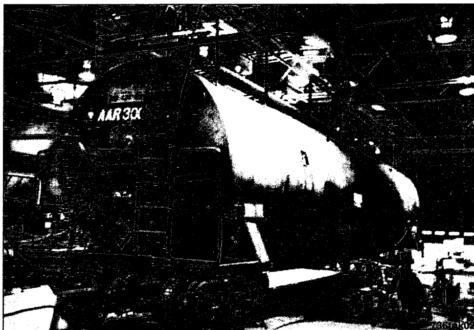
Figure 29. AE Pressure Test Setup on Baseline Tank Car
