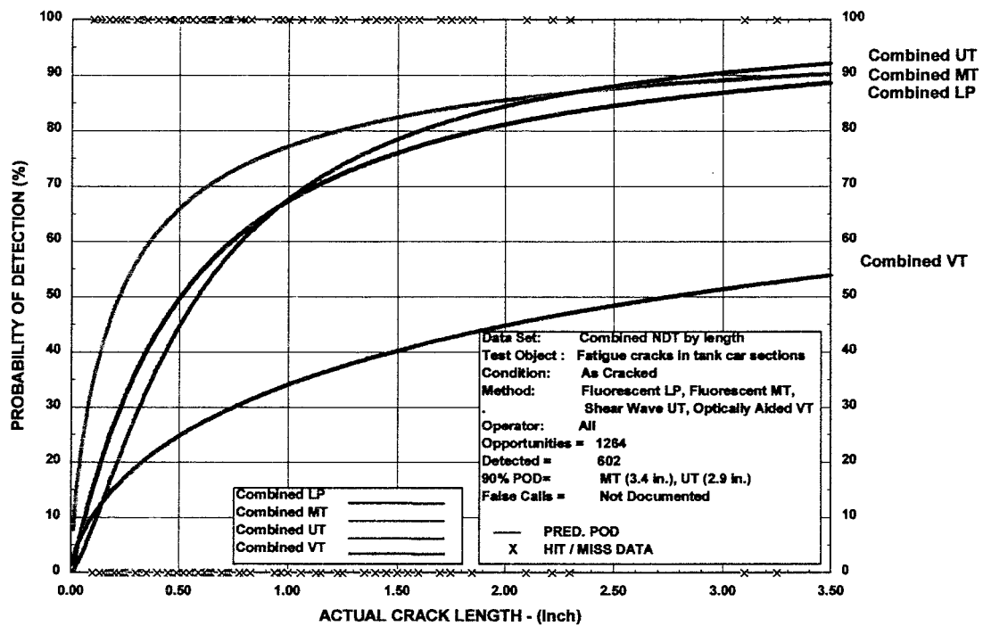
Figure 67. POD Curve Comparison for All Methods for All Operators Combined
