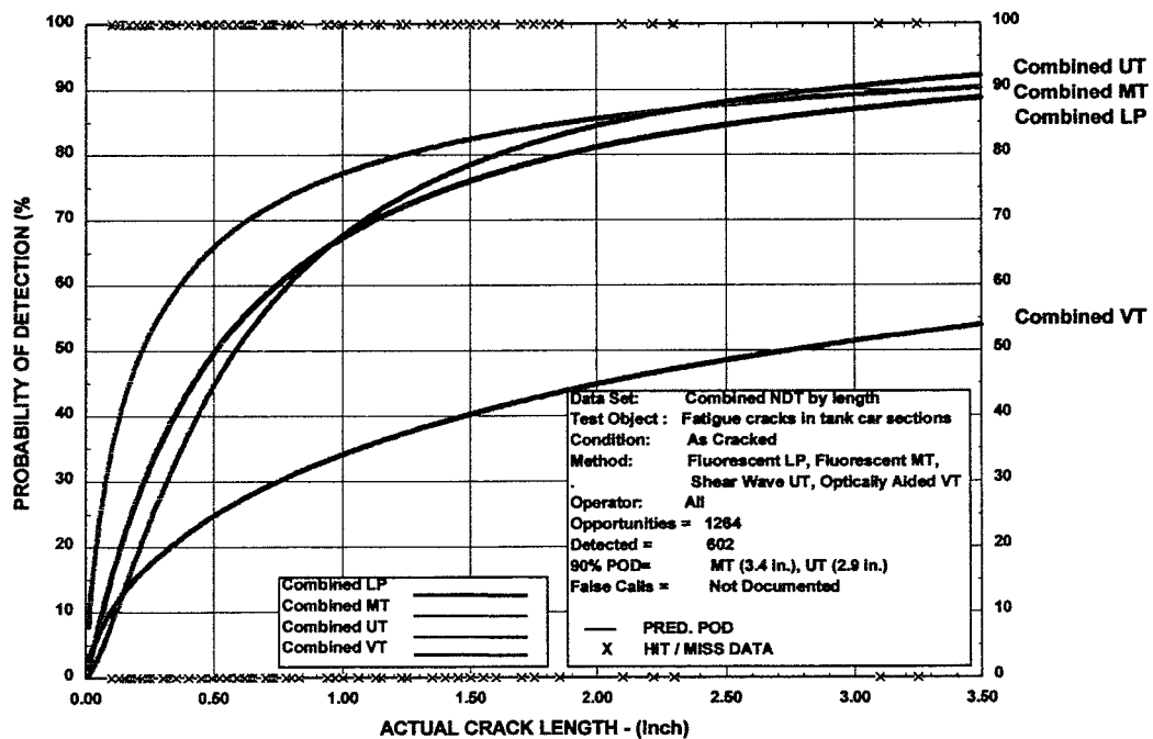
Figure 69. POD Curve Comparison of All Methods for All Operators Combined, Showing Variability Between NDE Test Methods
