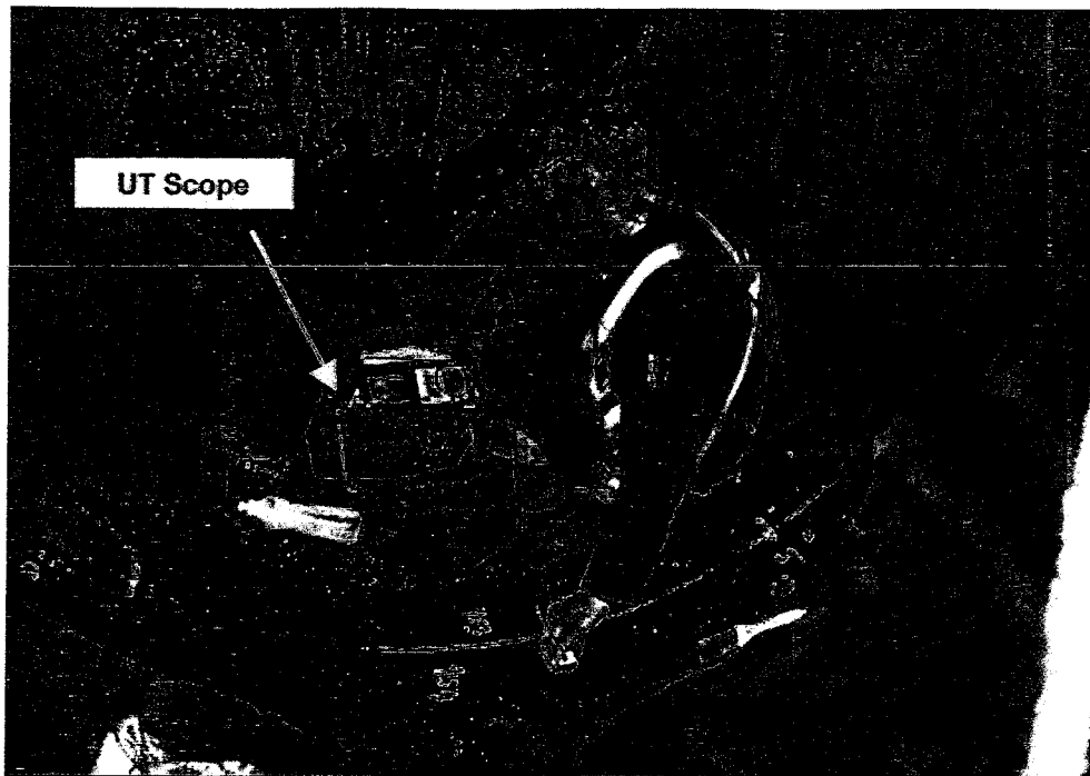
Figure 38. Ultrasonic Evaluation of the Transverse Butt Weld from the Interior of the Tank
