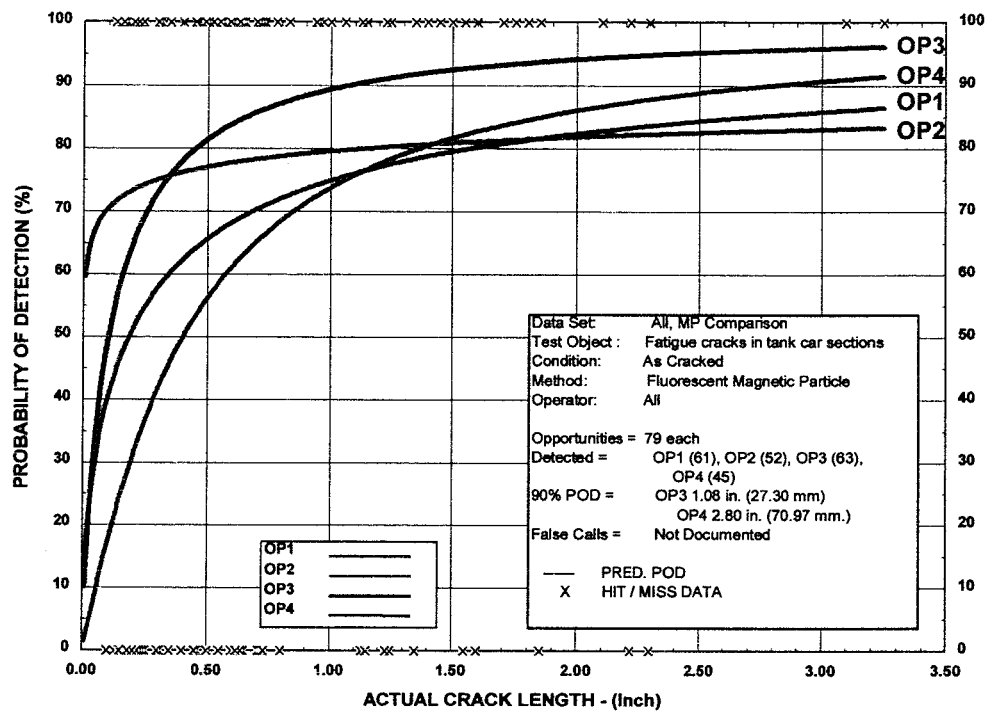
Figure 50. Fluorescent Magnetic Particle POD Curve Comparison for All Operators
