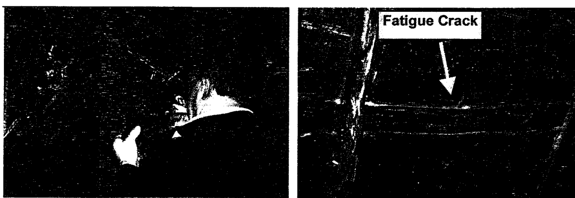
Figure 45. Fluorescent Magnetic Particle Longitudinal and Transverse Crack Indications on Tank Car Test Panels
