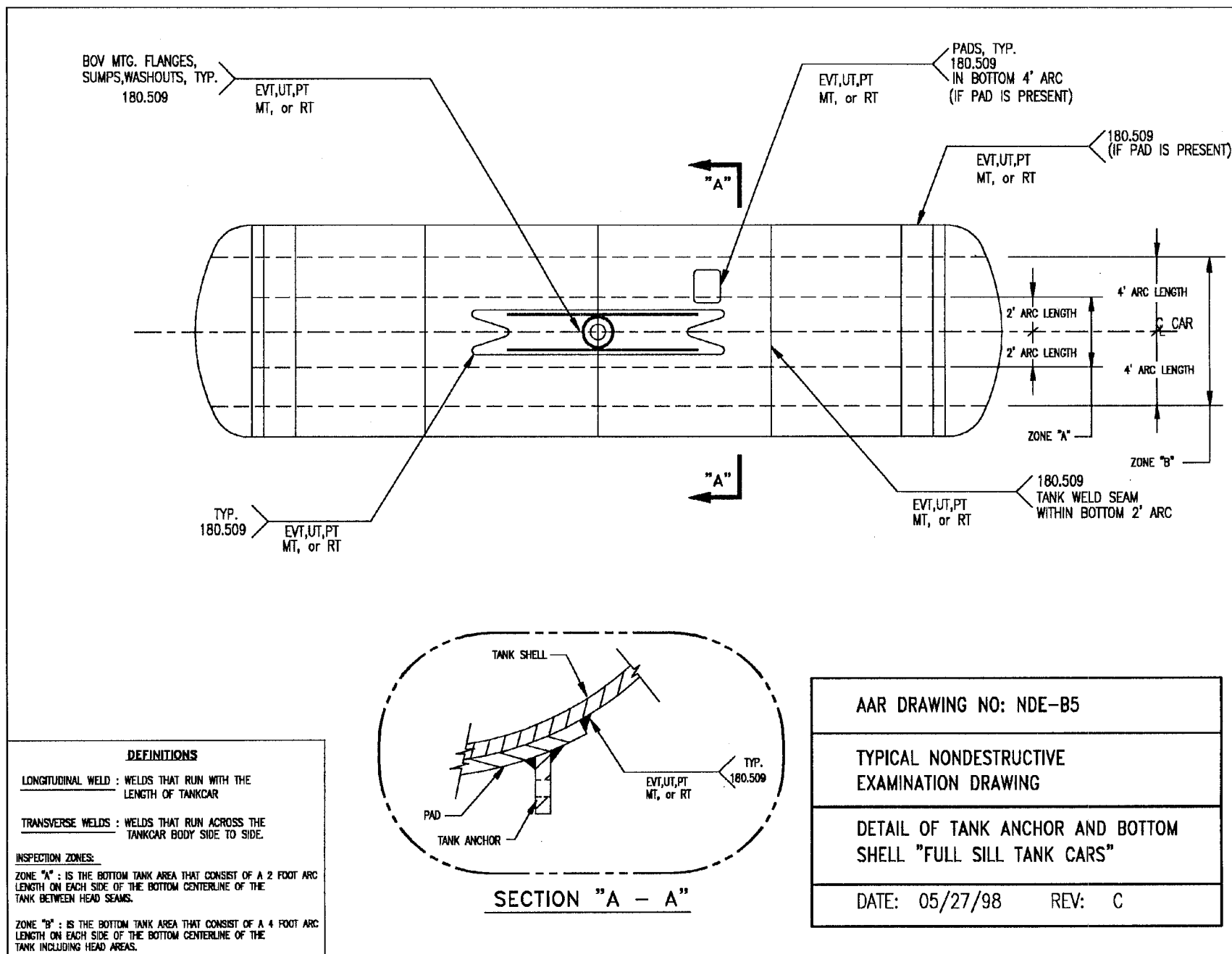
Figure 13. AAR Drawing No. NDE-B5 Detailing the Tank Car Anchor and Bottom Shell "Full Sill Tank Cars"
