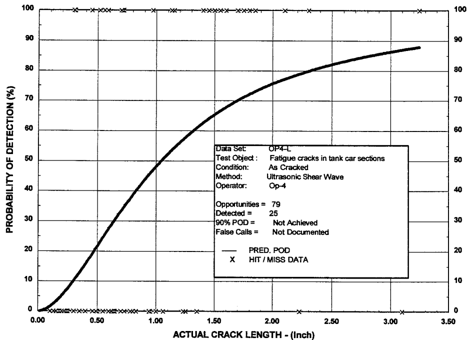
Figure 55. Shear Wave Ultrasonics POD Curve for Operator Number 4
