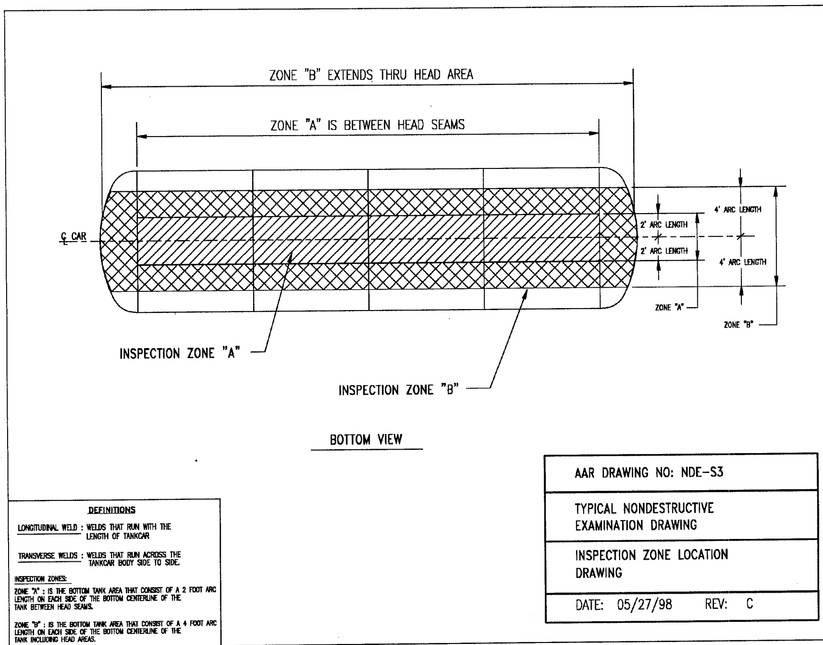
Figure 8. AAR Drawing No. NDE-S3 Identifying the Inspection Zone Locations
