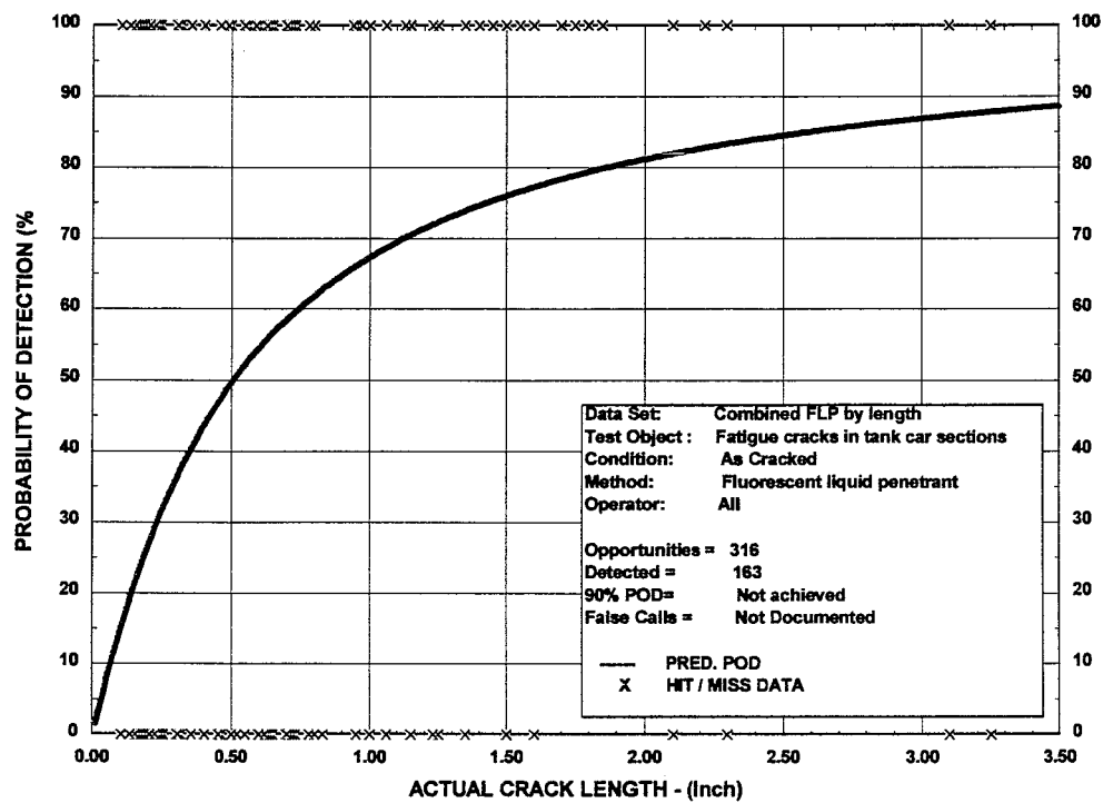
Figure 63. Fluorescent Liquid Penetrant POD Curve for All Operators Combined
