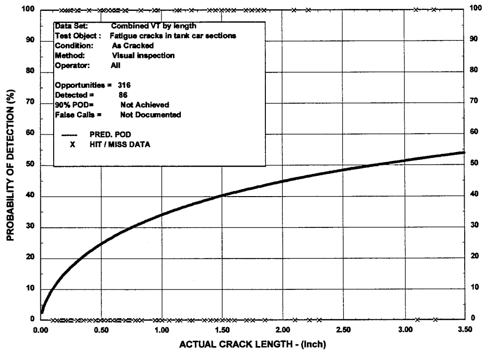
Figure 66. Optically Aided Visual POD Curve for All Operators Combined
