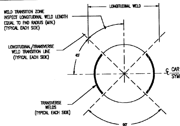
DOUBLE SIDED CIRCULAR PAD
