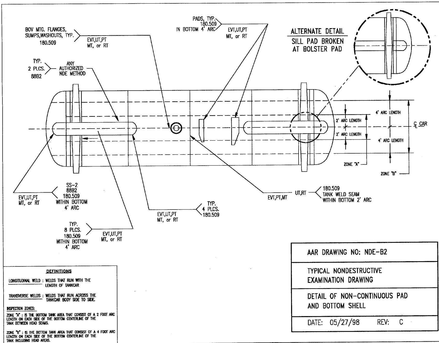
Figure 10. AAR Drawing No. NDE-B2 Detailing a Non-continuous Pad and Bottom Shell
