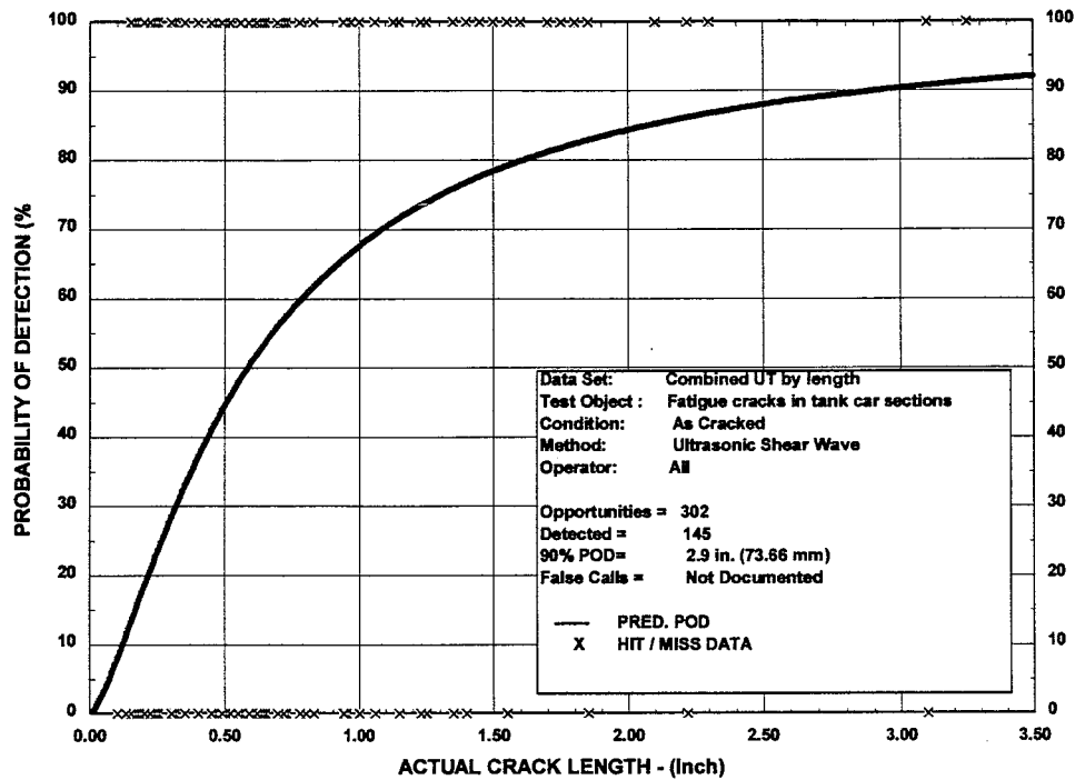
Figure 65. Shear Wave Ultrasonics POD Curve for All Operators Combined
