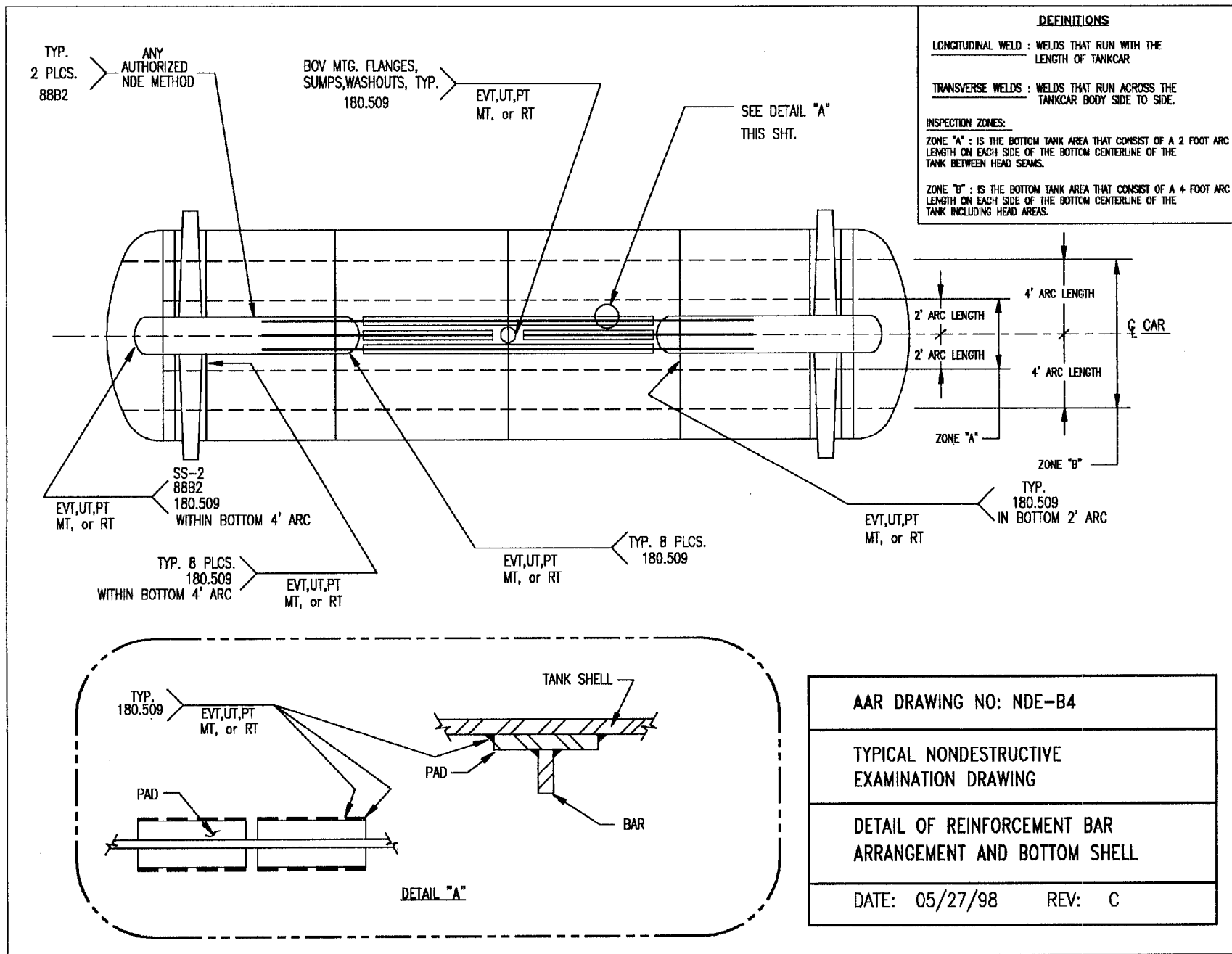
Figure 12. AAR Drawing No. NDE-B4 Detailing the Reinforcement Bar Arrangement and Bottom Shell
