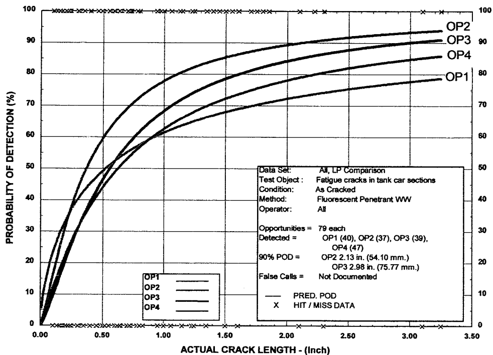
Figure 44. Fluorescent Liquid Penetrant POD Curve Comparison of All Operators
