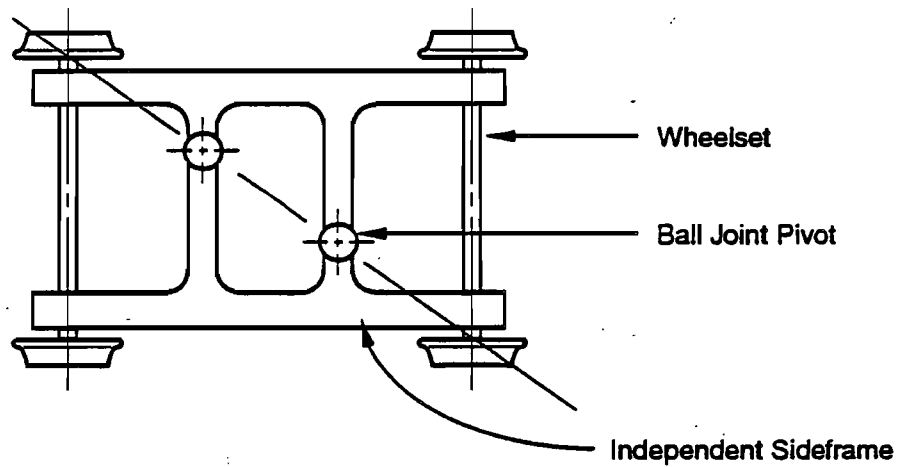
Figure 2.9b Pivots in Transoms (Rockwell)
