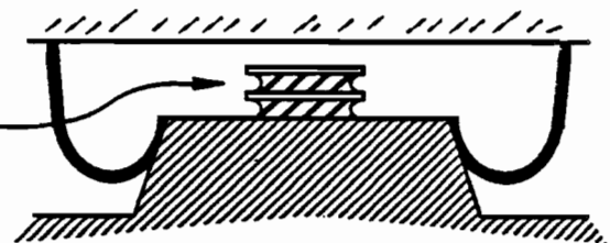
Figure 2.14c Rolling Diaphragm Air Spring
