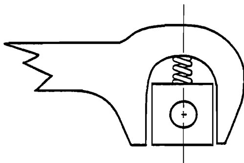
Figure 2.11a Coil Spring/Pedestal
