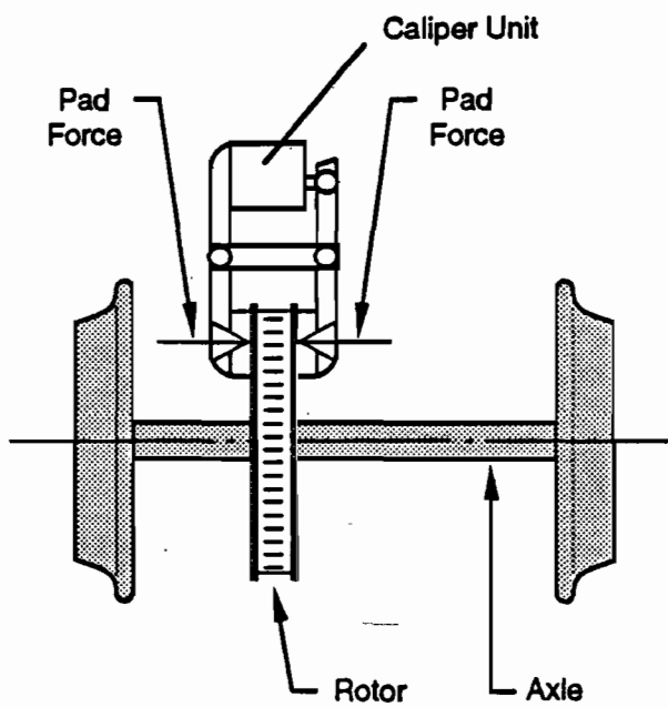
Figure 2.5c Disk Brake
