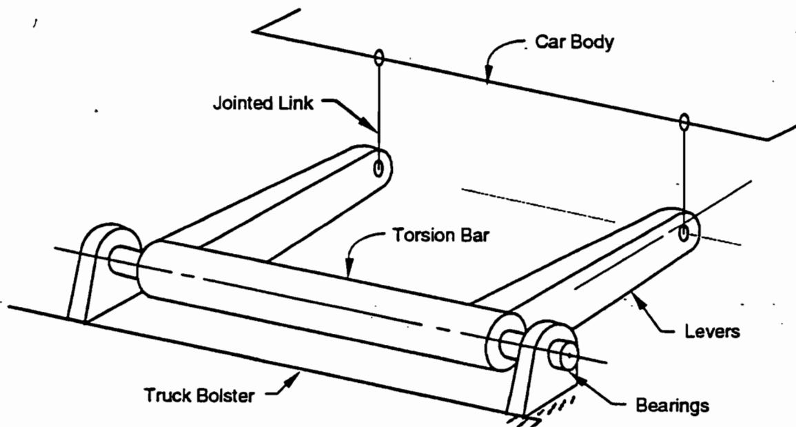
Figure 2.14d Anti-Roll Bar
