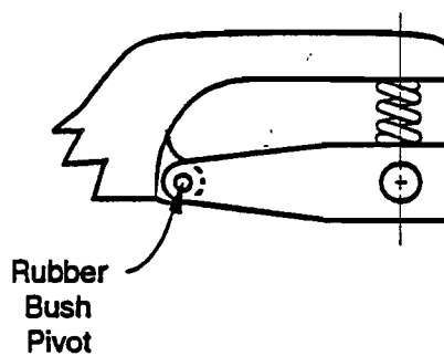
Figure 2.11d Radius Arm
