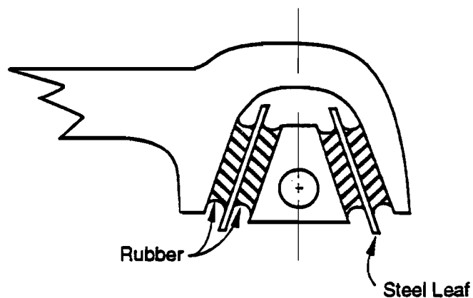
Figure 2.11b Rubber Chevron
