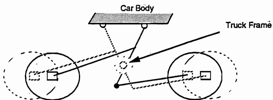
Figure 2.19b Forced Steering on a Two-Axle Truck
