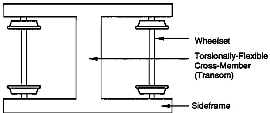
Figure 2.9c Torsionally-Flexible Frame
