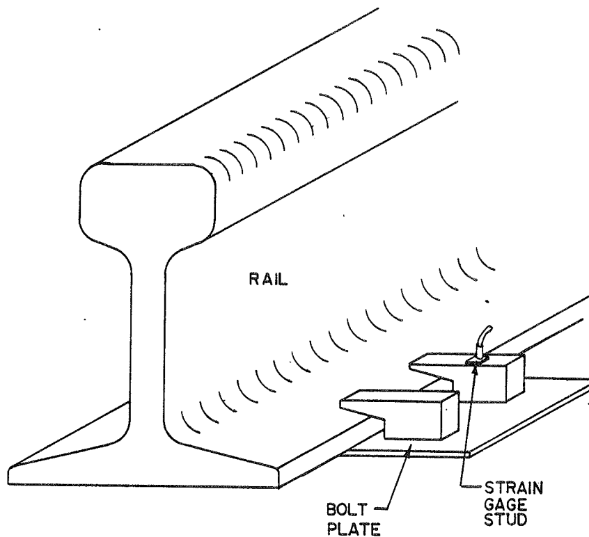
Figure 6 Strain Gage Stud Presence Detector
