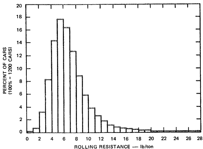
FIGURE 3 ROLLING RESISTANCE HISTOGRAM — 1-lb/ton INTERVALS
