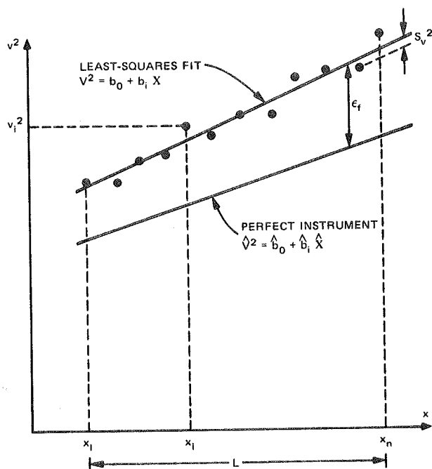
FIGURE A-1 INSTRUMENT ERRORS
