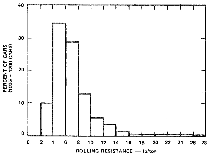
FIGURE 2 ROLLING RESISTANCE HISTOGRAM — 2-lb/ton INTERVALS
