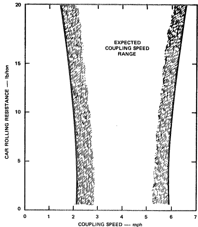
FIGURE 1 EXPECTED RANGE OF COUPLING SPEED WHEN UNCERTAINTIES IN ROLLING RESISTANCE, DISTANCE TO COUPLE, AND TANGENT POINT SPEED ARE \pm 0.5 lb/ton, \pm 50 ft, AND \pm 0.1 mph, RESPECTIVELY
