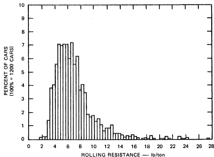
FIGURE 4 ROLLING RESISTANCE HISTOGRAM — 0.4-lb/ton INTERVALS
