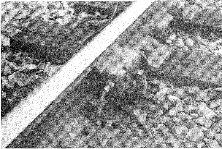
a) Permanent Magnet Wheel Detector
