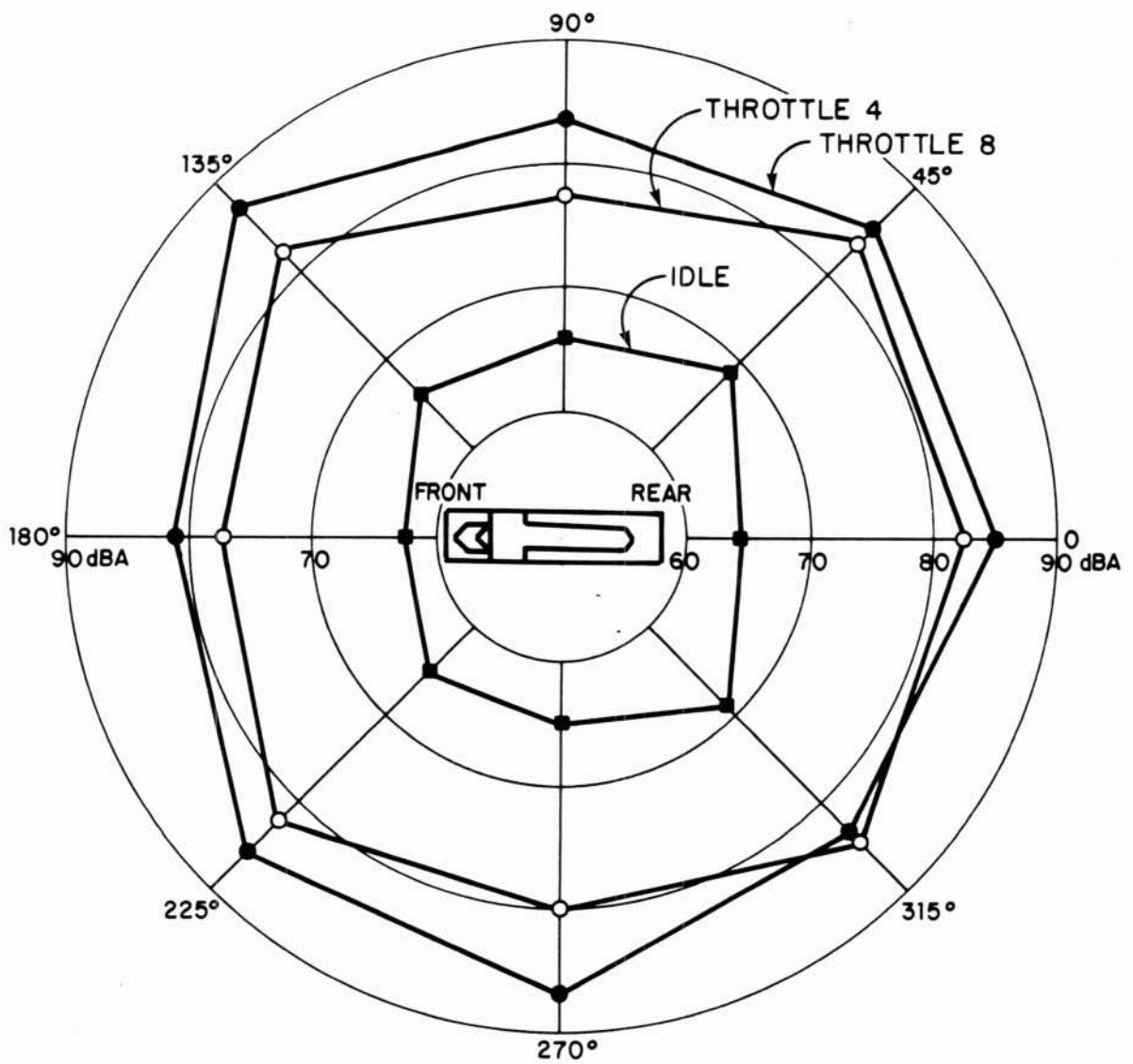
FIG. 4.6. DIRECTIVITY OF LOCOMOTIVE NOISE.
