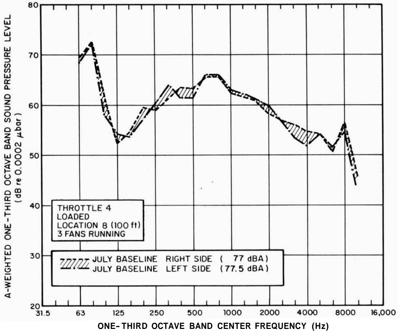
FIG. A.23. LOCOMOTIVE BASELINE NOISE, THROTTLE 4, FULL LOAD, MICROPHONE LOCATION 8.
