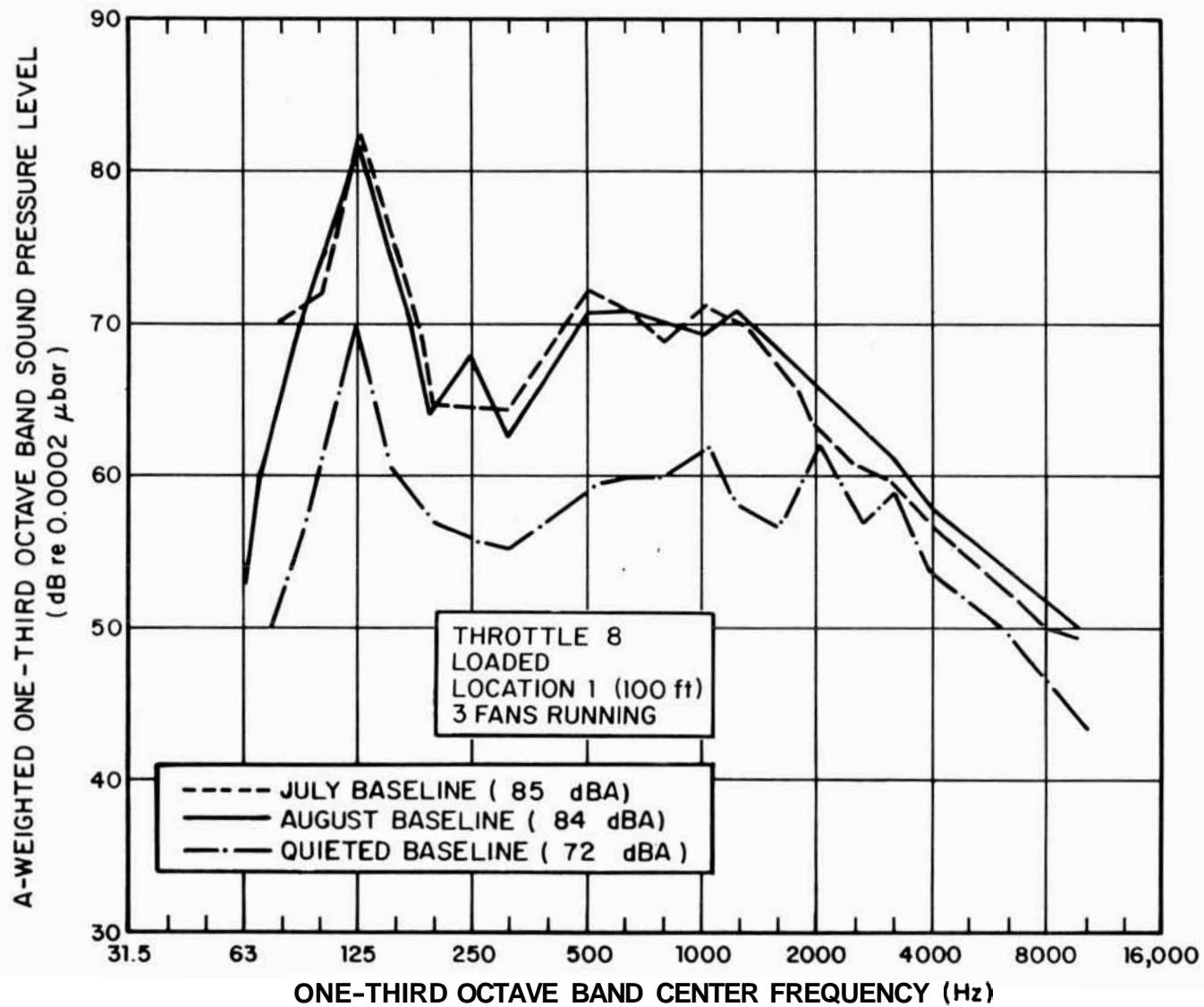
FIG. A.3. LOCOMOTIVE BASELINE NOISE, THROTTLE 8, FULL LOAD, MICROPHONE LOCATION 1.
