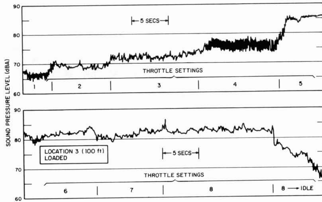
FIG. 4.11. NOISE FROM INDIVIDUAL THROTTLE SETTINGS, LOCATION 3, LOADED.
