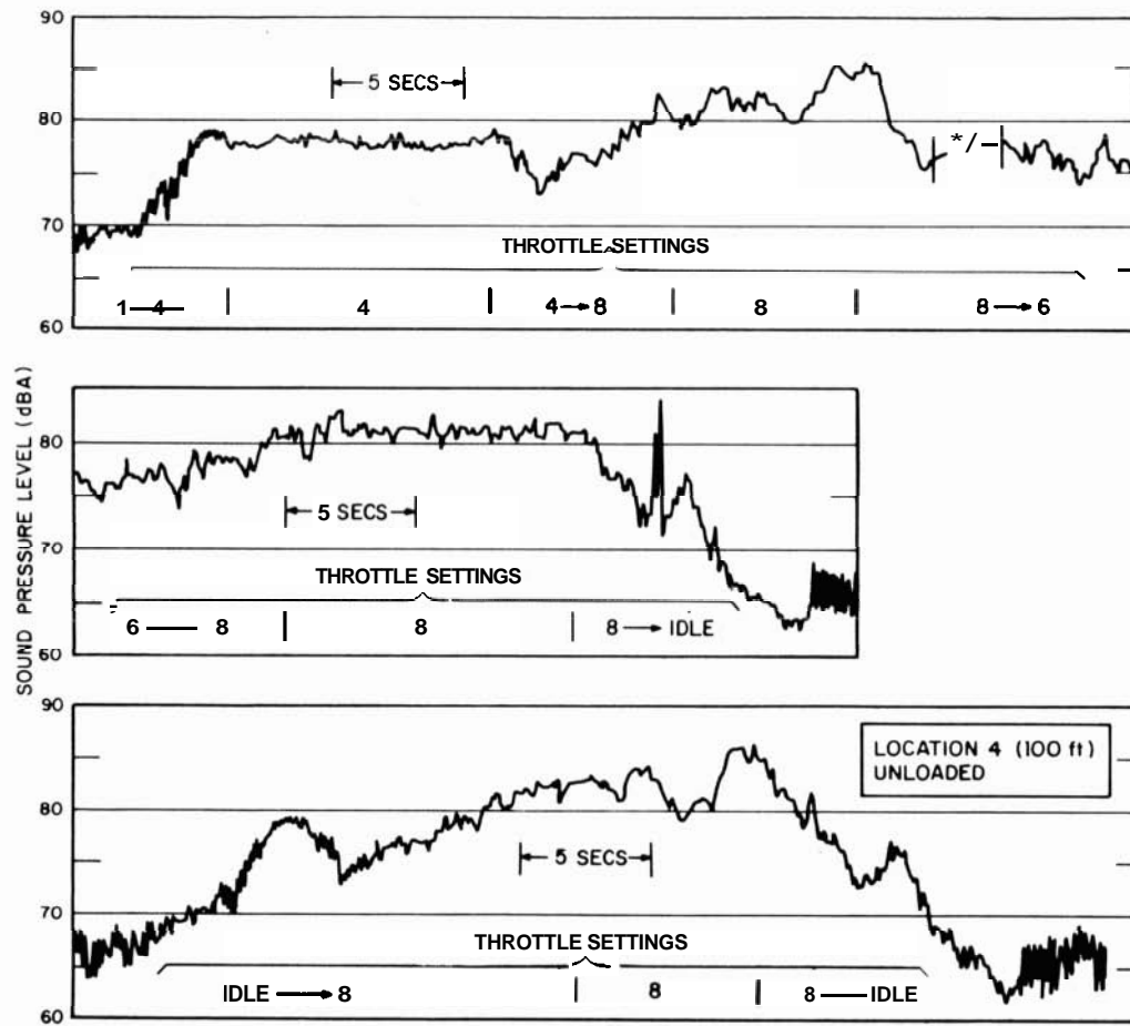
FIG. 4.10. NOISE DURING "THROTTLE WIPE" TESTS, LOCATION 4, UNLOADED.
