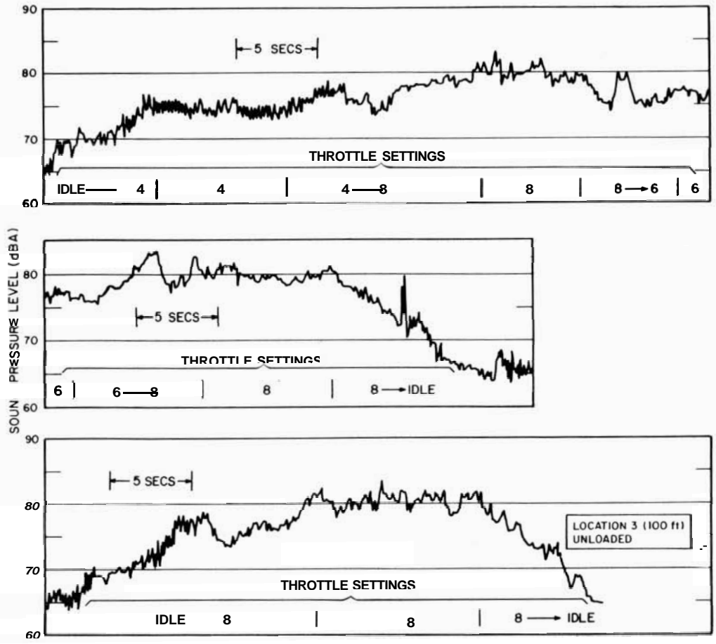
FIG. 4.14. NOISE DURING "THROTTLE WIPE" TESTS, LOCATION 3, UNLOADED
