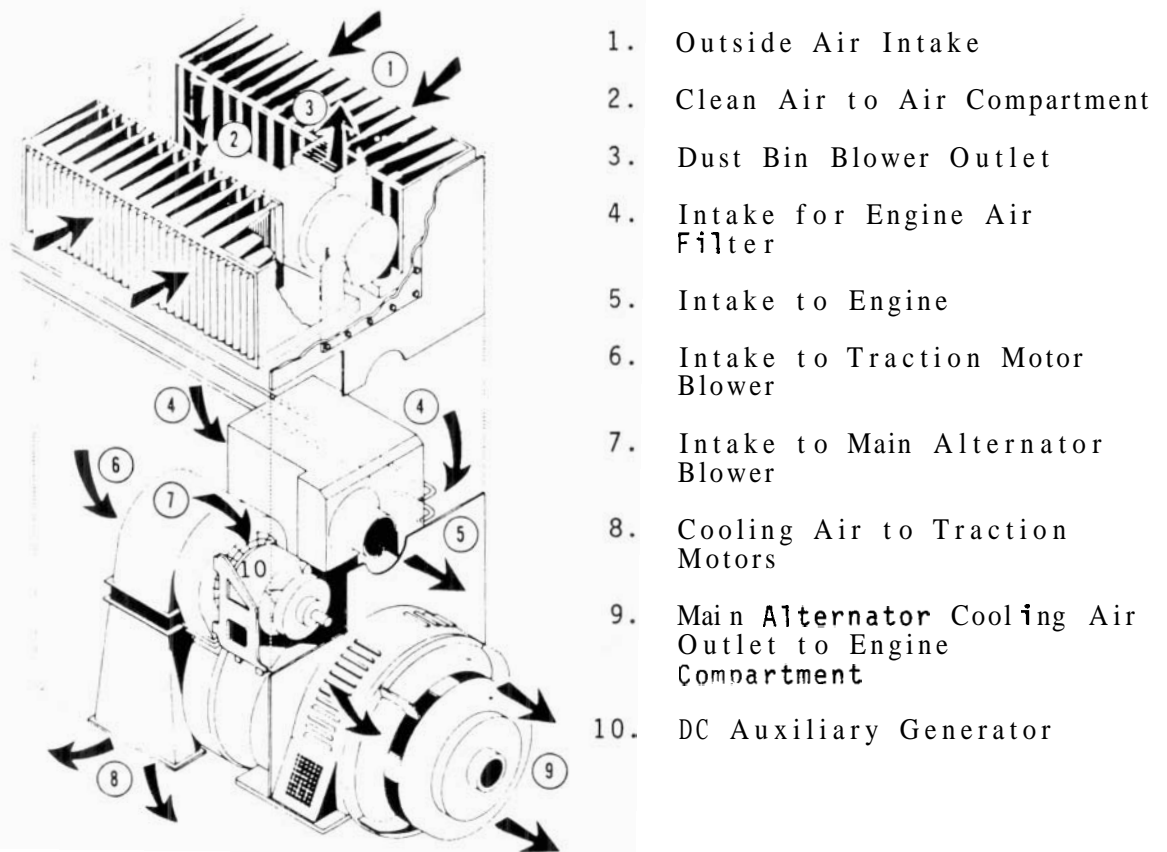
FIG. 2.3. DETAILS OF THE AIR COMPARTMENT.
