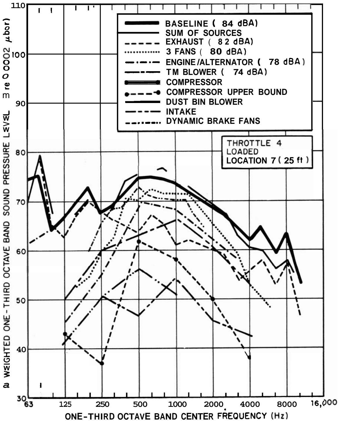
FIG. 8.19. SOURCE SPECTRA, THROTTLE 4, FULL LOAD, MICROPHONE LOCATION 7.
