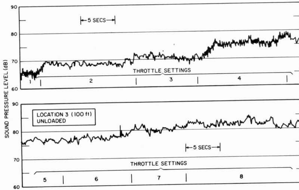
FIG. 4.13. NOISE FROM INDIVIDUAL THROTTLE SETTINGS, LOCATION 3, UNLOADED.
