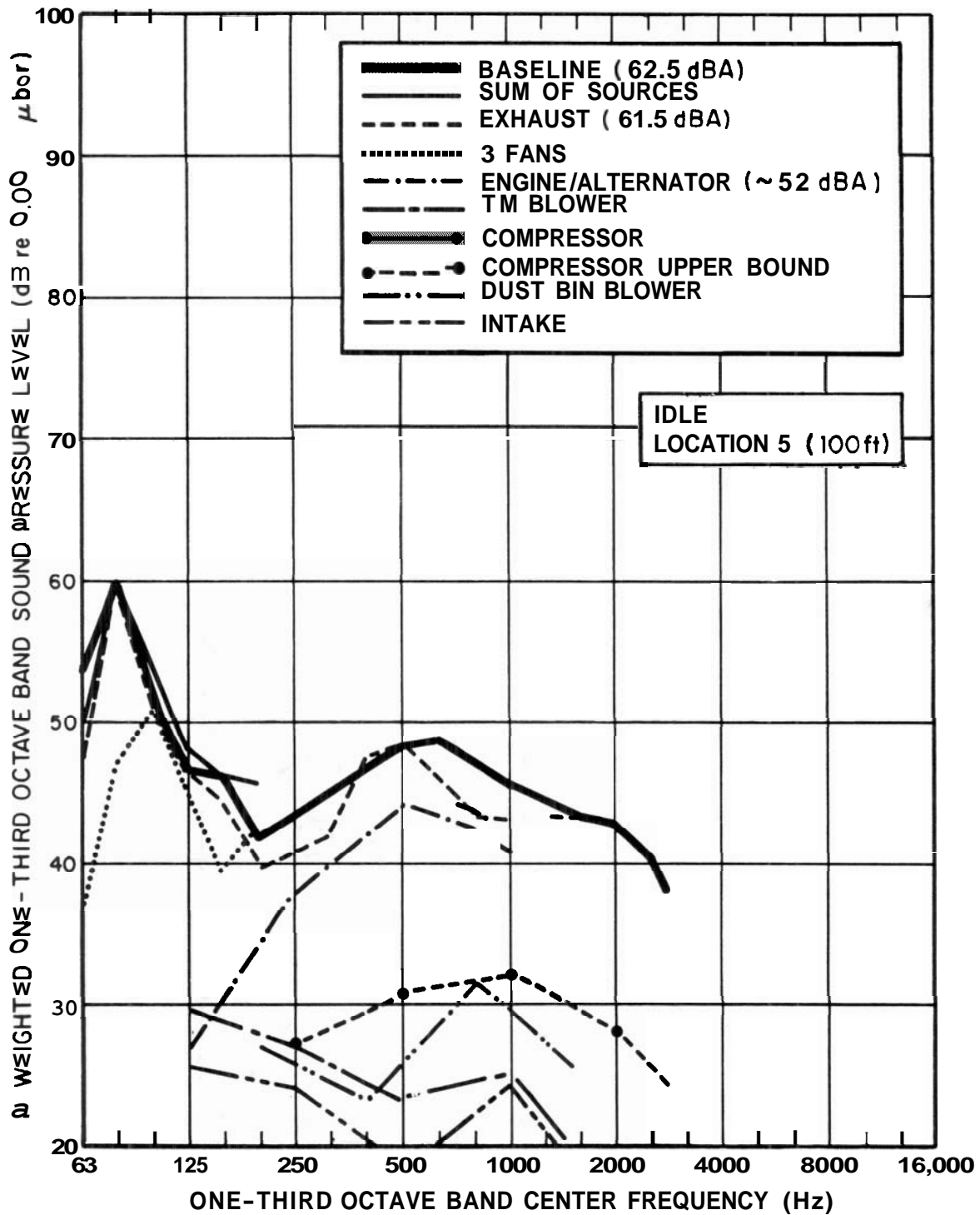
FIG. B.12. SOURCE SPECTRA, IDLE, MICROPHONE LOCATION 5.
