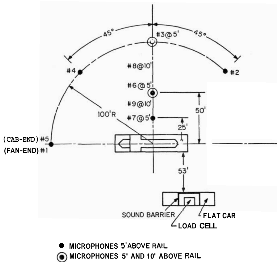
FIG. 3.4. BASELINE MICROPHONE LOCATIONS.
