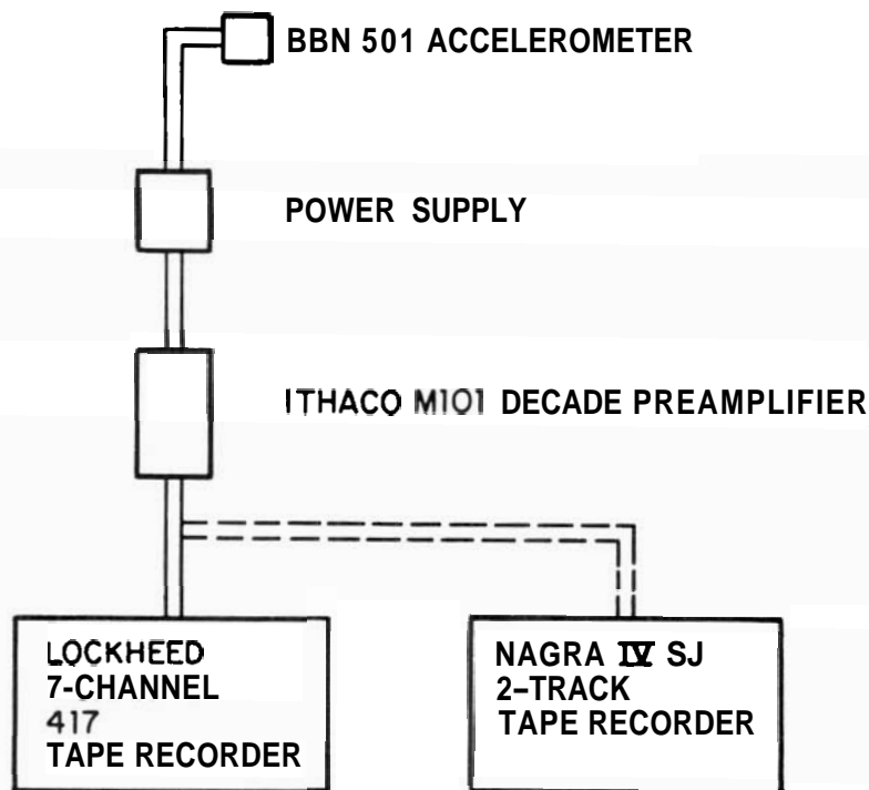
FIG. 3.7. TYPICAL ACCELEROMETER INSTRUMENTATION CHAIN.
