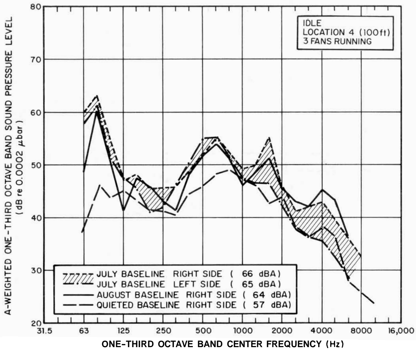
FIG. A.10. LOCOMOTIVE BASELINE NOISE, IDLE, MICROPHONE LOCATION 4.
