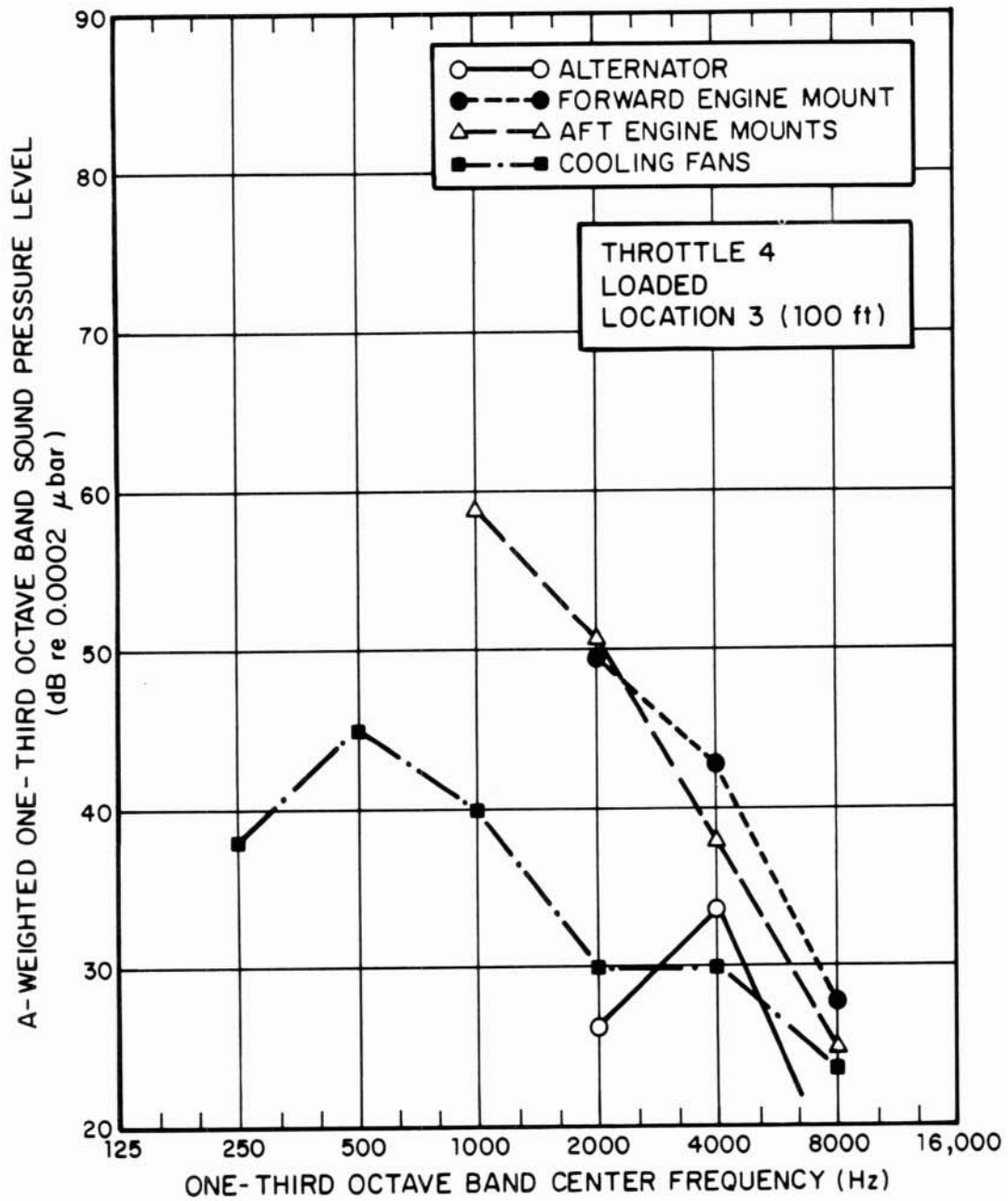
FIG. D.4. STRUCTUREBORNE NOISE AT THROTTLE 4, FULL LOAD, LOCATION 3.
