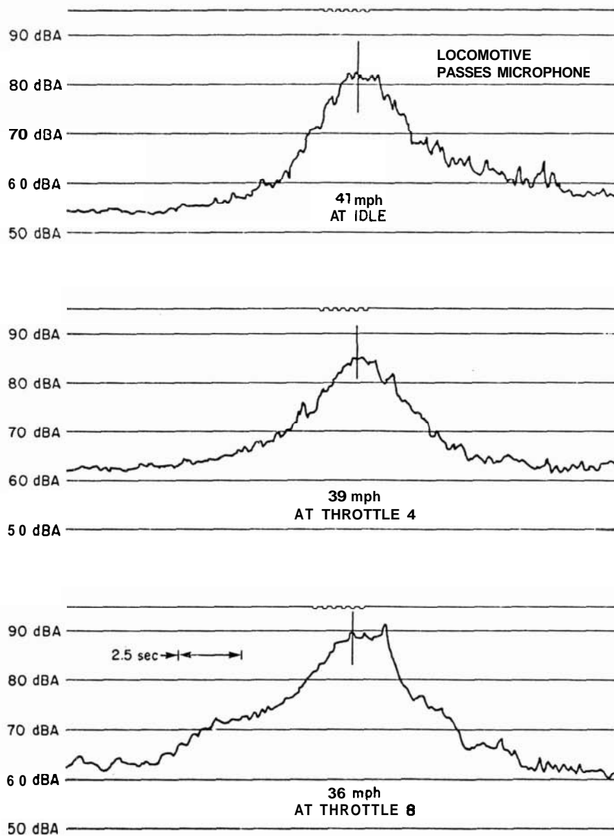
FIG. 4.3. LOCOMOTIVE PASS-BY AT 50 FT (WEST).
