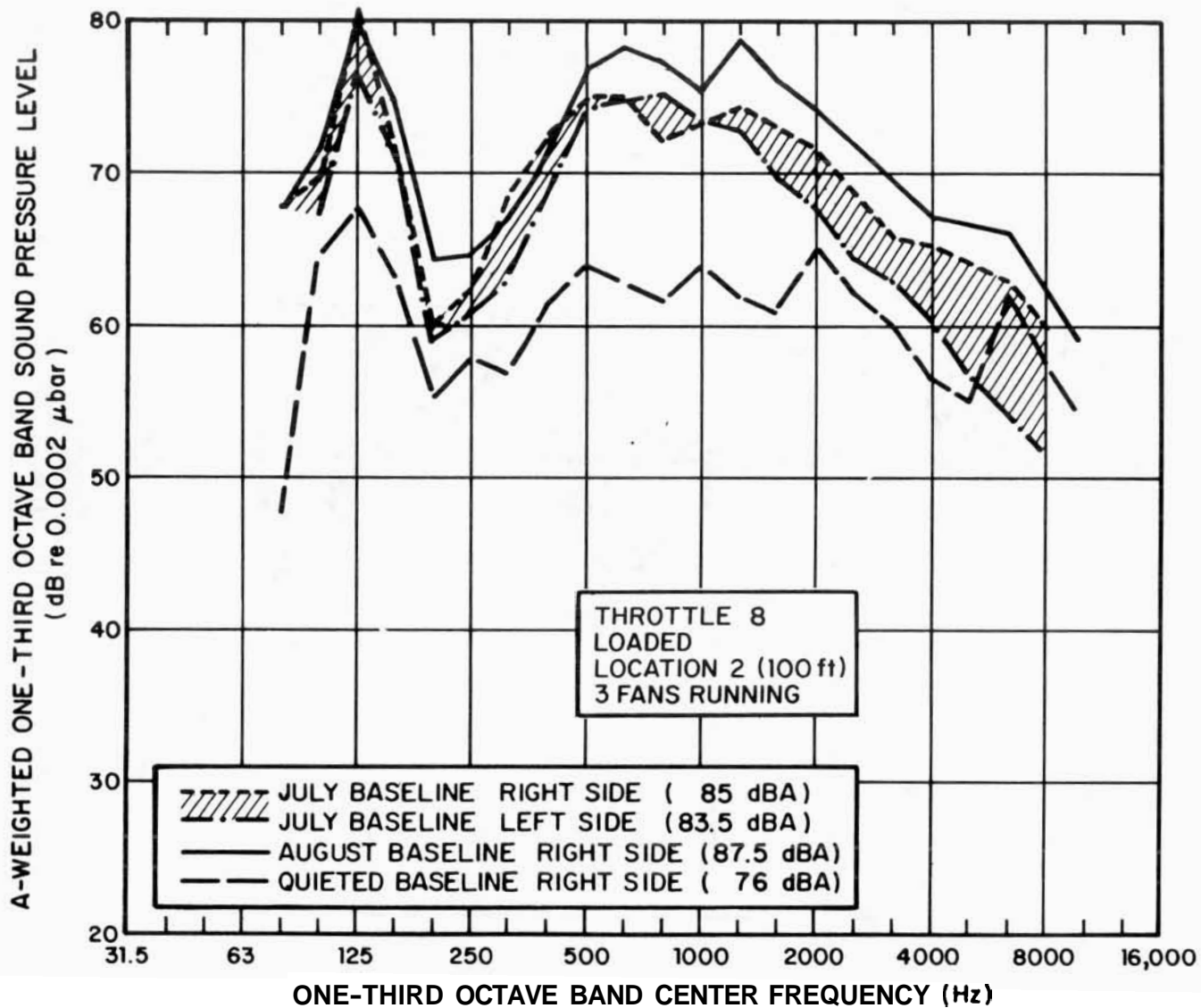
FIG. A.6. LOCOMOTIVE BASELINE NOISE, THROTTLE 8, FULL LOAD, MICROPHONE LOCATION 2.
