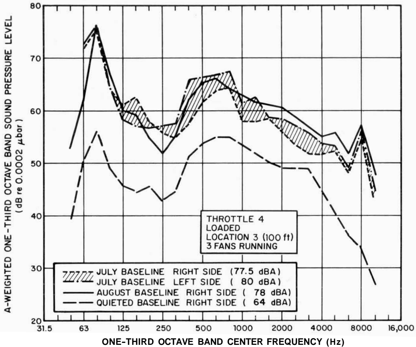
FIG. A.8. LOCOMOTIVE BASELINE NOISE, THROTTLE 4, MICROPHONE LOCATION 3.
