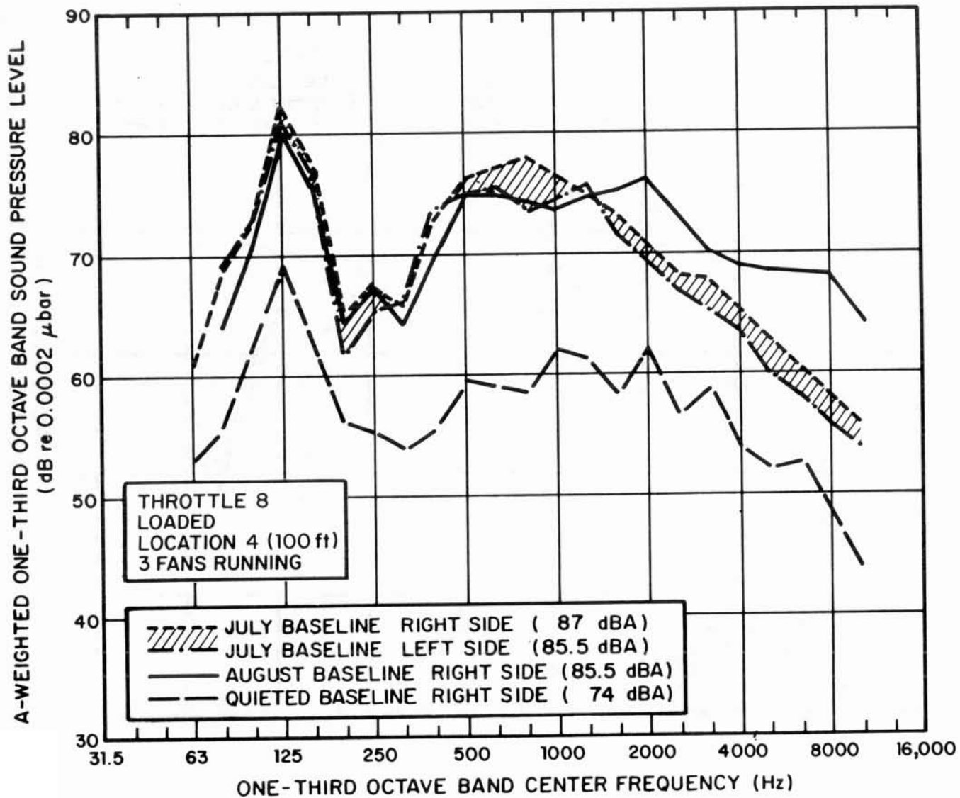
FIG. A.12. LOCOMOTIVE BASELINE NOISE, THROTTLE 8, FULL LOAD, MICROPHONE LOCATION 4.
