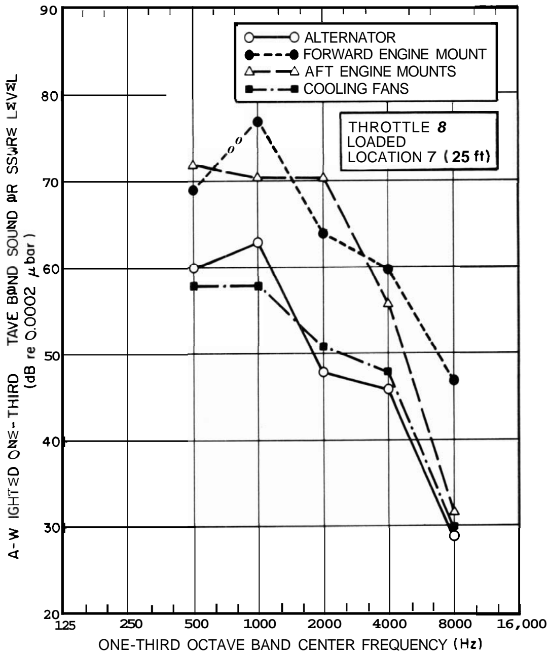
FIG. 0.8. STRUCTUREBORNE NOISE AT THROTTLE 8, FULL LOAD, LOCATION 7.
