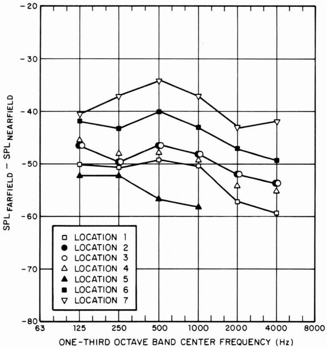
FIG. C.3. ENGINE/ALTERNATOR AIRBORNE PATH TRANSFER FUNCTION.
