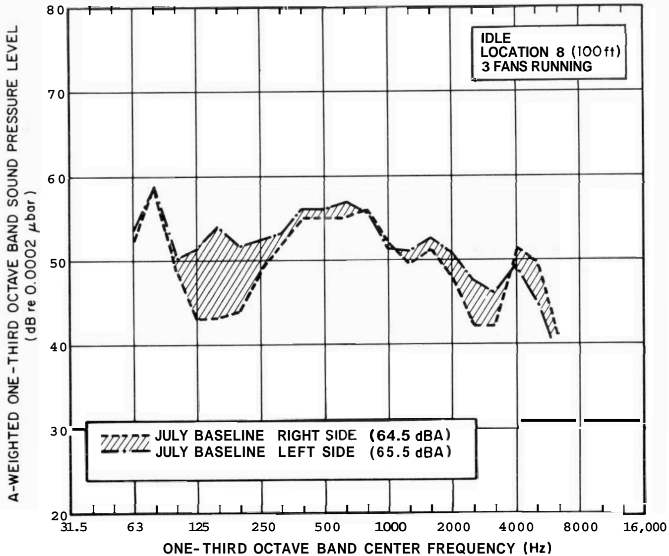
FIG. A.22 LOCOMOTIVE BASELINE NOISE, IDLE, MICROPHONE LOCATION 8.
