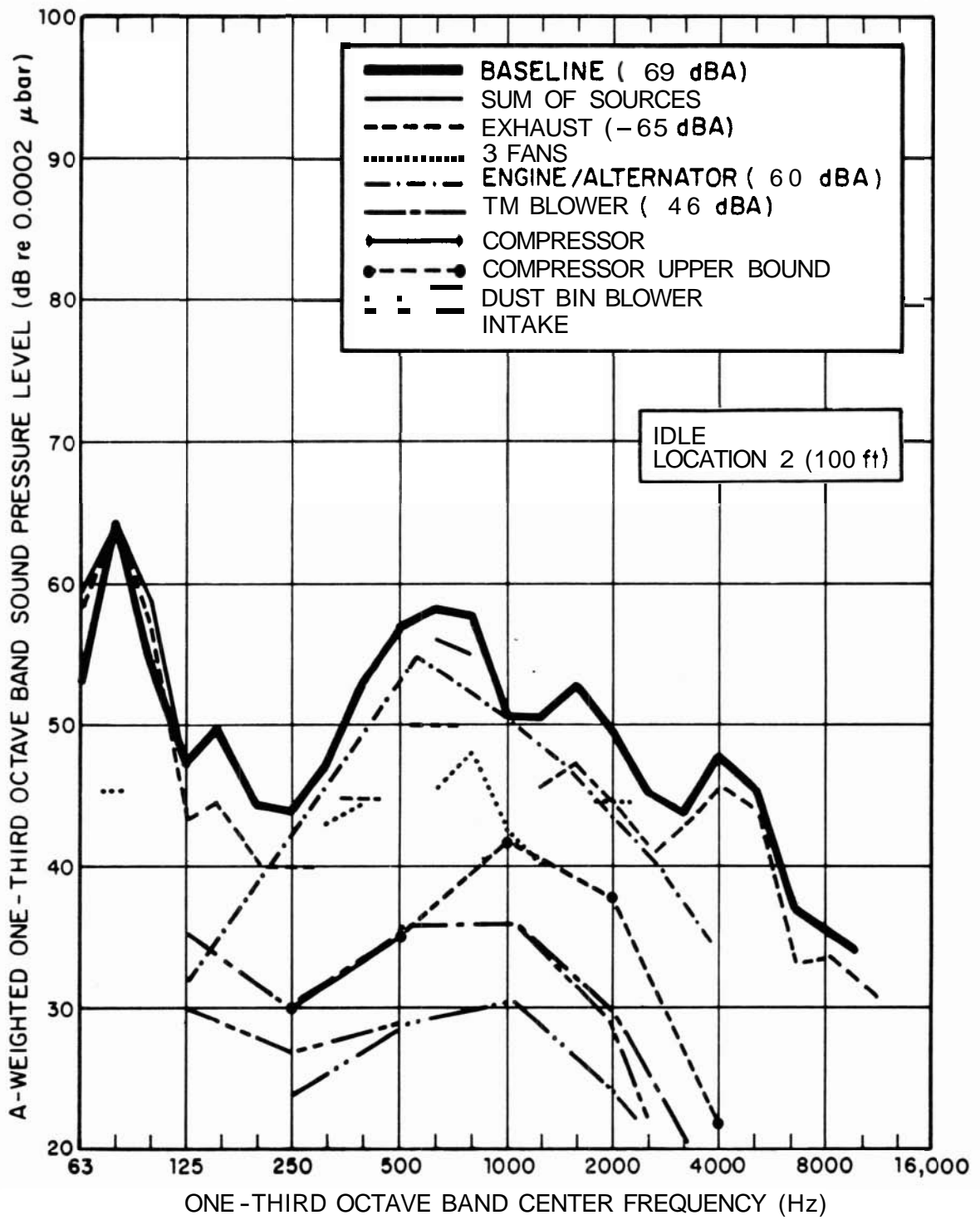
FIG. 8.3. SOURCE SPECTRA AT IDLE, MICROPHONE LOCATION 2.
