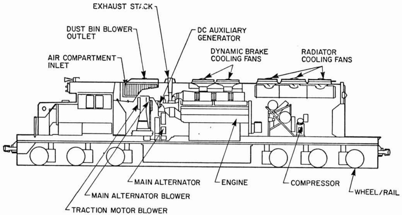
FIG. 2.2. MAJOR NOISE SOURCE LOCATIONS IN THE SD40-2 LOCOMOTIVE.
