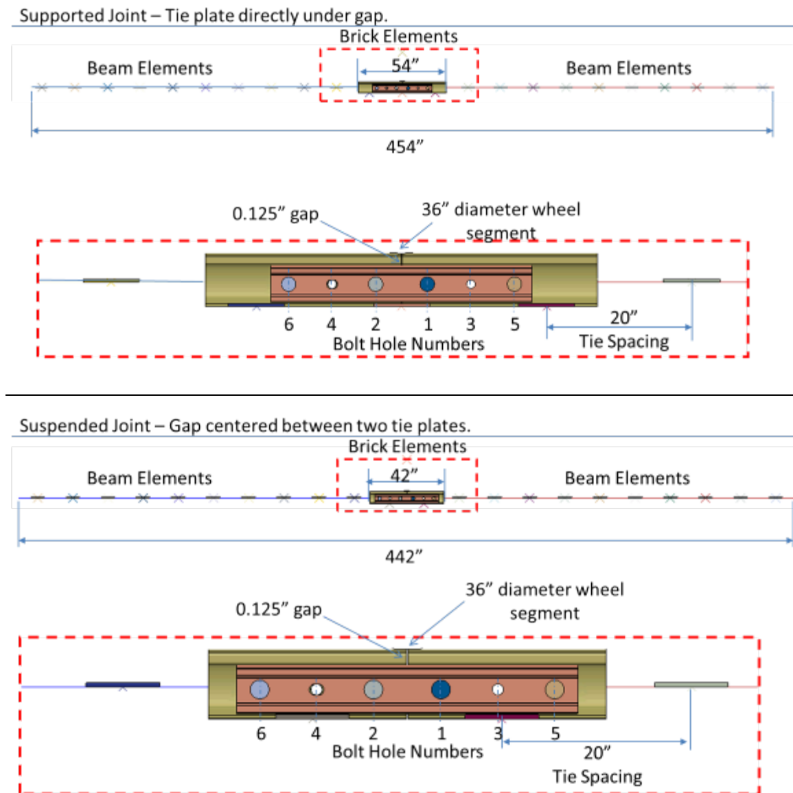
Figure 32. Finite Element Model Setup for Supported and Suspended Joints
