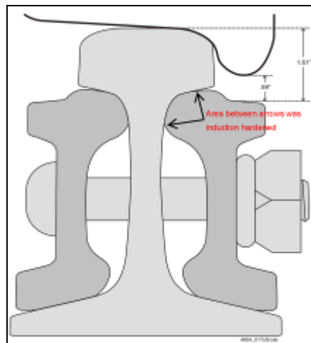
Figure 15. Locations of the Induction Hardened Areas on the Joint Bars
