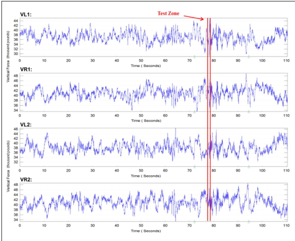
Figure 27. Time History for IWS Vertical Wheel Force Data (1/4-in Mismatch, 10 mph)
