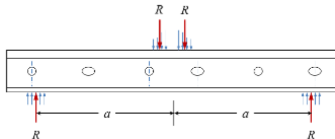
Figure 34. Joint Bar Reactions under Positive Bending
