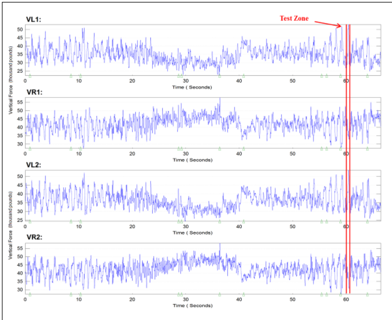
Figure 25. Time History for IWS Vertical Wheel Force Data (1-in Gap, 45 mph)
