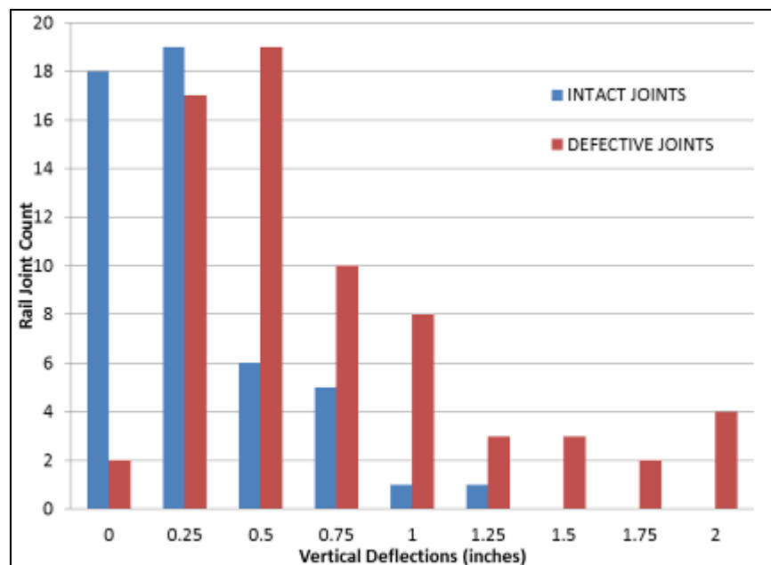
Figure 6. Distribution of Vertical Deflections for Intact and Defective Rail Joints
