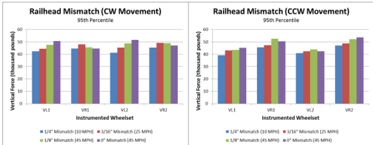
Figure 26. Plots of the 95 th Percentile for IWS Vertical Wheel Force Data (Railhead Mismatch)
