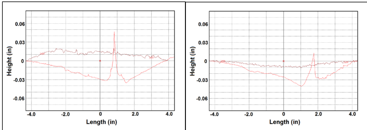
Figure 19. Pre- and Post-Test Longitudinal Profiles for an Untreated (left) and a Post-Hardened (right) Joint Bar
