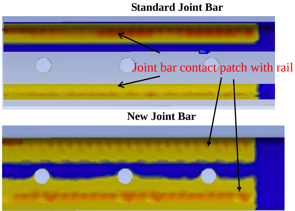
Figure 37. Calculated Contact between Rail and Joint Bar by Design
