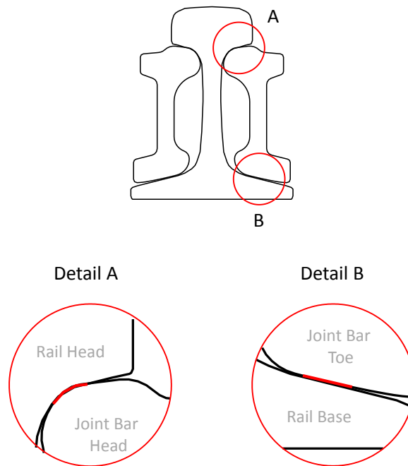
Figure 35. Potential Locations for Contact between Rail and Joint Bar
