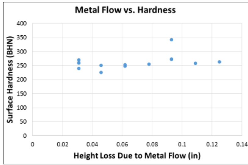
Figure 31. Plot of the Height Loss Due to Metal Flow against Surface Hardness
