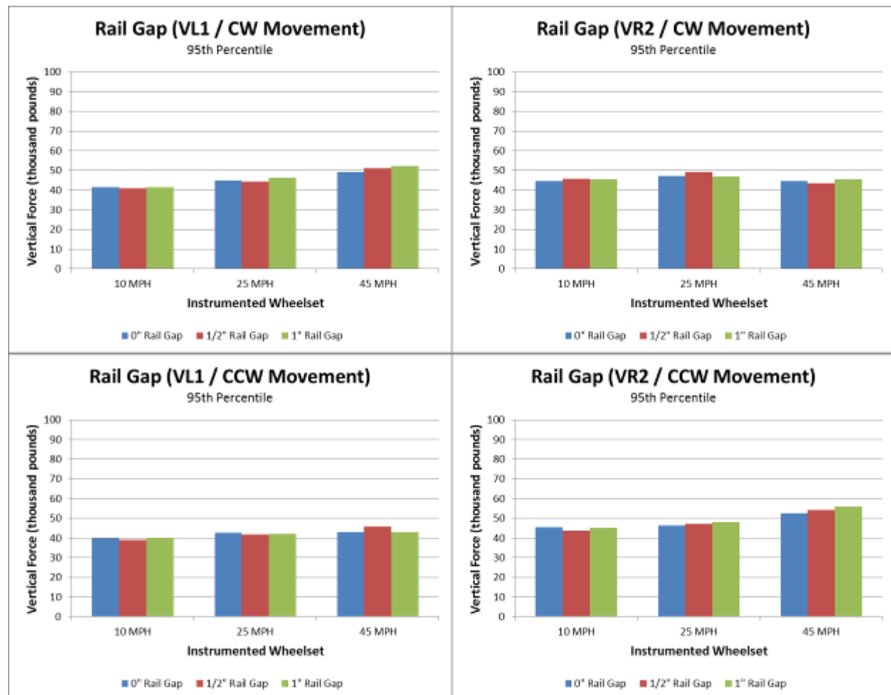
Figure 24. Plots of the 95 th Percentile for IWS Vertical Wheel Force Data (Rail Gaps)
