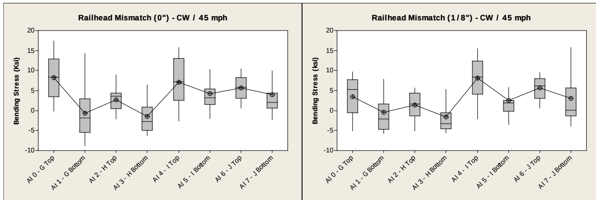
Figure 29. Box Plots of the Bending Stresses under the IWS for Each Circuit (Railhead Mismatch)
