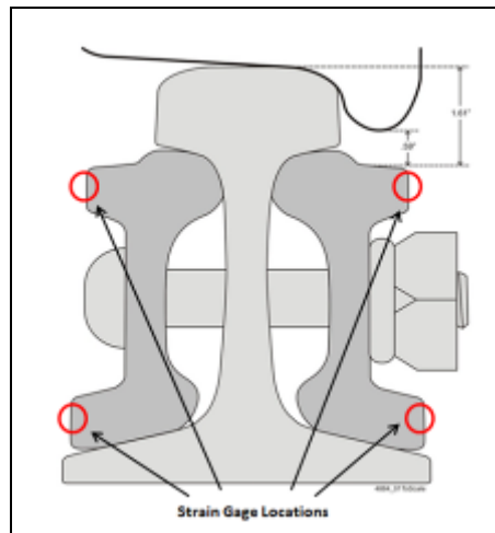
Figure 10. Location of Bending Circuits along the Central Axis
