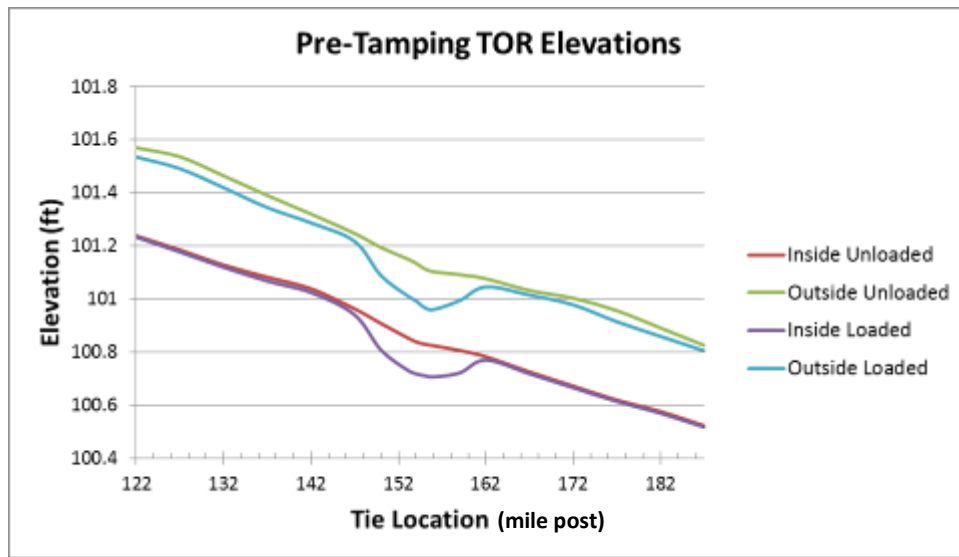
Figure 12. Plot of the Pre-Tamping TOR Elevations for the Test Zone, for both Loaded and Unloaded Scenarios
