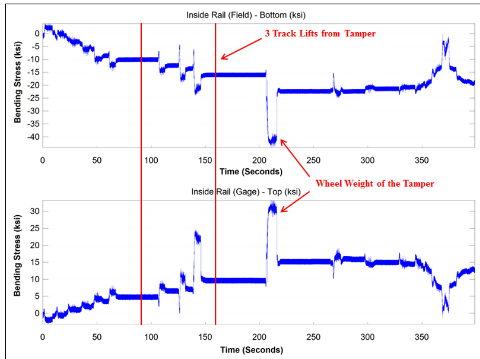
Figure 14. Stripcharts Presenting the Bending Stresses for Two of the Four Joint Bars
