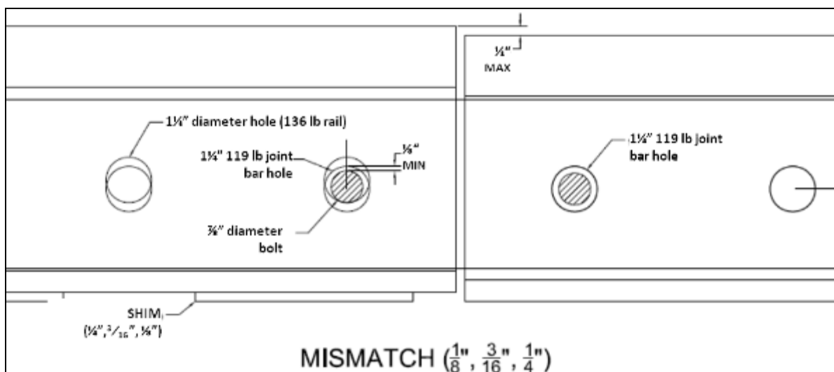
Figure 23. Plan View of an Example Railhead Mismatch Test Setup (1/2 in)
