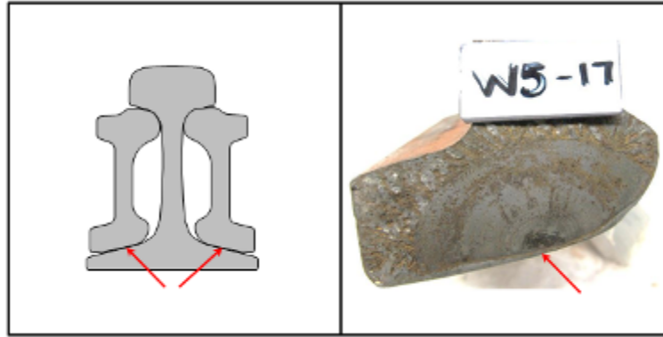
Figure 3. Bottom Center Crack
