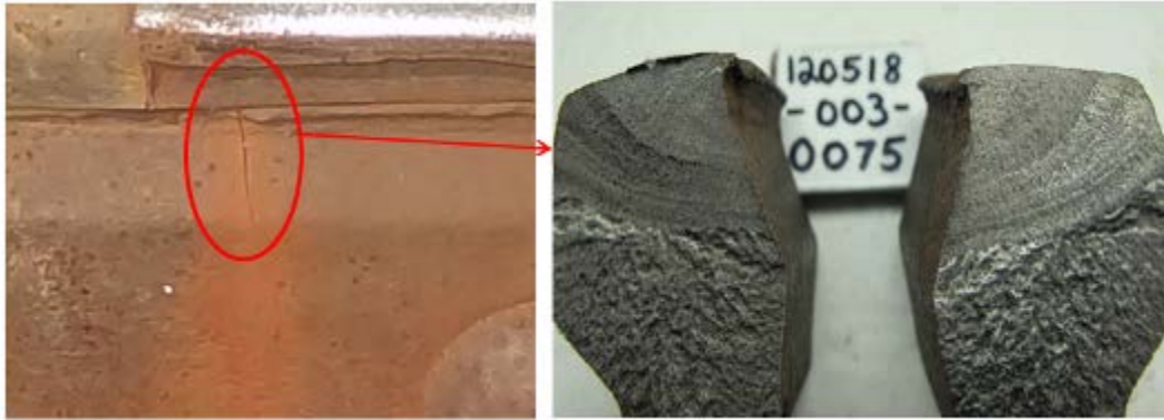
Figure 1. Top Center Crack
