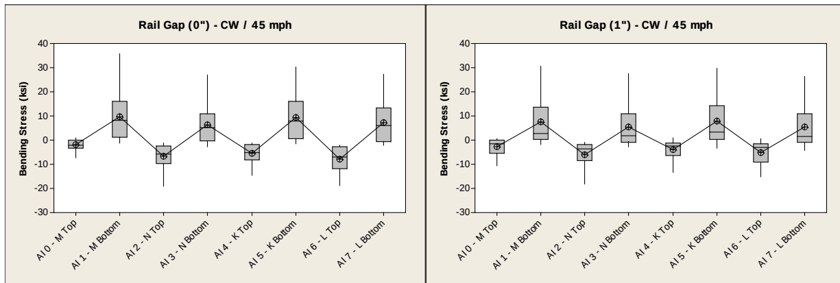
Figure 28. Box Plots of the Bending Stresses under the IWS for Each Circuit (Rail Gap)
