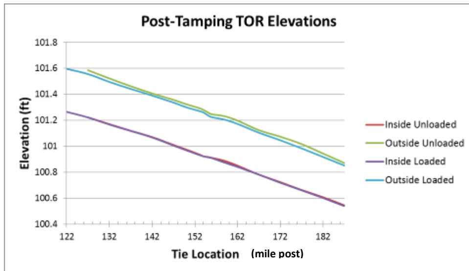
Figure 13. Plot of the Post-Tamping TOR Elevations for the Test Zone, for both Loaded and Unloaded Scenarios
