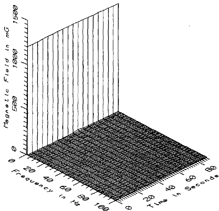
MET046 - 10cm ABOVE FLOOR AT SHADY GROVE DISPATCHER'S SEAT
