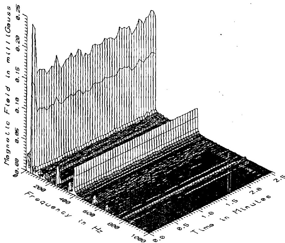
TR7018 - 3M WEST OF HIGH STEEL GUIDEWAY, 25M NORTH OF PROFILE
