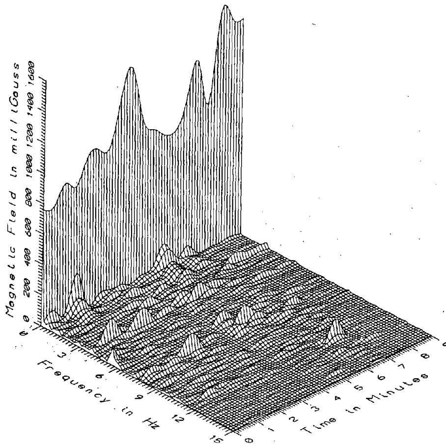
TR7008 - FLOOR LEVEL - WINDOW SEAT AT REAR OF PASSENGER SECTION, CAR#2
