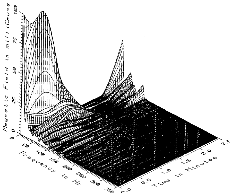
IP7011 - AISLE SEAT - FLOOR LEVEL IN MIDDLE OF PASSENGER SECTION, CAR#2
