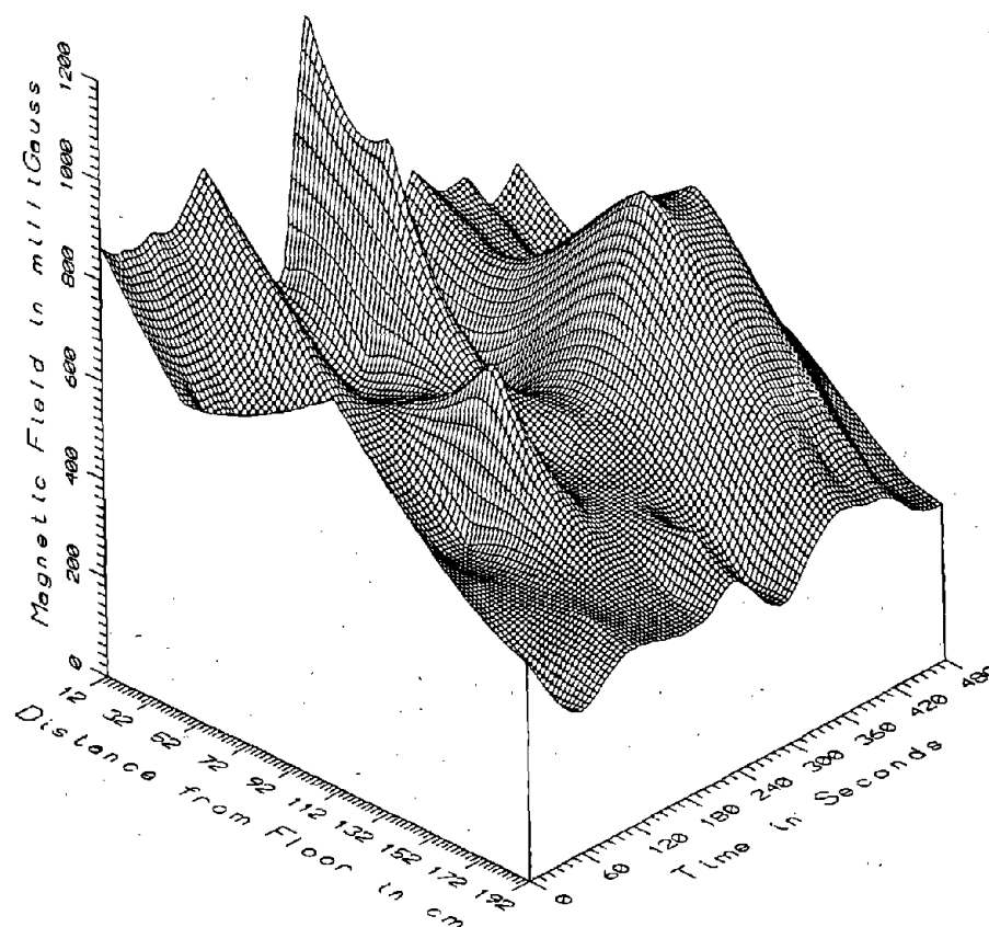
TR7003 - AISLE SEAT IN MIDDLE OF PASSENGER SECTION, CAR2 - DC
