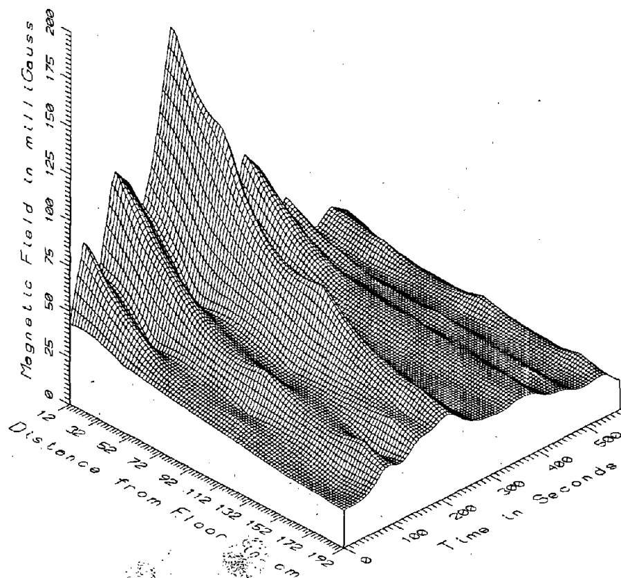
TR7010, REAR ENGINEER SECTION, CAR#2 - LOW FREQUENCY 5-45Hz
