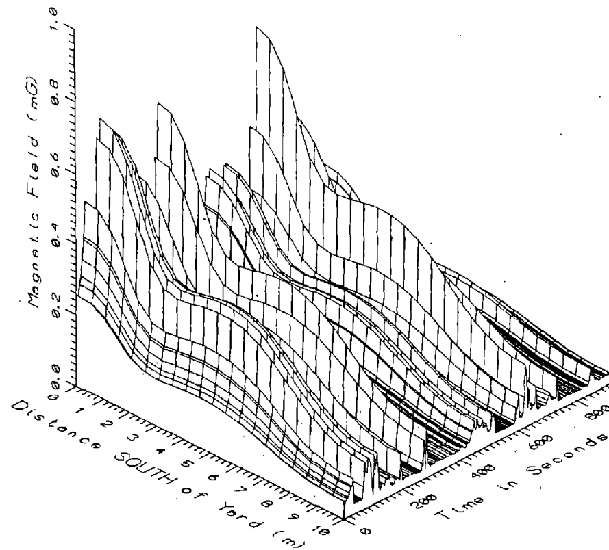
TR7022, OUTPUT TRANSFORMER YARD - HIGH FREQUENCY, 305-2560Hz
