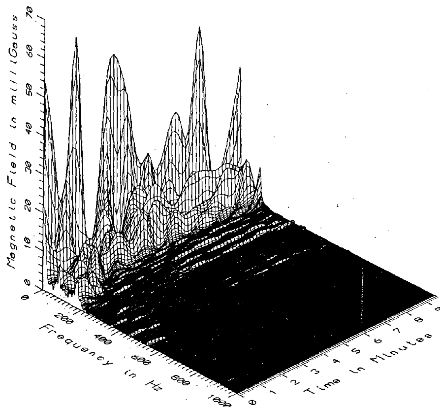
TR7010 - REFERENCE PROBE - BULKHEAD IN REAR OF PASSENGER SECTION, CAR#2
