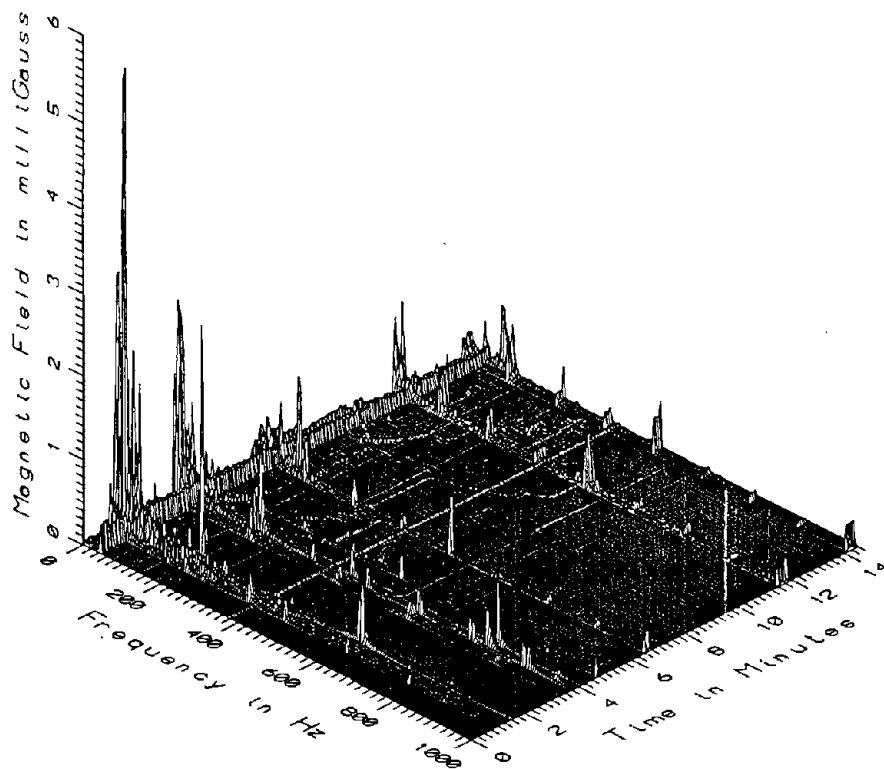
TR7030 - 25M NORTH OF INVERTER BUILDING
