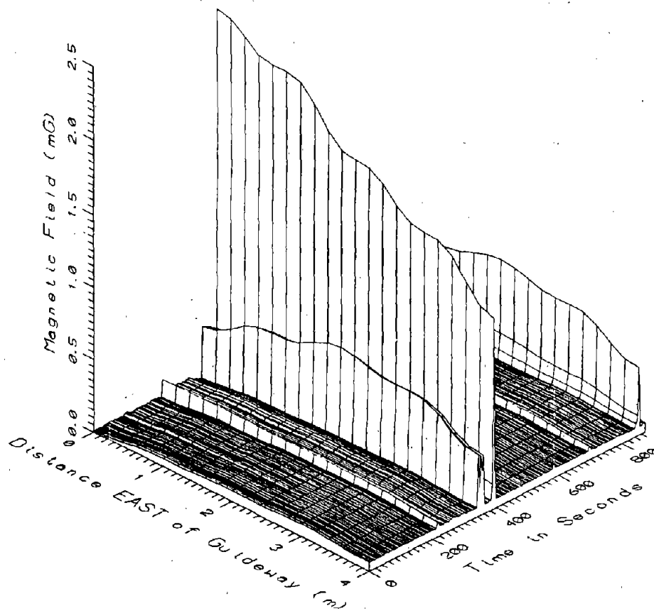
TR7032, SOUTH LOOP FEEDER CABLE 3.5m EAST OF GUIDEWAY - HIGH FREQ, 65-2560Hz
