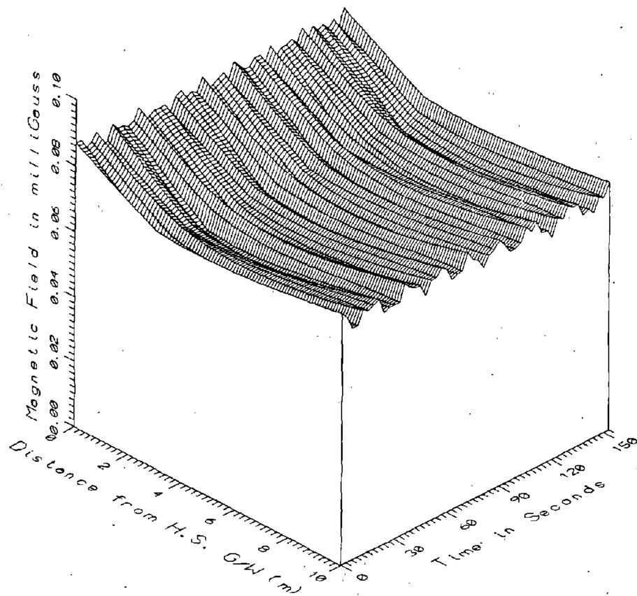
TR701B, HIGH STEEL GUIDEWAY - HIGH FREQUENCY, 305-2560Hz
