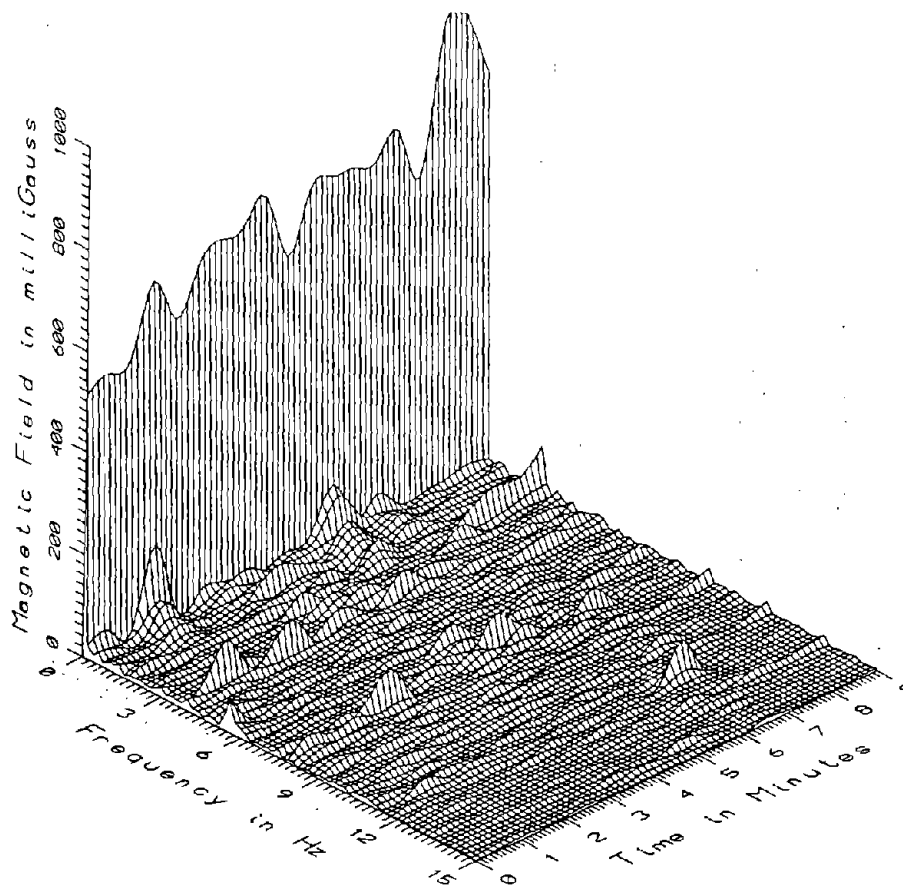
TR7008 - SEAT LEVEL - WINDOW SEAT AT REAR OF PASSENGER SECTION, CAR#2
