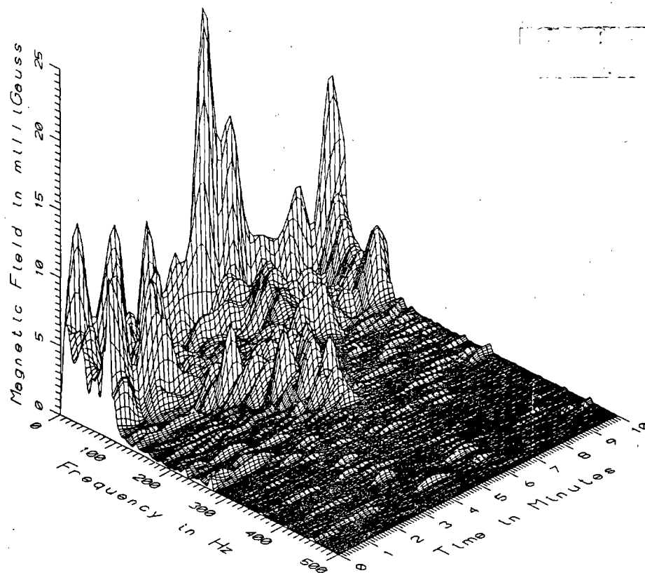
TR7002 - SEATED HEAD LEVEL - AISLE SEAT IN MIDDLE OF PASSENGER SECTION, CAR#2
