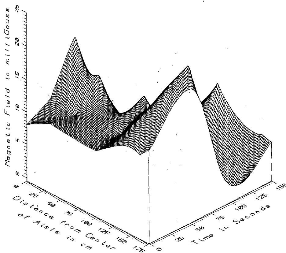
TR7011, FLOOR LEVEL IN MIDDLE OF PASSENGER SECTION, CAR2 - POWER FREQ. 50-60Hz
