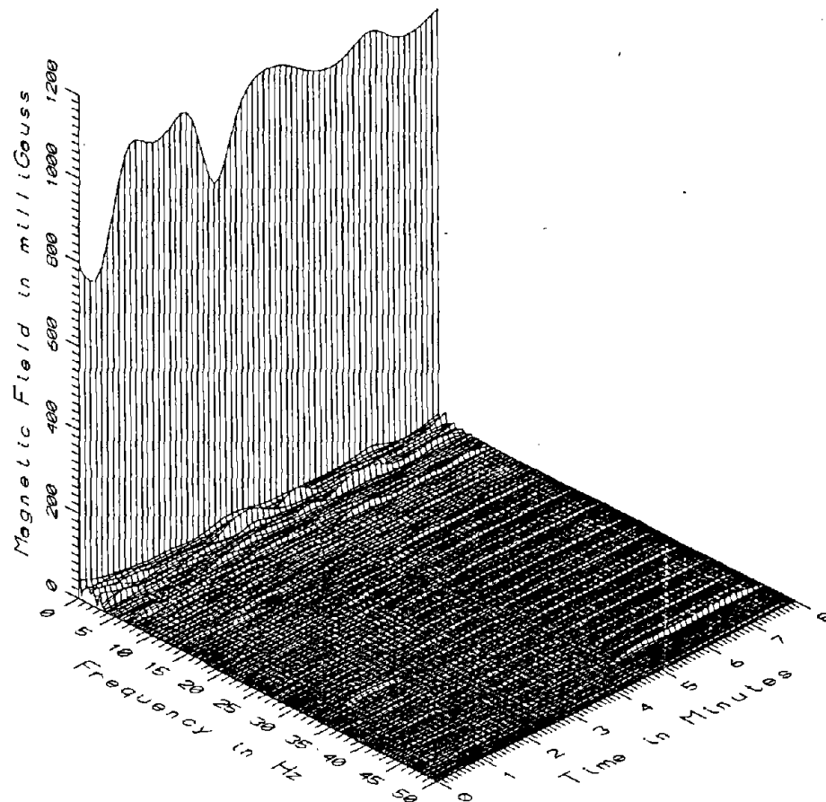
TR7009 - SEATED HEAD LEVEL - VIP SECTION, CAR#2
