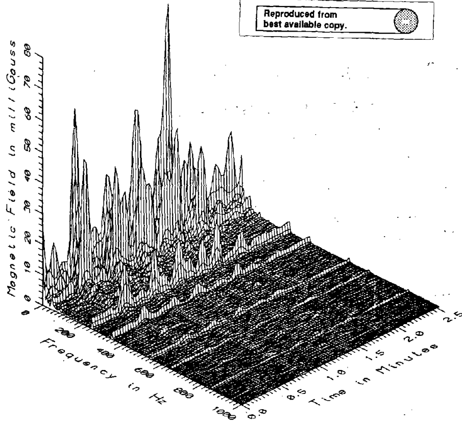
TR7026 - UNDER LOW CONCRETE GUIDEWAY OUTSIDE MAINTENANCE FACILITY
