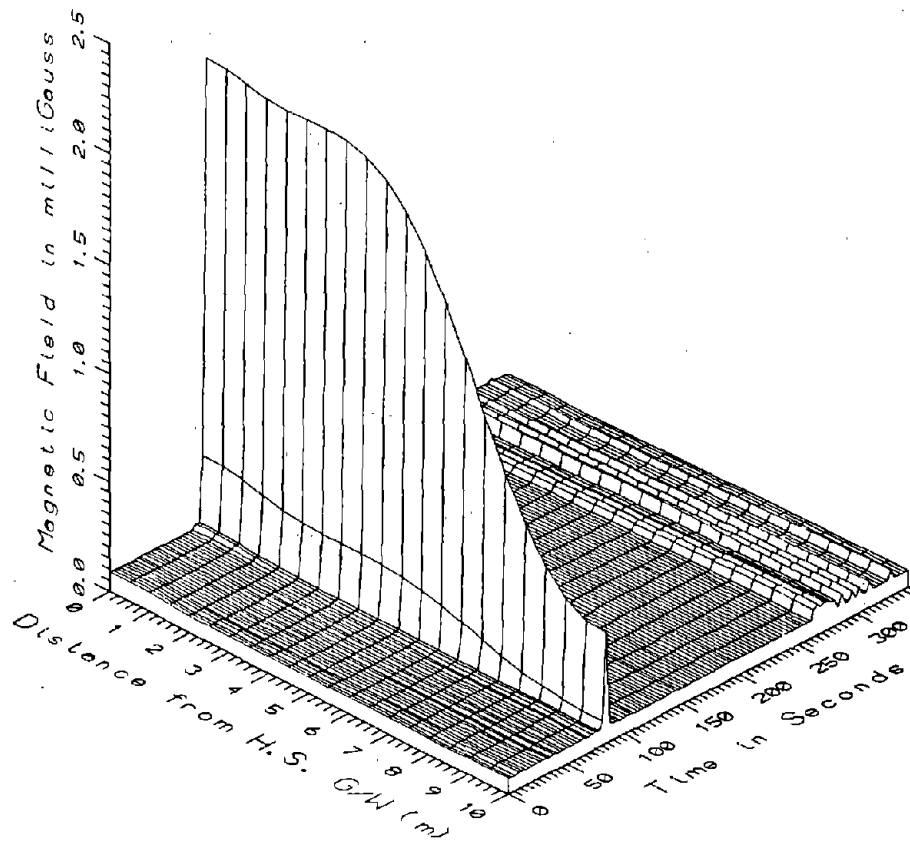
TR7014, HIGH STEEL GUIDEWAY - HIGH FREQUENCY, 305-2560Hz
