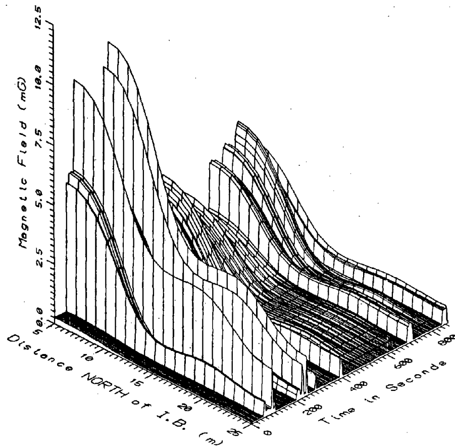
TR7030, INVERTER BUILDING - HIGH FREQUENCY, 305-2560Hz
