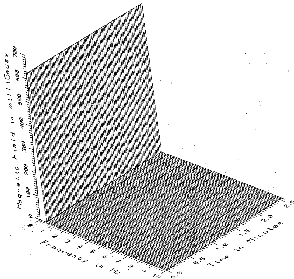
TR701B - UNDER CENTER OF HIGH STEEL GUIDEWAY
