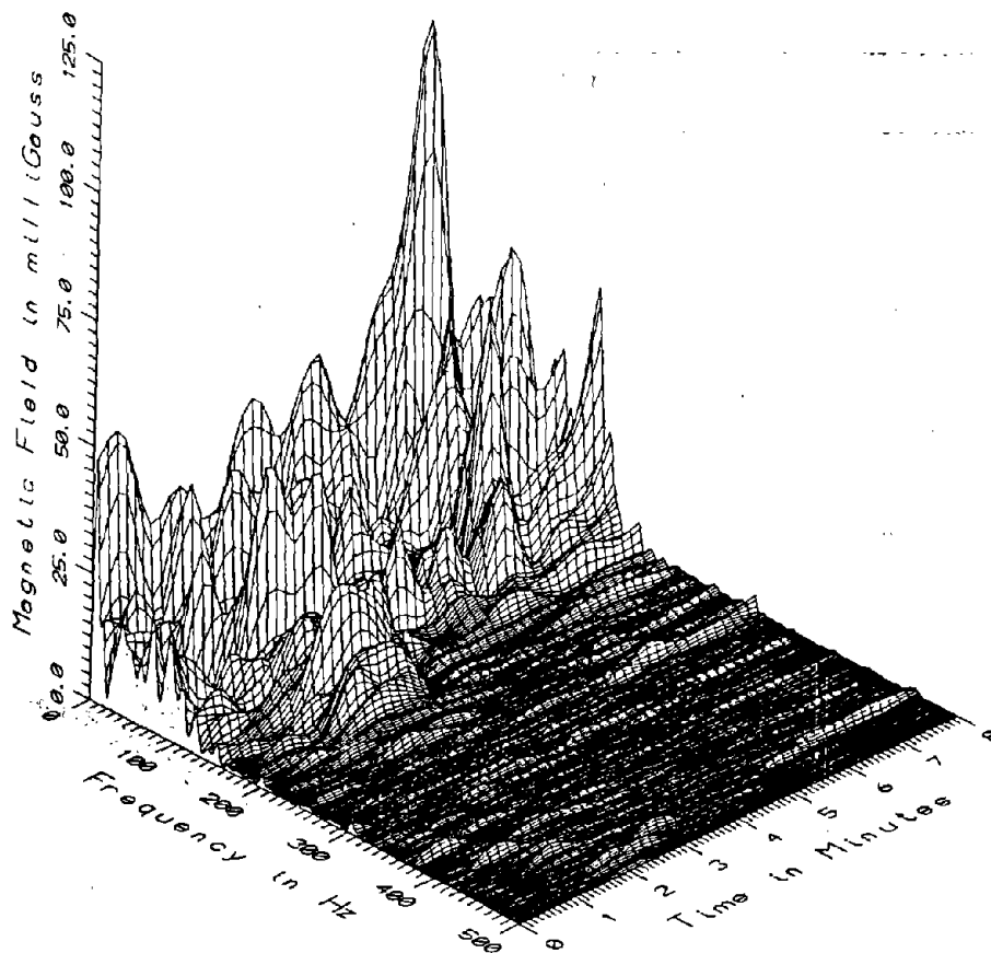
TR7003 - FLOOR LEVEL - AISLE SEAT IN MIDDLE OF PASSENGER SECTION, CAR#2
