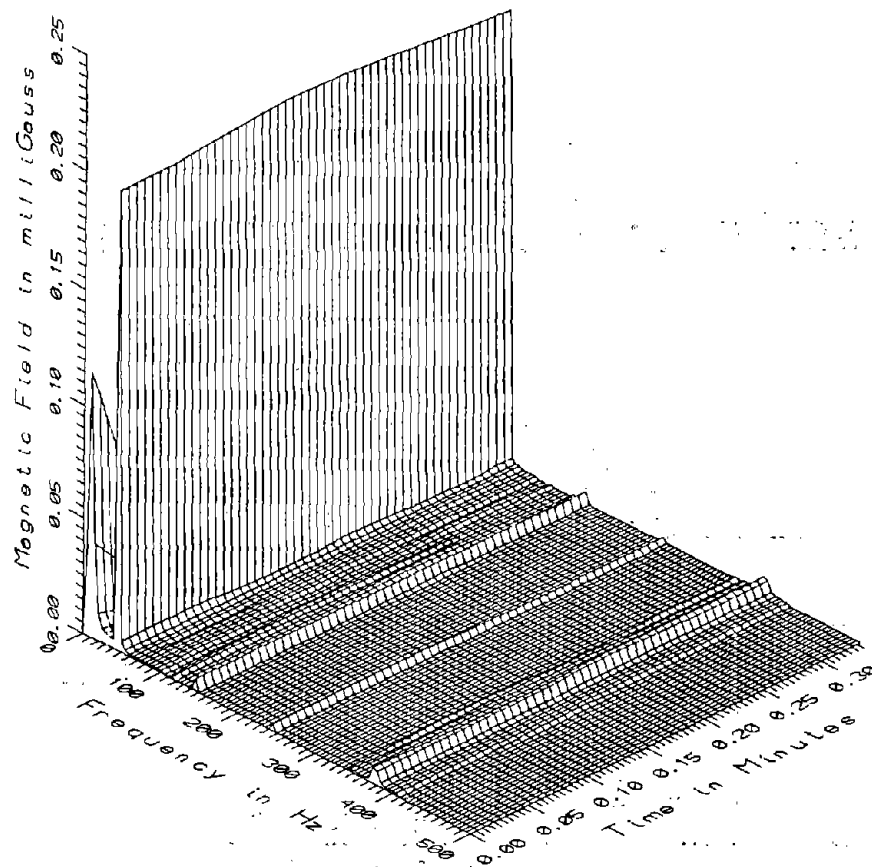
TR7031 - 0.5M EAST OF SOUTH LOOP FEEDER CABLE, GROUND LEVEL
