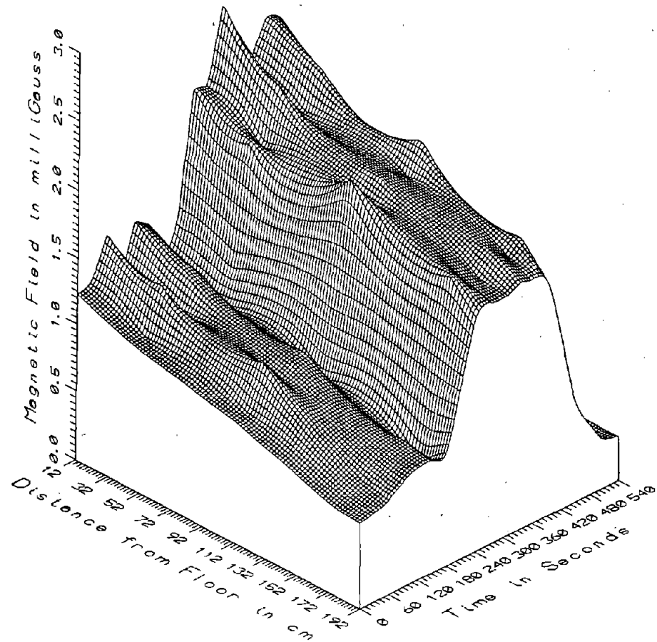
TR700B, WINDOW SEAT IN REAR OF PASSENGER SECTION, CAR2 - HIGH FREQ. 305-2560Hz
