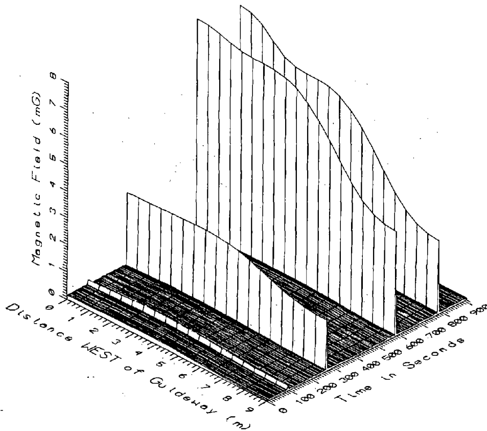
TR7020, GUIDEWAY AT LOADING PLATFORM - POWER FREQUENCY, 50-60Hz
