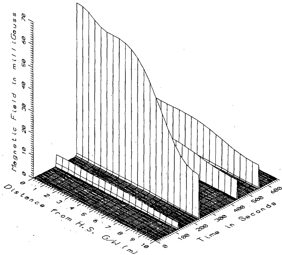
TR7013, HIGH STEEL GUIDEWAY - POWER HARMONICS, 65-300Hz
