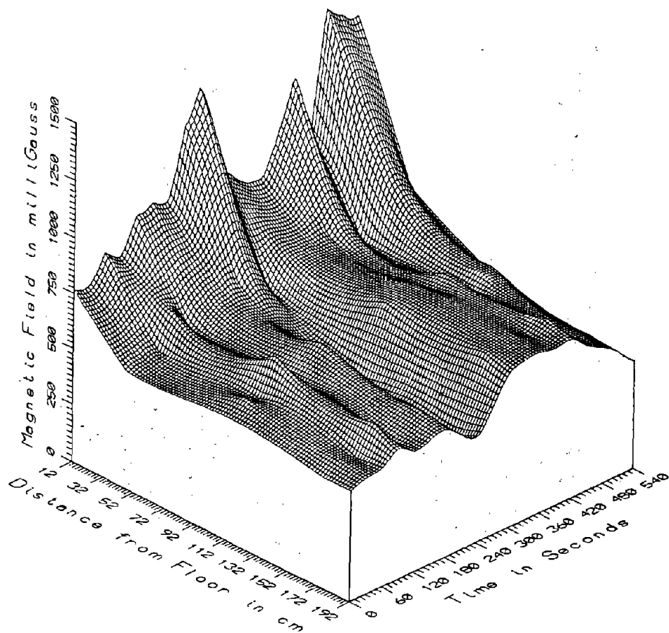
TR700C - WINDOW SEAT IN REAR OF PASSENGER SECTION, CAR2 - DC
