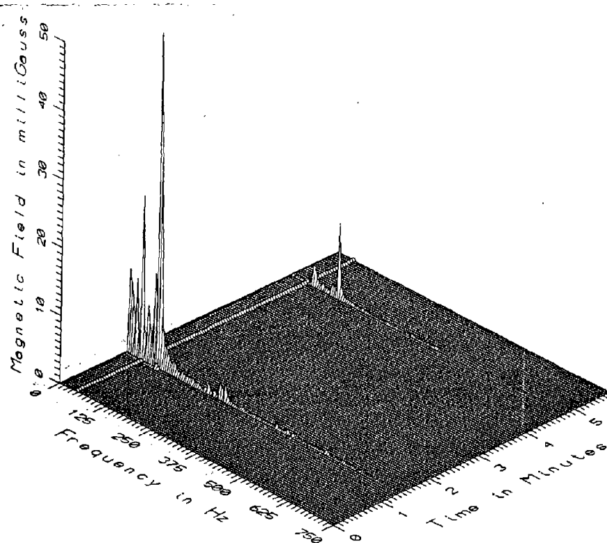
TR7014 - 3M WEST OF HIGH STEEL GUIDEWAY, 25M NORTH OF PROFILE
