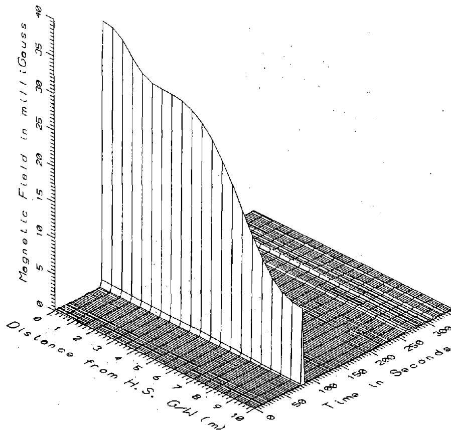
TR7014, HIGH STEEL GUIDEWAY - LOW FREQUENCY, 5-45Hz
