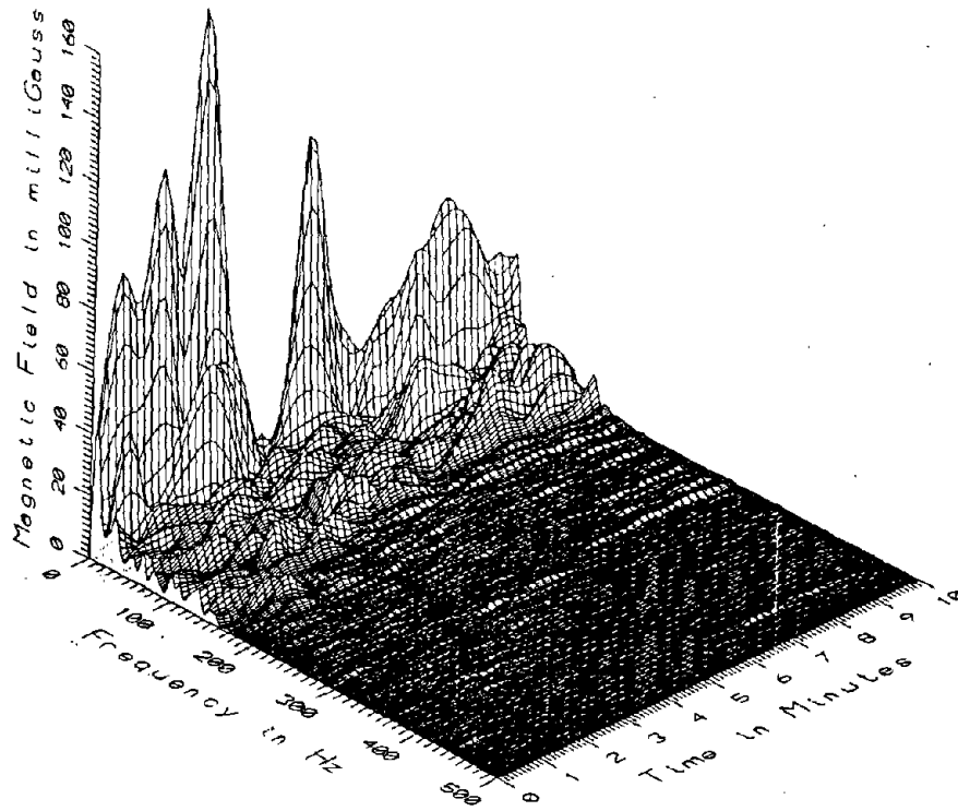
TR7001 - FLOOR LEVEL - WINDOW SEAT IN MIDDLE OF PASSENGER SECTION, CAR#2
