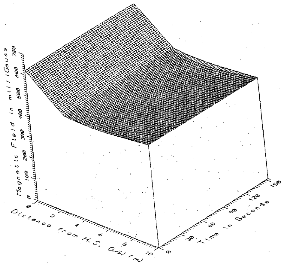
TR7018, HIGH STEEL GUIDEWAY - DC
