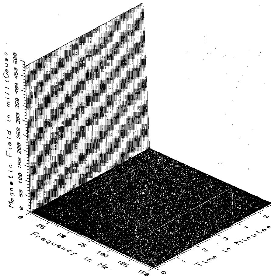
TR7014 - 10M WEST OF HIGH STEEL GUIDEWAY
