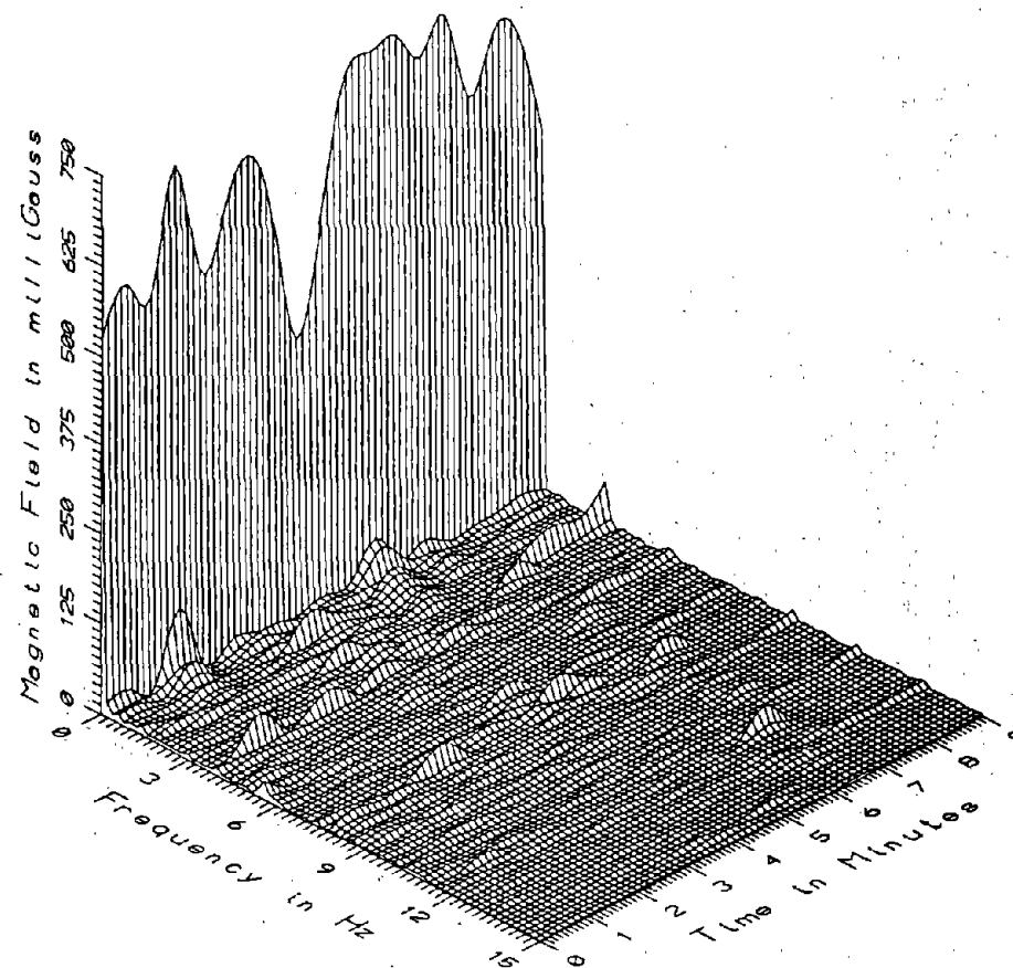
TR7008 - SEATED HEAD LEVEL - WINDOW SEAT AT REAR OF PASSENGER SECTION, CAR#7
