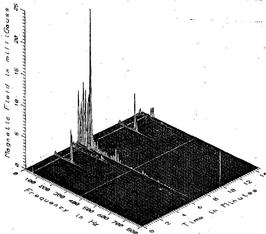
TR7032 - 1.5M WEST OF SOUTH LOOP FEEDER CABLE, GROUND LEVEL
