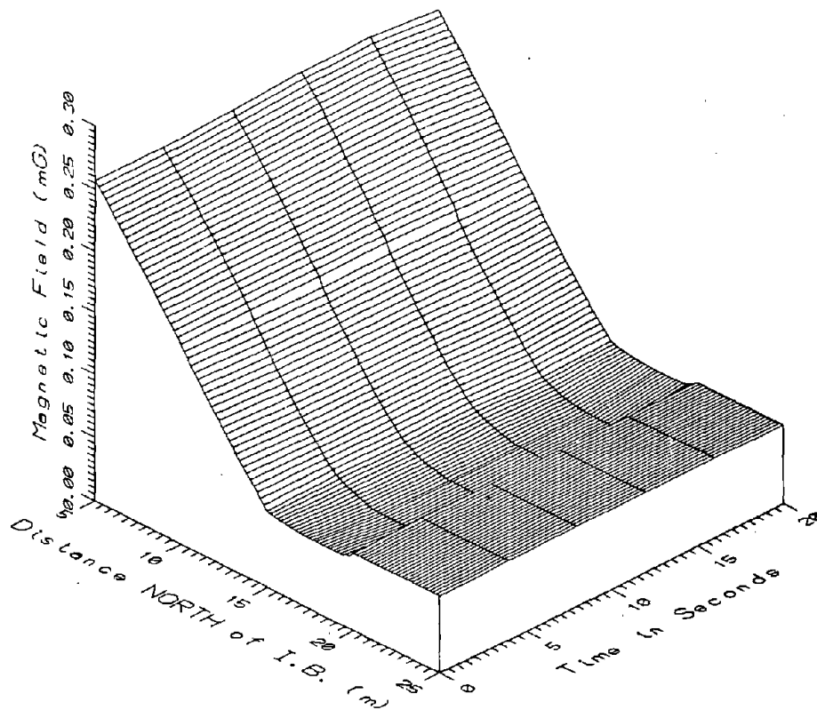
TR7028, INVERTER BUILDING - HIGH FREQUENCY, 305-2560Hz
