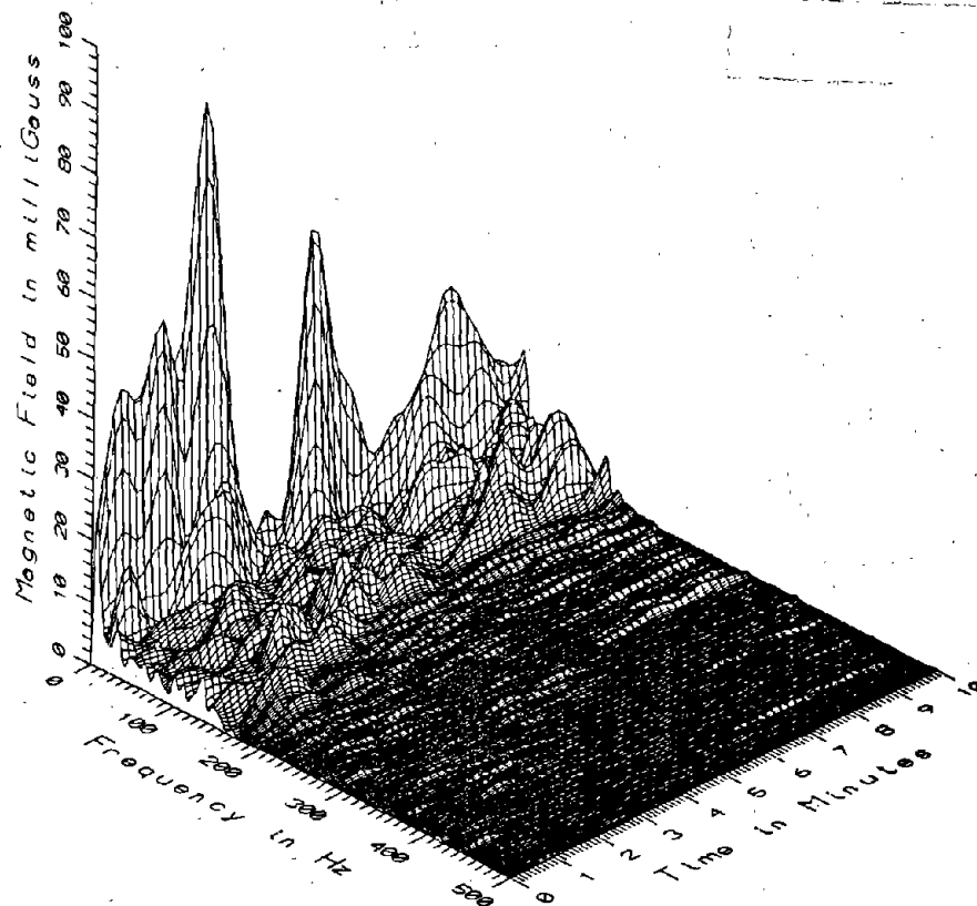
TR7001 - SEAT LEVEL - WINDOW SEAT IN MIDDLE OF PASSENGER SECTION, CAR#2
