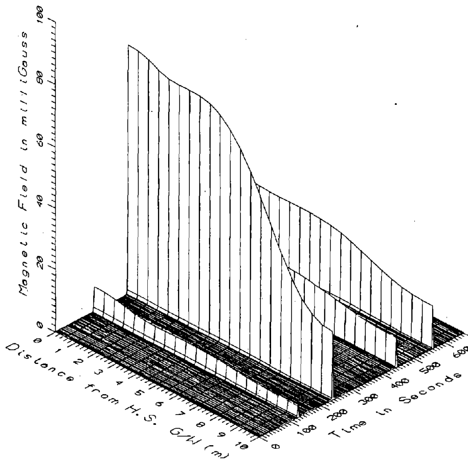
TR7013, HIGH STEEL GUIDEWAY - ALL FREQUENCIES, 5-2560Hz
