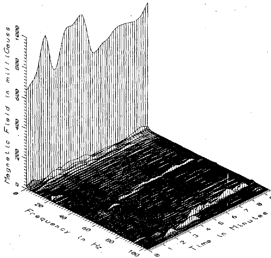
TR7010 - SEATED HEAD LEVEL - REAR ENGINE SECTION, CAR#2
