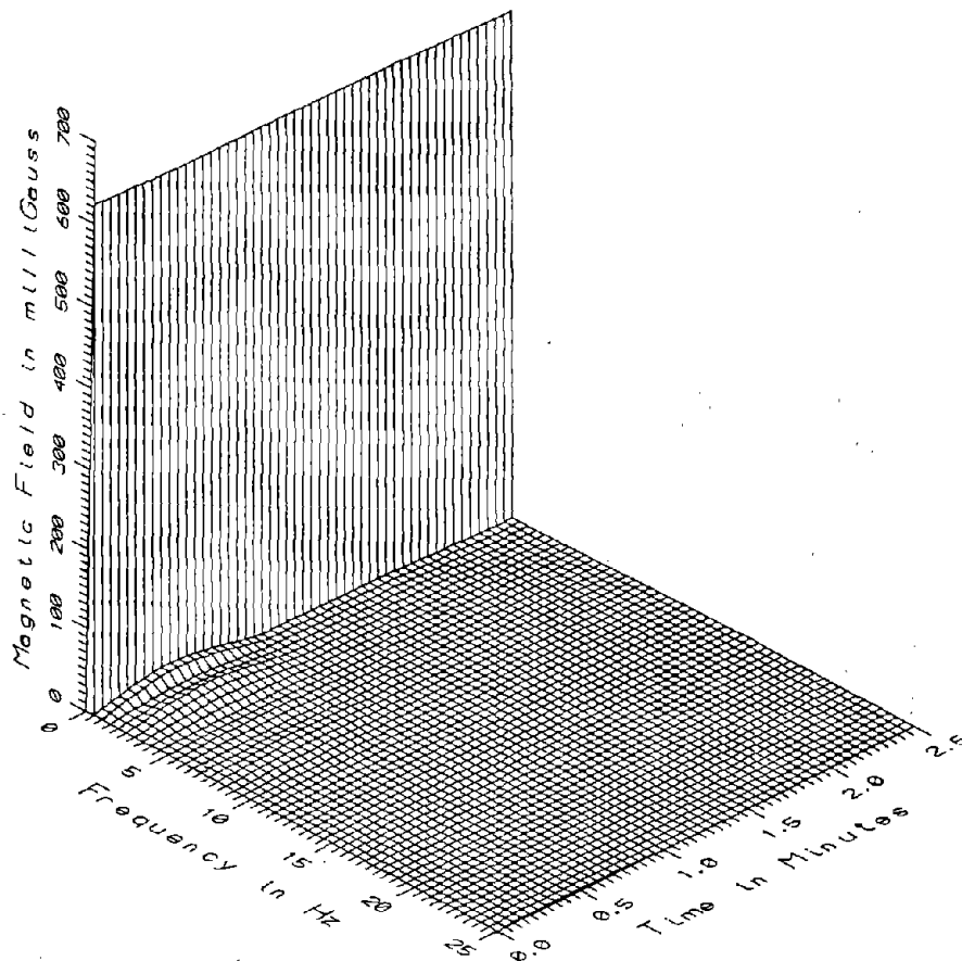
TR7012 - UNDER CENTER OF HIGH STEEL GUIDEWAY
