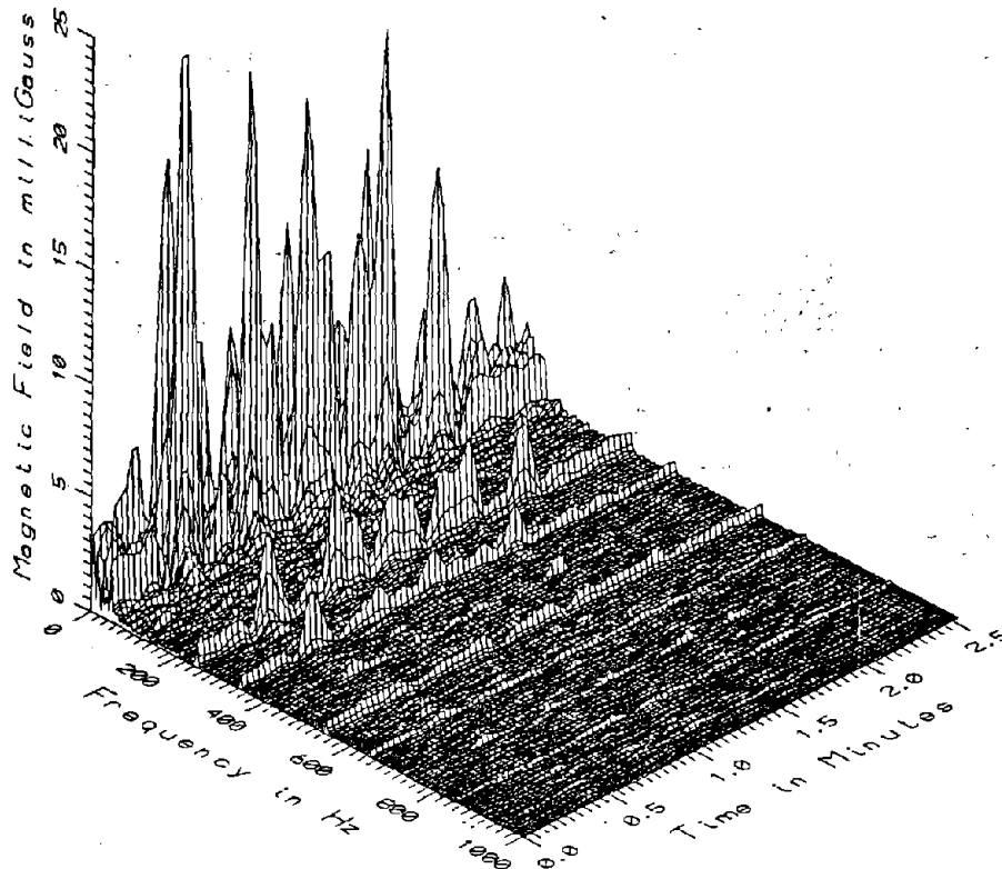
TR7026 - 3M NORTHWEST OF LOW CONCRETE GUIDEWAY OUTSIDE MAINTENANCE FACILITY
