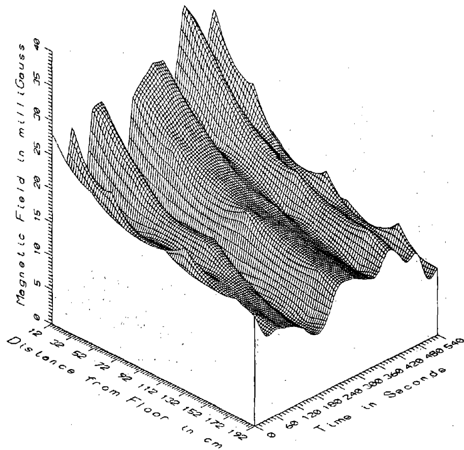
TR700B, WINDOW SEAT IN REAR OF PASSENGER SECTION, CAR2 - POWER HARM. 65-300Hz
