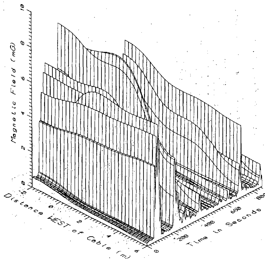
TR7030, BURIED CABLE FEEDING INVERTER BUILDING - LOW FREQUENCY, 5-45Hz
