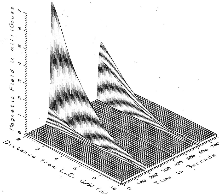
TR7019. LOW CONCRETE GUIDEWAY IN SOUTH LOOP - POWER FREQUENCY, 50-60Hz
