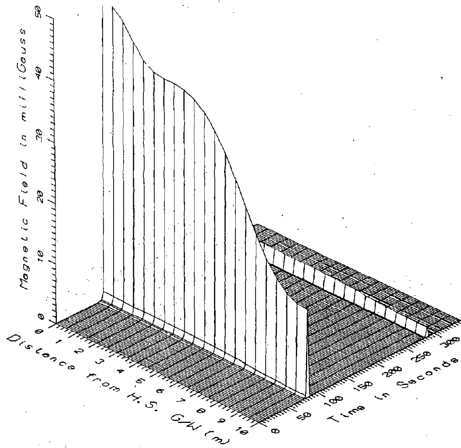
TR7014, HIGH STEEL GUIDEWAY - POWER HARMONICS, 65-300Hz
