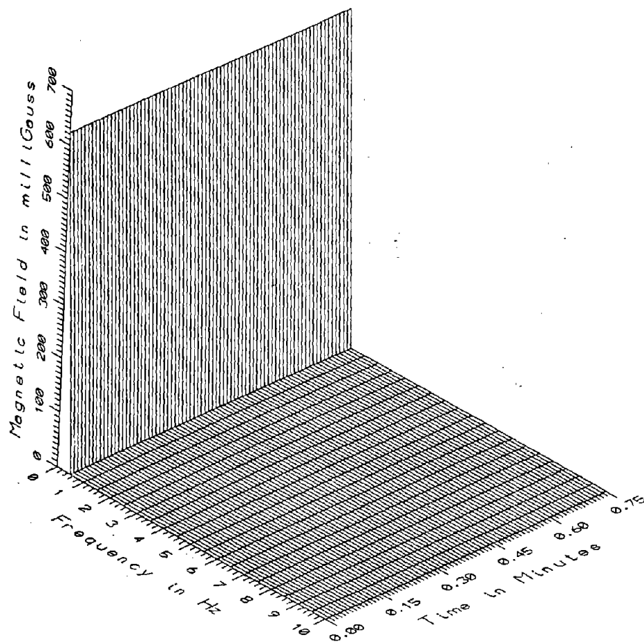
TR7017 - UNDER CENTER OF HIGH STEEL GUIDEWAY M-5
