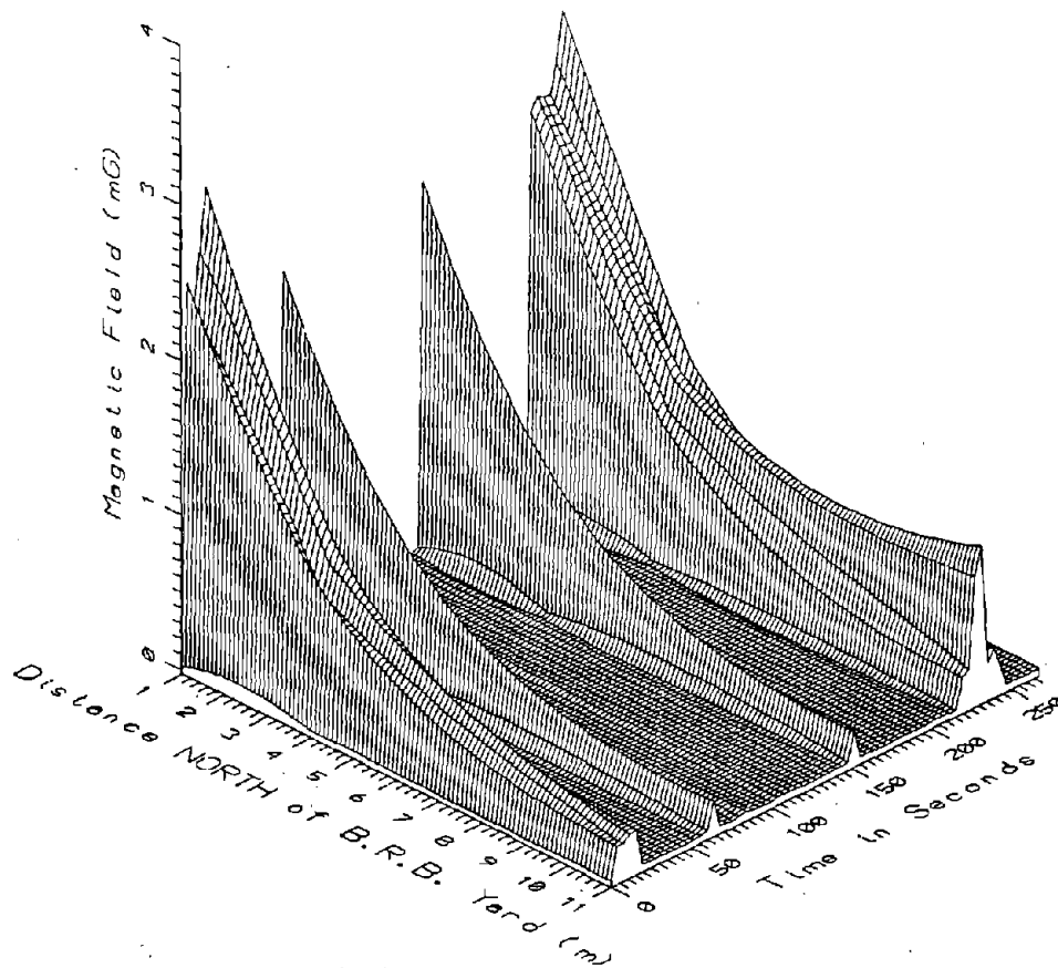
TR7024. BRAKING RESISTOR BANK - POWER HARMONICS, 65-300Hz
