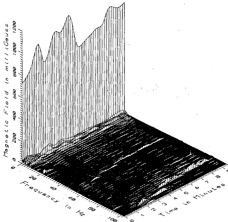
TR7010 - SEAT LEVEL - REAR ENGINE SECTION, CAR#2
