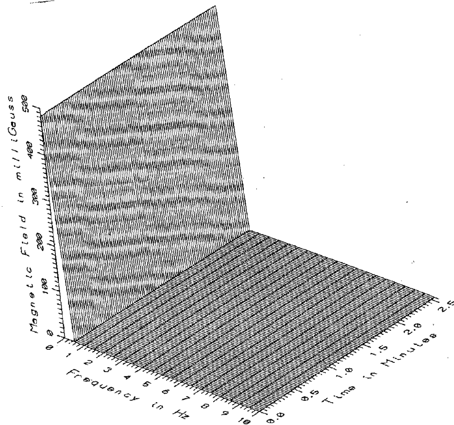
TR7018 - 10M WEST OF HIGH STEEL GUIDEWAY
