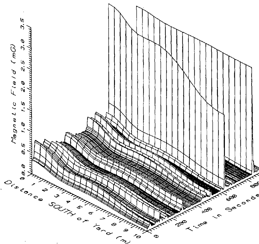
TR7022, OUTPUT TRANSFORMER YARD - POWER HARMONICS, 65-300Hz
