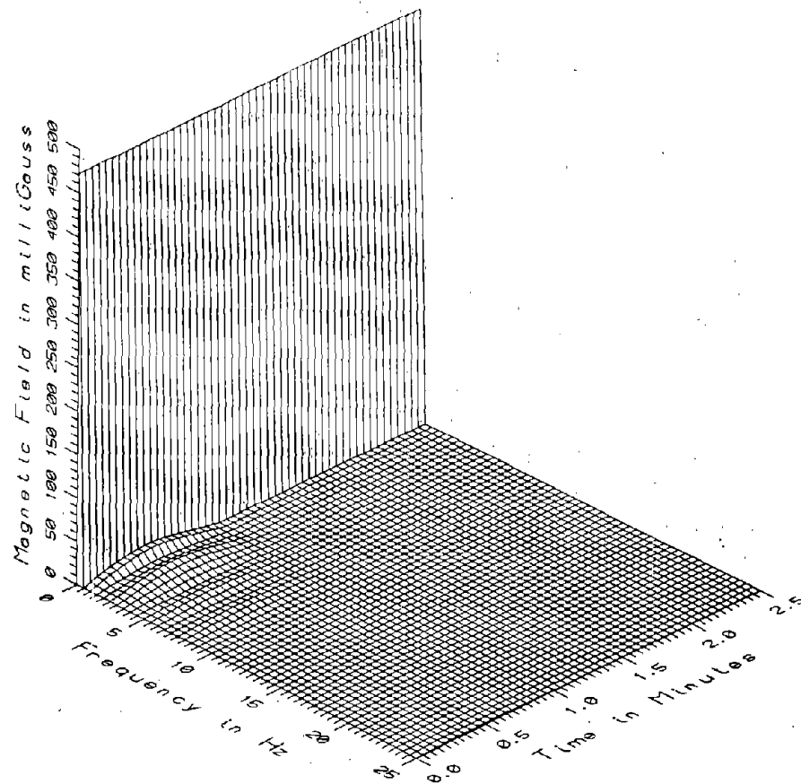
TR7012 - 3M WEST OF HIGH STEEL GUIDEWAY
