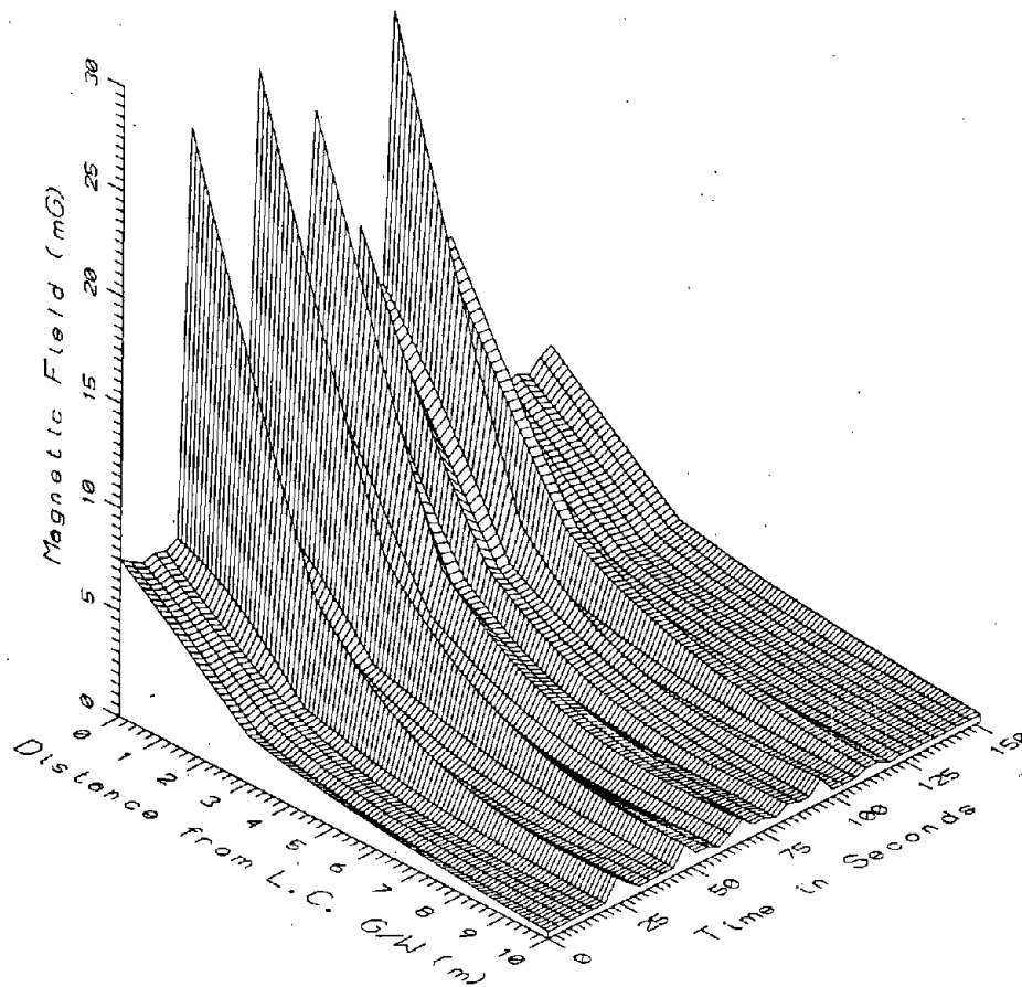
TR7026, LOW CONCRETE G/W OUTSIDE MAINTENANCE FACILITY - POWER FREQ, 60-300Hz
