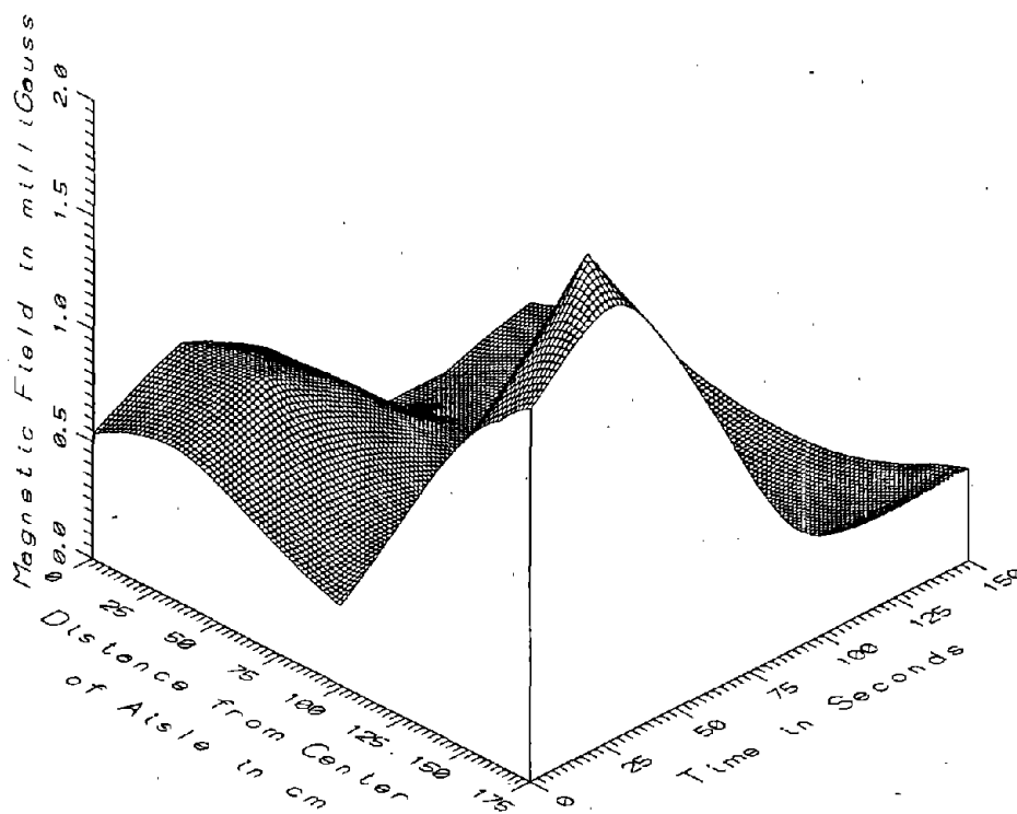
TR7011, FLOOR LEVEL IN MIDDLE OF PASSENGER SECTION, CAR2 - HIGH FREQ. 305-2560
