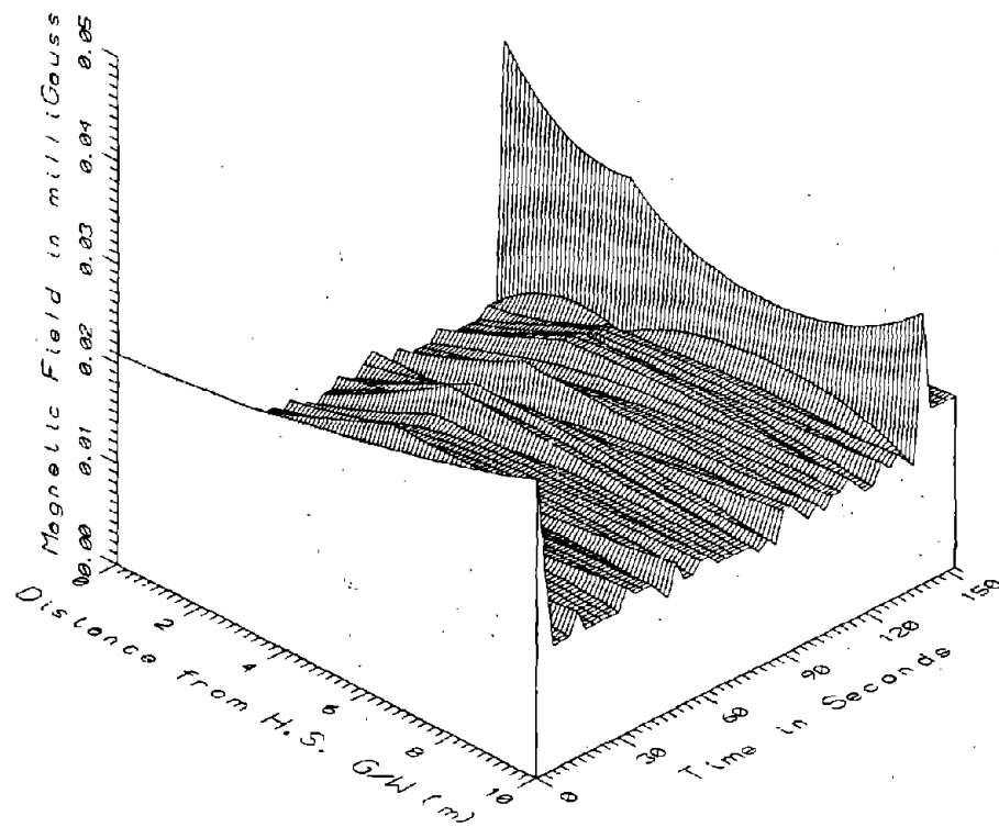
TR701B, HIGH STEEL GUIDEWAY - POWER HARMONICS, 65-300Hz
