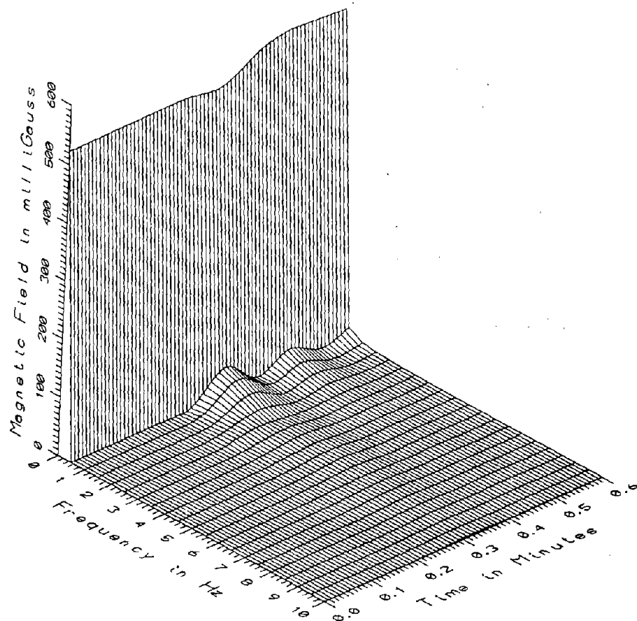
TR7025 - 10M NORTHWEST OF LOW CONCRETE GUIDEWAY OUTSIDE MAINTENANCE FACILITY
