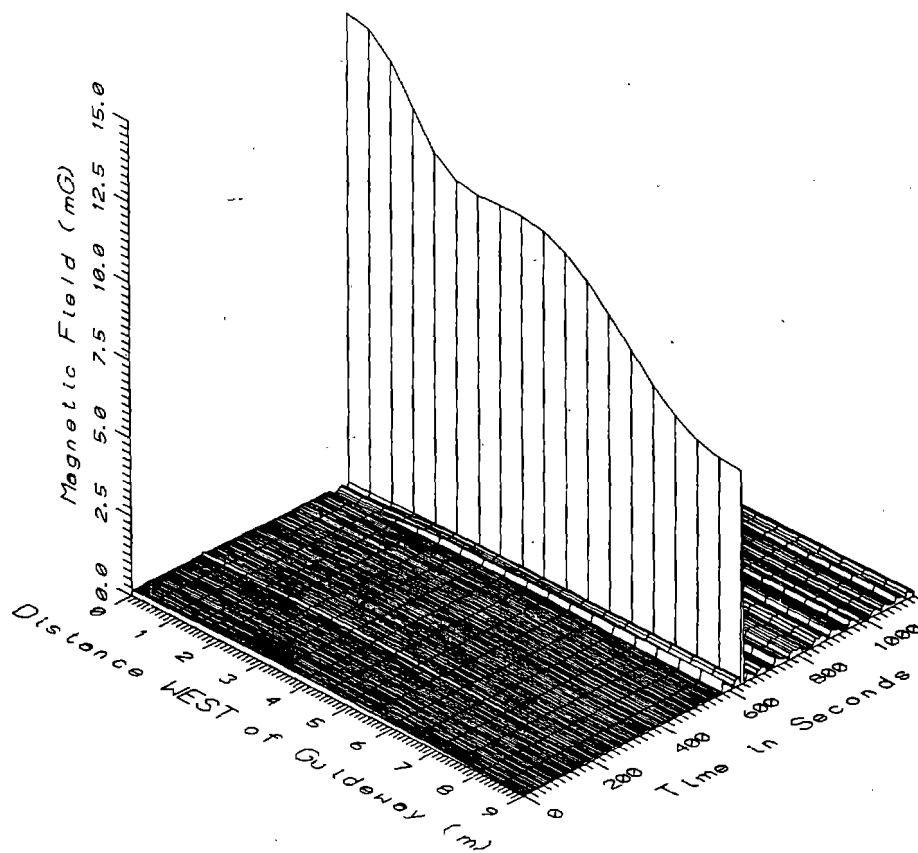
TR7021, GUIDEWAY AT LOADING PLATFORM - POWER FREQUENCY, 50-60Hz
