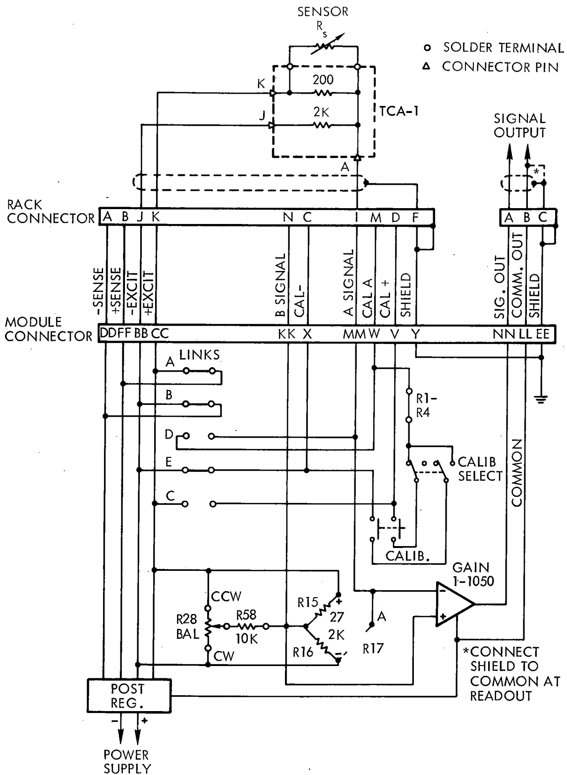
FIGURE F-6. MODE CARD SETUP FOR TEMPERATURE MEASUREMENTS
