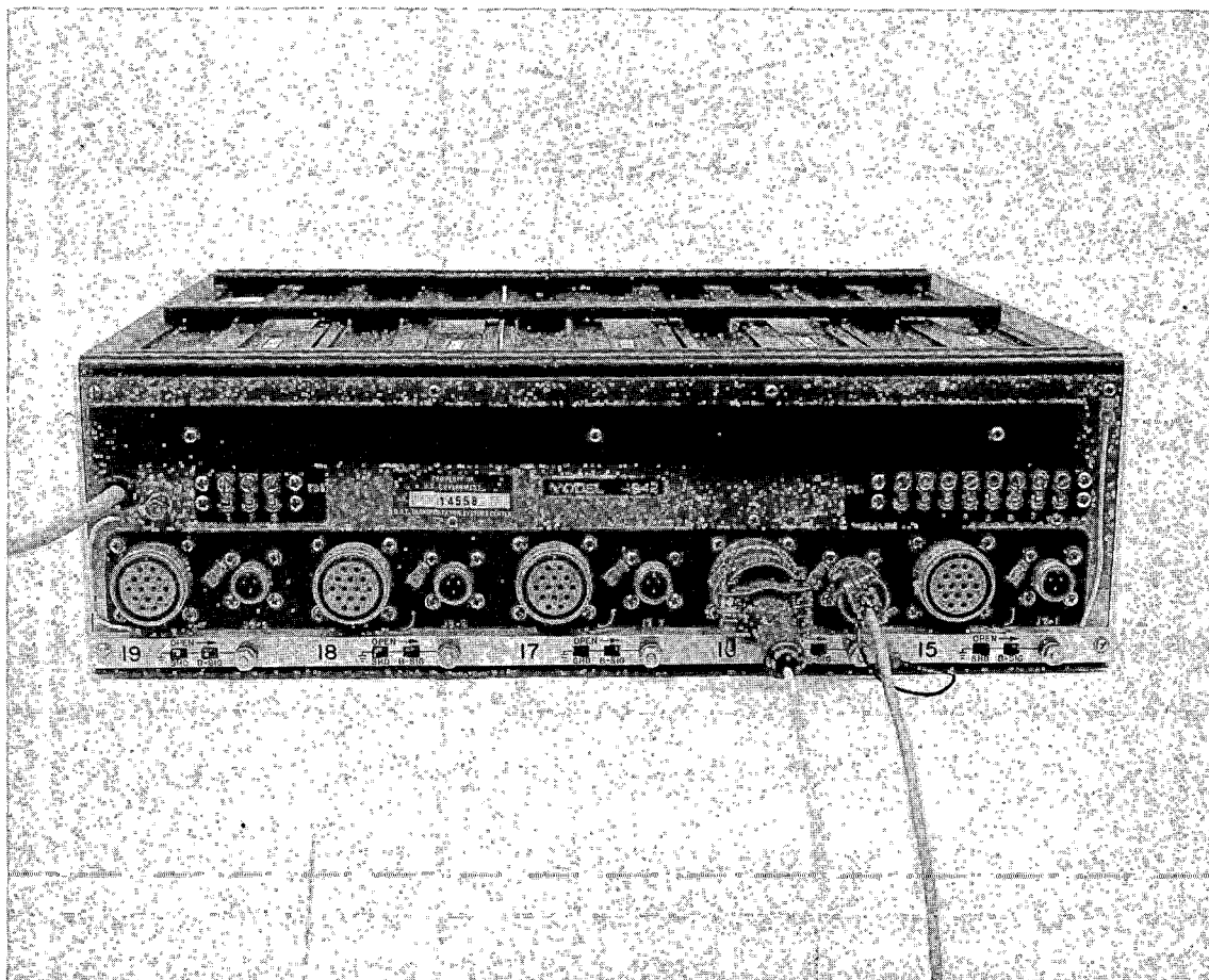
FIGURE 5-3. SHIELD/GROUND SWITCH PANEL
