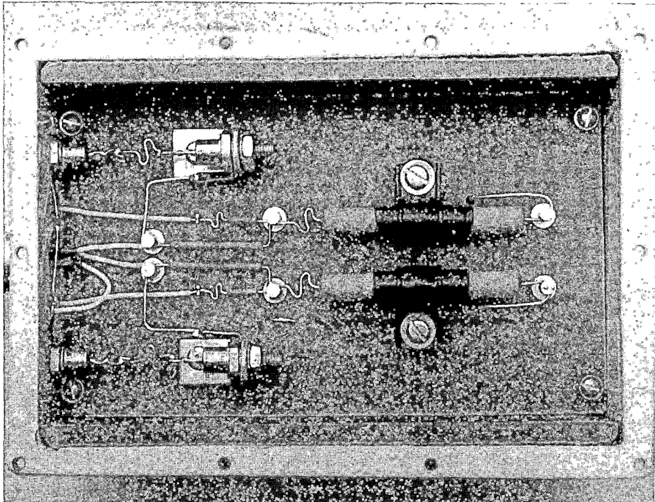
FIGURE C-7. TSC VOLTAGE DIVIDER COVER PLATE REMOVED, CIRCUIT EXPOSED
