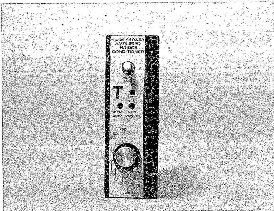
(Front Panel View)
