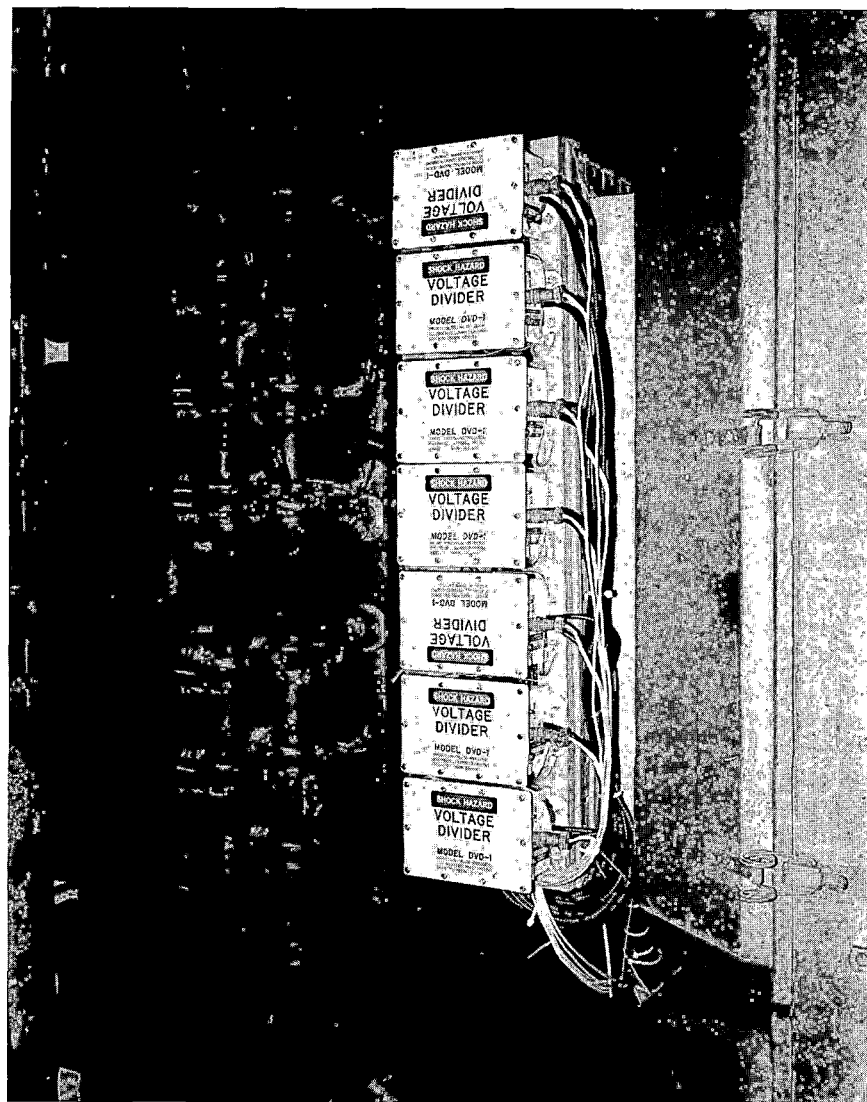
FIGURE C-6. TSC VOLTAGE DIVIDERS CUSTOM RACK MOUNTED ON R42 VEHICLES (VIEWED FROM MAINTENANCE PIT)
