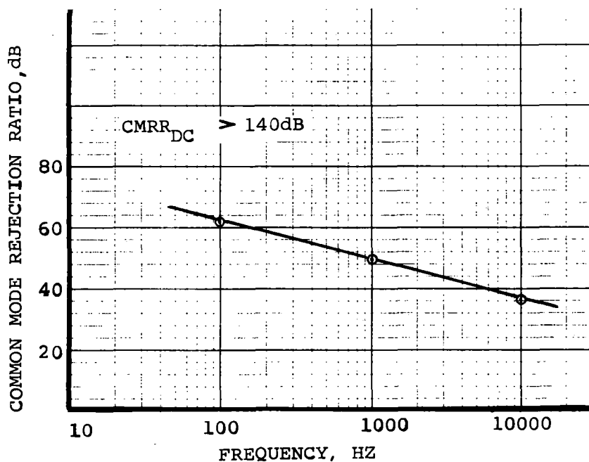
FIGURE B3-23. CURRENT SHUNT MEASUREMENT SYSTEM COMMON MODE REJECTION RATIO
