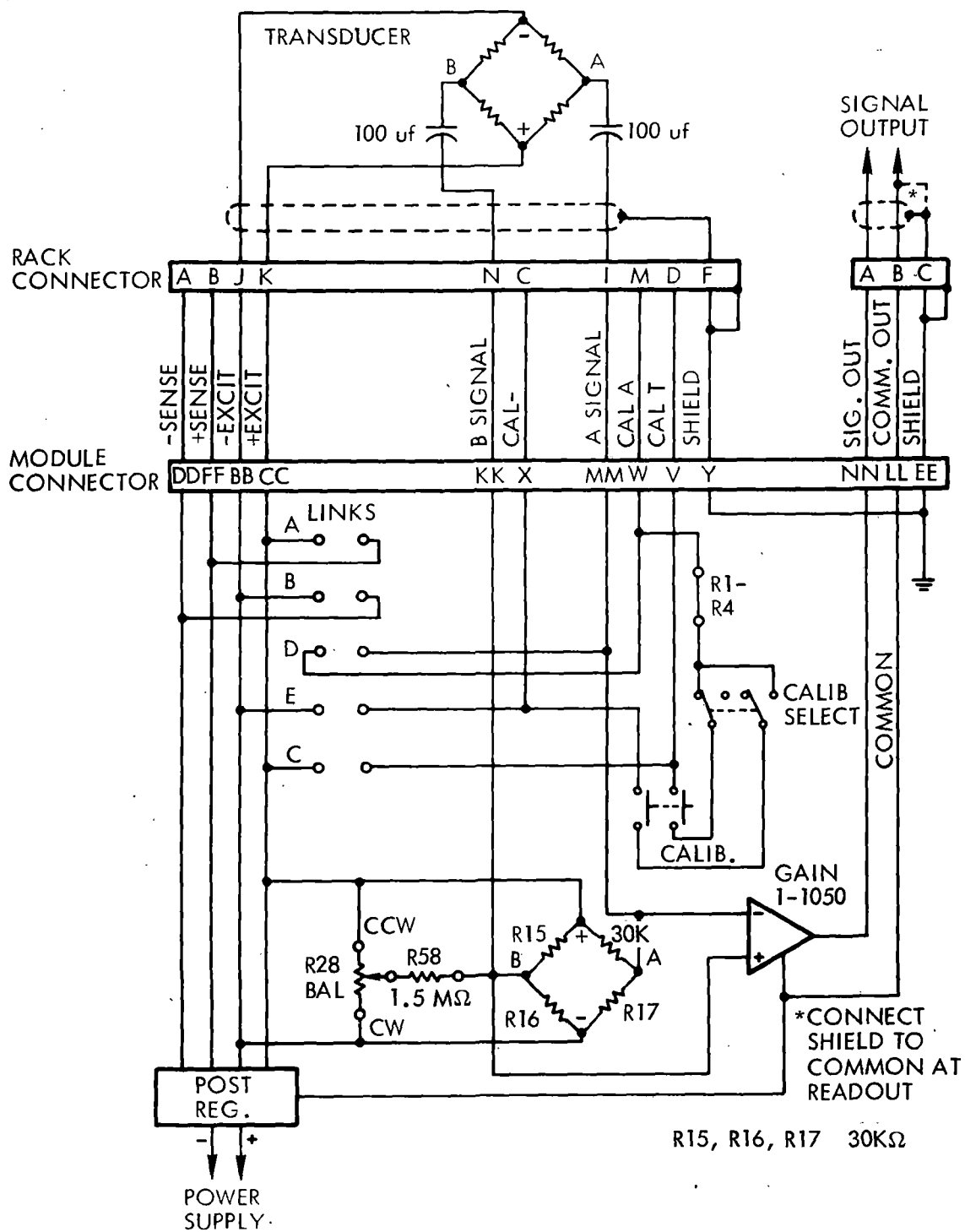
Figure G1-5. GVT Mode Card Setup for Strain Measurement
