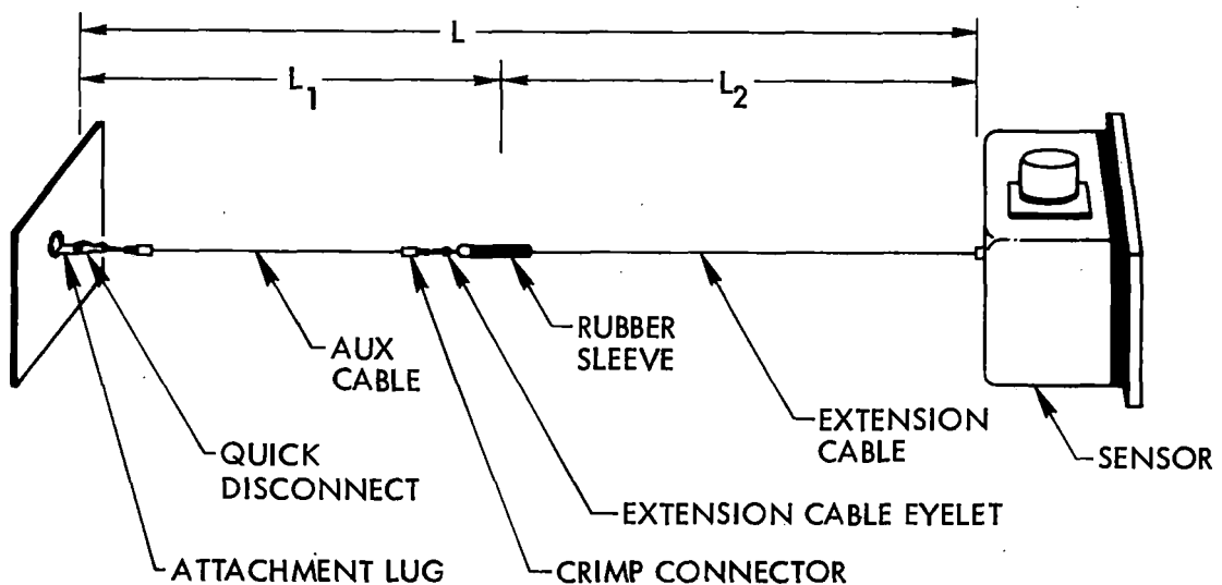
FIGURE G2-6. AUXILIARY COUPLING CABLE AS USED IN WIDELY SEPARATED PARALLEL PLANES SITUATION
