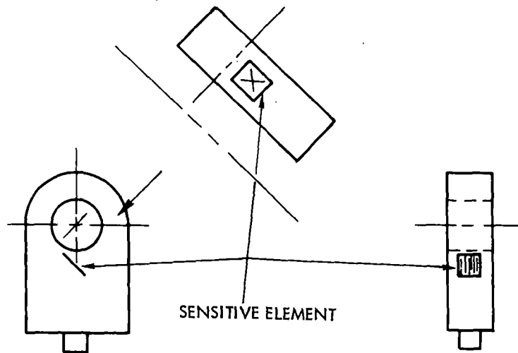
a. ORIENTATION OF SENSITIVE AXIS, SERIES 909 (NOT TO SCALE)
