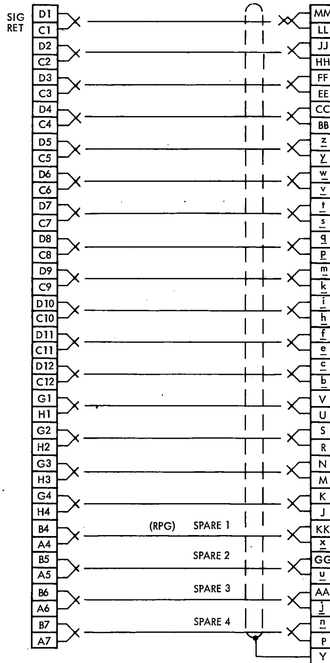
FIGURE A1-3. GVT CABLE STYLE R PHYSICAL/ FUNCTIONAL CHARACTERISTICS
