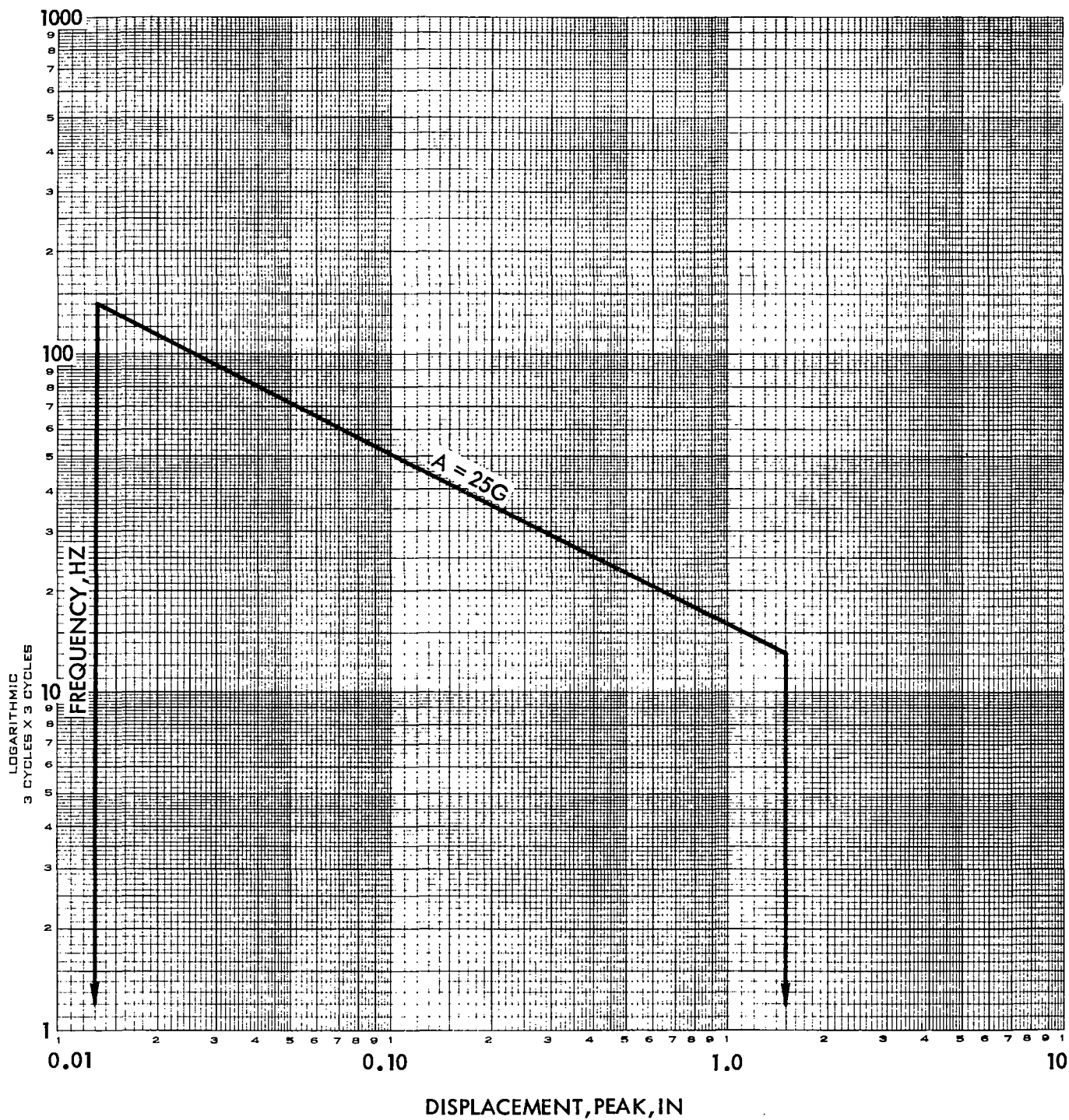
FIGURE G2-11. USEFUL MEASUREMENT RANGE FOR MODEL PT101-3A POTENTIOMETER DISPLACEMENT SENSOR
