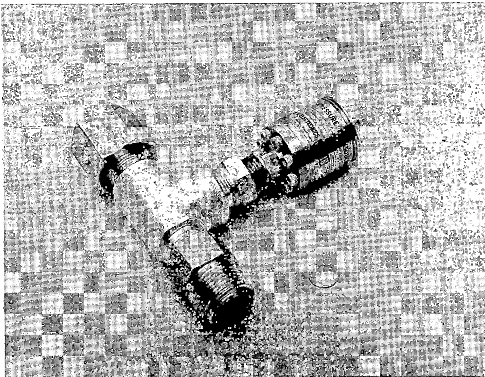
FIGURE E2. PRESSURE CELL AND INTERFACE HARDWARE
