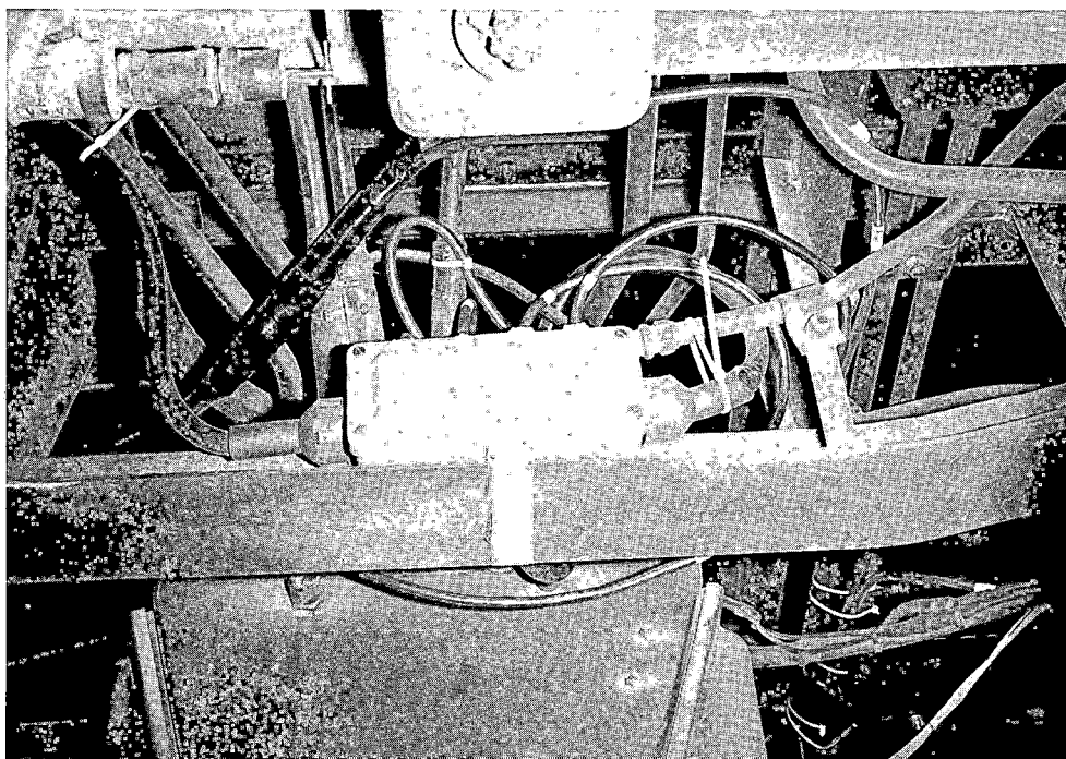
FIGURE B3-17. A CURRENT SHUNT INSTALLATION ON THE R42 VEHICLE
