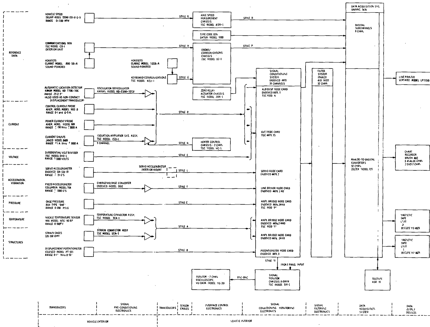
FIGURE 2-1. GENERAL VEHICLE TEST SYSTEM BLOCK DIAGRAM
