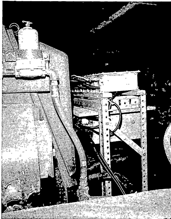
FIGURE B3-19. TYPICAL ISOLATION AMPLIFIER MOUNTING METHOD
