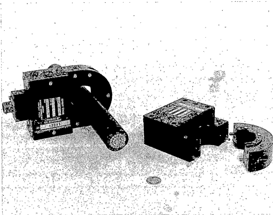
FIGURE B2-1. POWER CURRENT SENSOR - (LEFT) AS SEEN IN USE, (RIGHT) YOKE OPENED FOR INSTALLATION ON POWER CONDUCTOR
