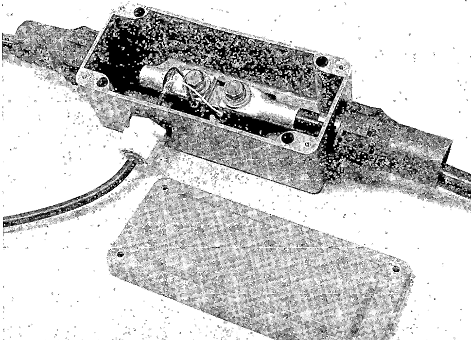
FIGURE B3-11. TYPICAL CURRENT SHUNT INSTALLATION INSIDE WEATHERPROOF, INSULATING JUNCTION BOX
