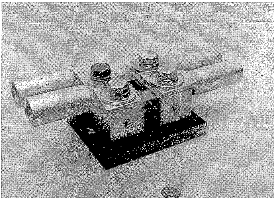
FIGURE B3-16. TYPICAL CABLE ATTACHMENT TECHNIQUE FOR TYPE 8406D CURRENT SHUNT
