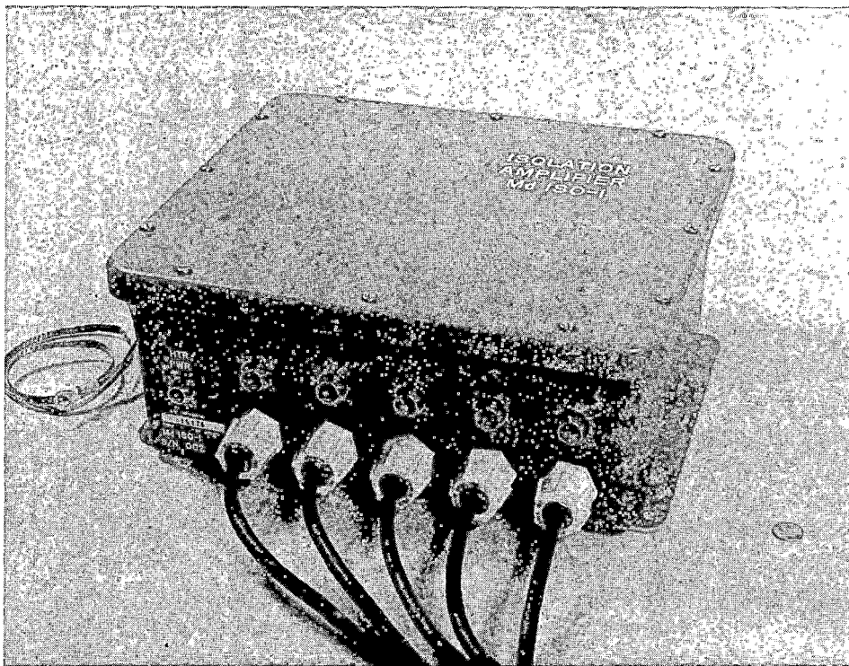
FIGURE B3-2. ISOLATION AMPLIFIER
