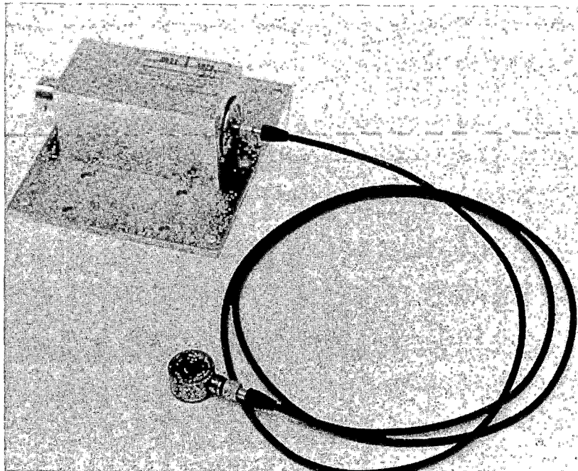
FIGURE D2-2. PIEZO ACCELEROMETER/CABLE/CHARGE CONVERTER/MOUNT ASSEMBLY, PRIOR TO INSTALLATION
