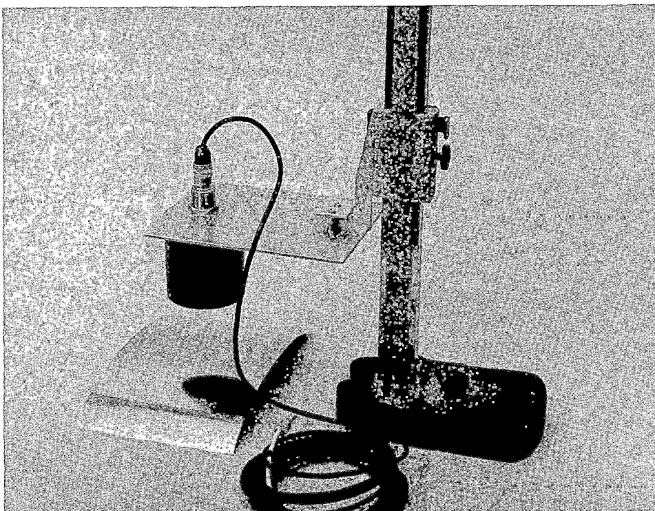
FIGURE G3-2. LABORATORY SIMULATION OF IN-SITU CALIBRATION
