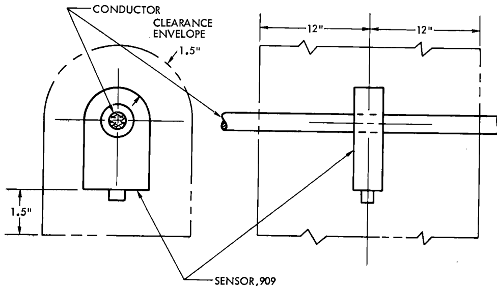
FIGURE B2-5. CONDUCTOR POSITIONING IN SENSOR AND CLEARANCE ENVELOPE REQUIREMENTS
