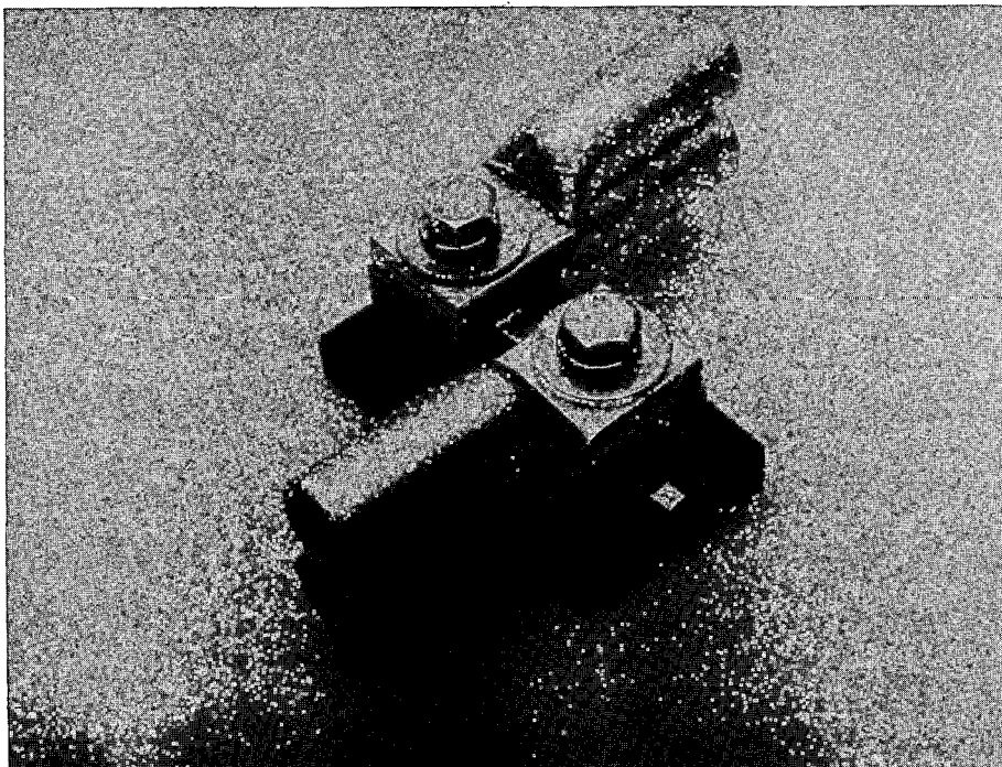
FIGURE B3-15. TYPICAL CABLE ATTACHMENT TECHNIQUE FOR TYPE 8406C CURRENT SHUNT
