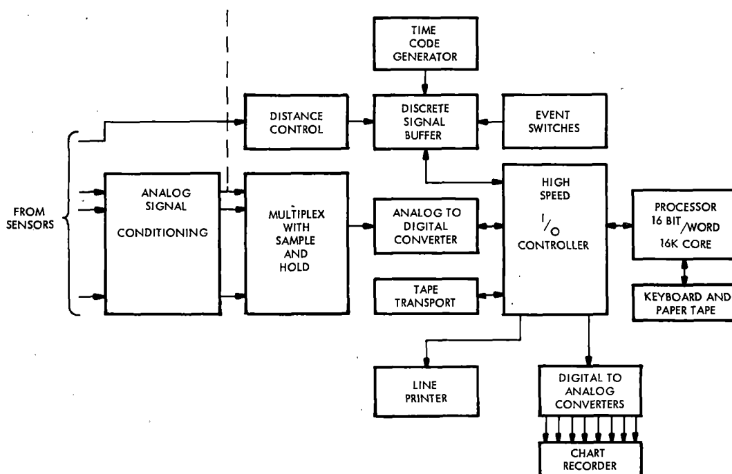
FIGURE 2-4. DATA ACQUISITION SYSTEM BLOCK DIAGRAM
