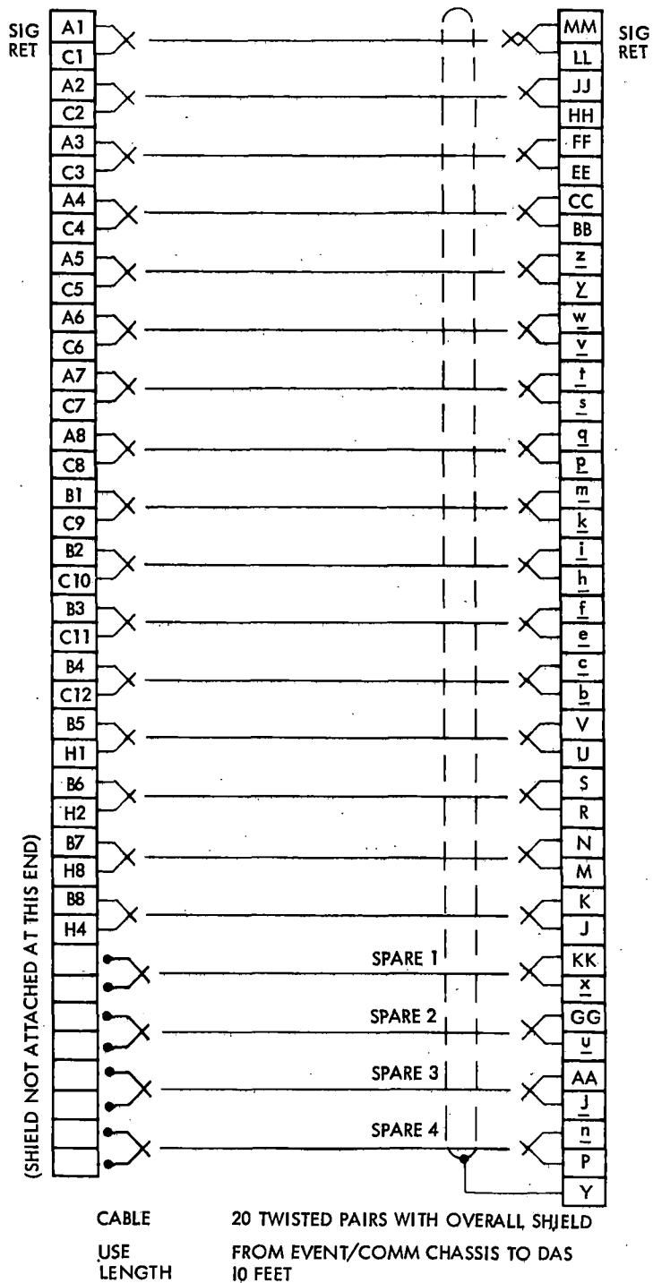
FIGURE A2-6. GENERAL VEHICLE TEST CABLE STYLE P
