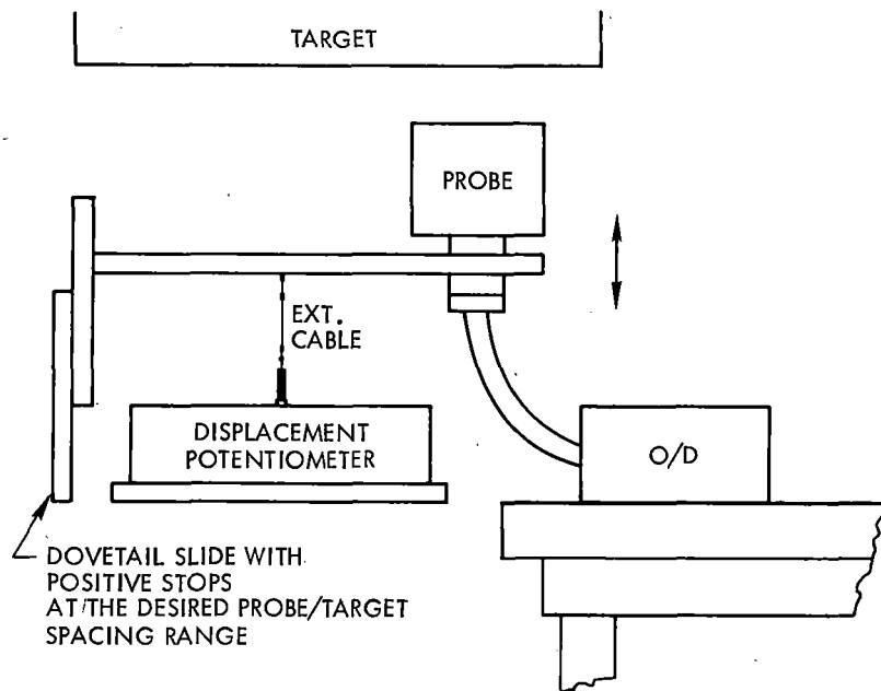
FIGURE G3-3. SAMPLE MECHANICAL LAYOUT FOR SWEEPED CALIBRATION
