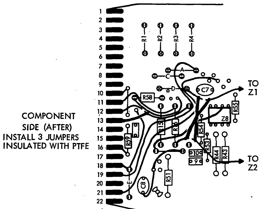
FIGURE F-5. MODE CARD SETUP- COMPONENT BOARD MODIFICATIONS
