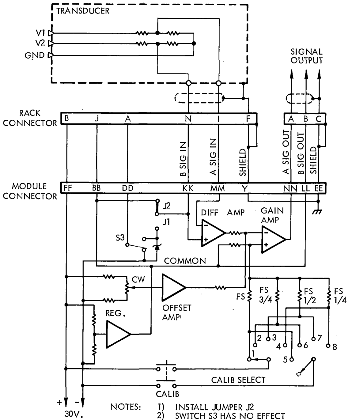
FIGURE C-5. GVT MODE CARD SETUP FOR VOLTAGE MEASUREMENT SYSTEM
