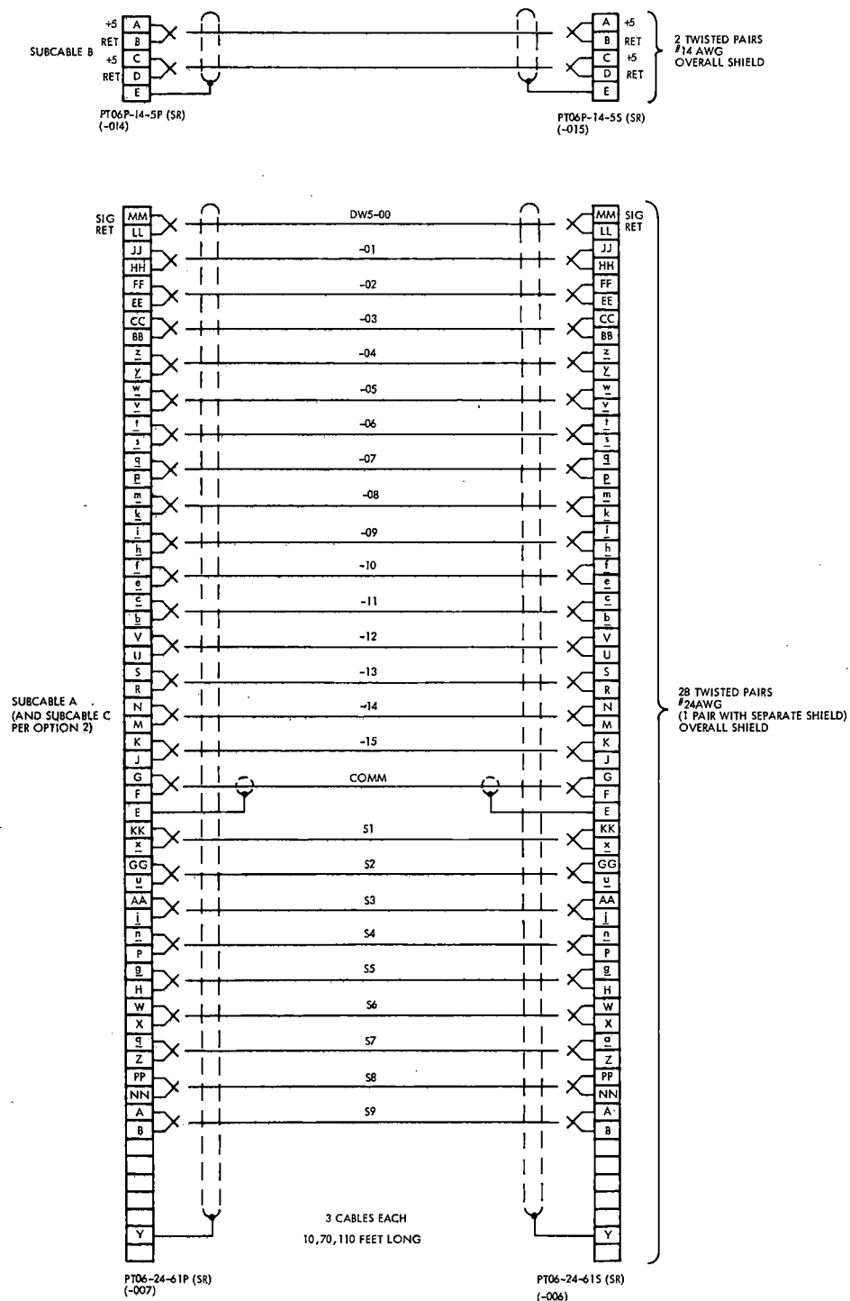
FIGURE A2-5. GENERAL VEHICLE TEST CABLE STYLE G
