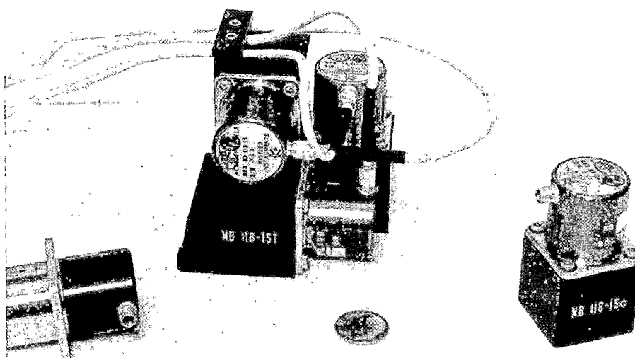
FIGURE D1-2. Q-FLEX ACCELEROMETERS INSTALLED IN MOUNTING BLOCKS
