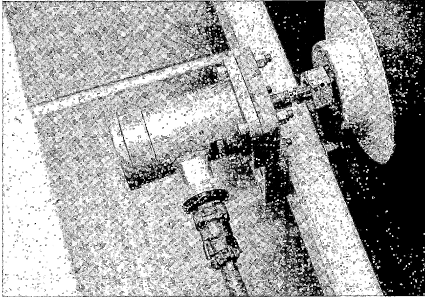
FIGURE A1-6. RPG MOUNTED ON THE PCC VEHICLE
