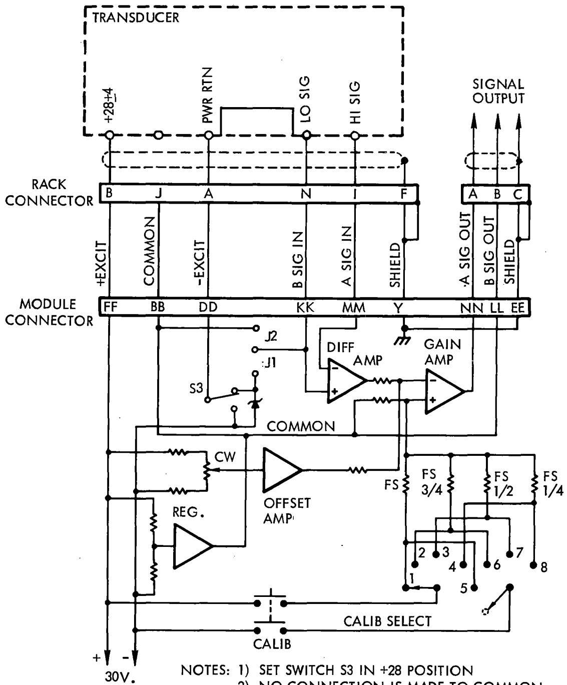
FIGURE B1-5. GVT MODE CARD SETUP FOR CONTROL CURRENT MEASUREMENT SYSTEM
