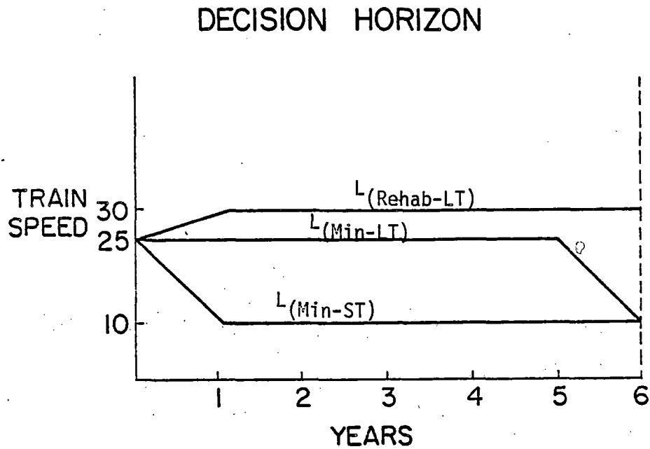
Figure 6. Branch Line (N) Speed Deterioration Curves for Levels of Investment (L)
