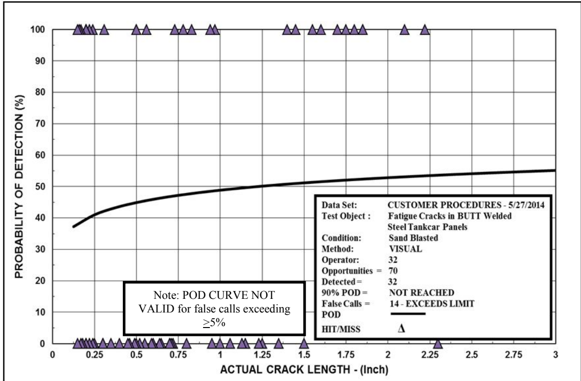
Figure 5. VT Butt Weld POD Results for Operator 32
