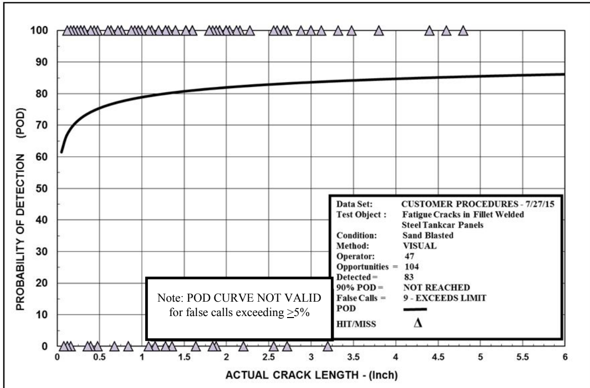
Figure 20. VT Fillet Weld POD Results for Operator 47
