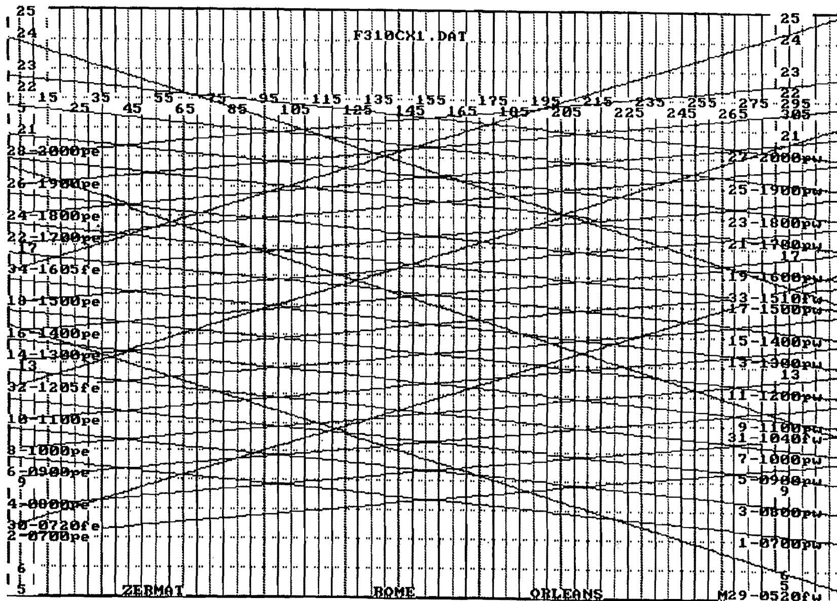
Figure 7-13. Case C: Stringline, 150-mph Passenger Train Speeds
