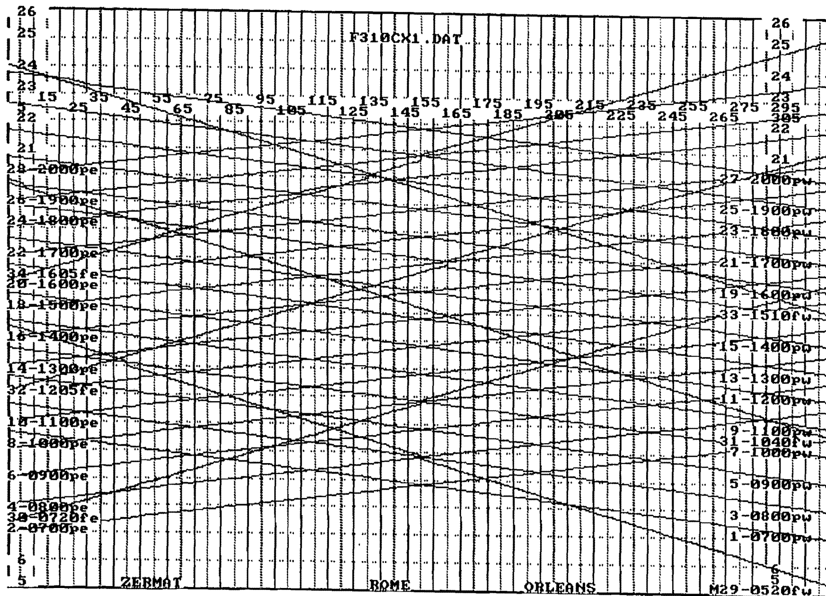
Figure 7-11. Case C: Stringline, 110-mph Passenger Train Speeds
