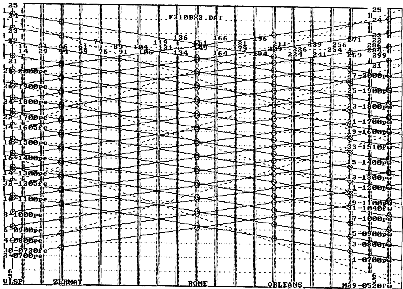
Figure 7-7. Case B: Stringline, 90-mph Passenger Train Speeds
