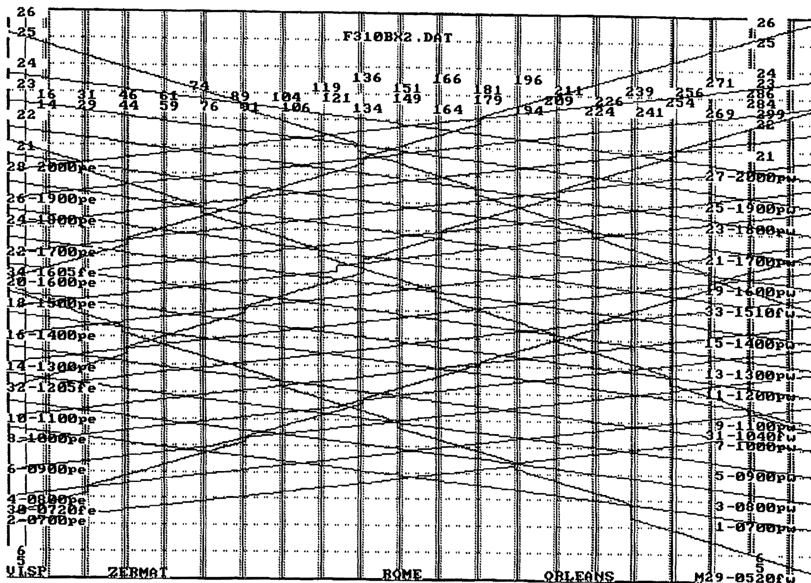
Figure 7-8. Case B: Stringline, 110-mph Passenger Train Speeds
