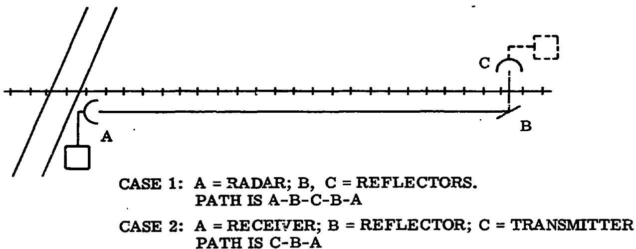
Figure 4.24. - More Elaborate Beam Interruption Method
