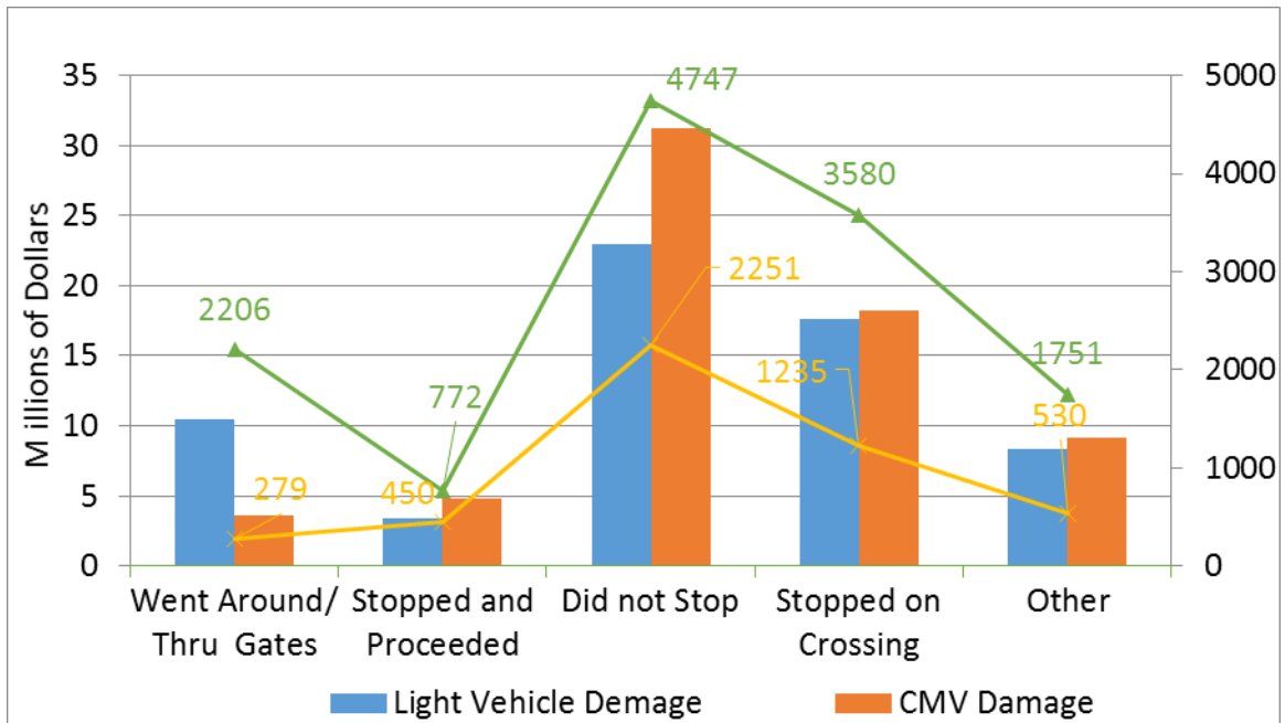
Figure 19. HRI Incident Cost, in Millions of Dollars, by Crash Mechanism for Light and Commercial Vehicles and the Number of Incidents at All Crossing Type as a Function of Vehicle Type, from 2008–2017
