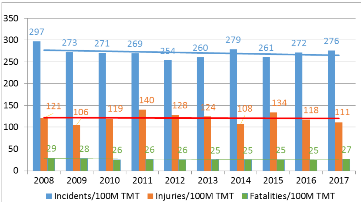
Figure 6. Public and Private HRI Incident and Casualty Rates per 1,000 HRIs, from 2008–2017, Excluding Pedestrians
