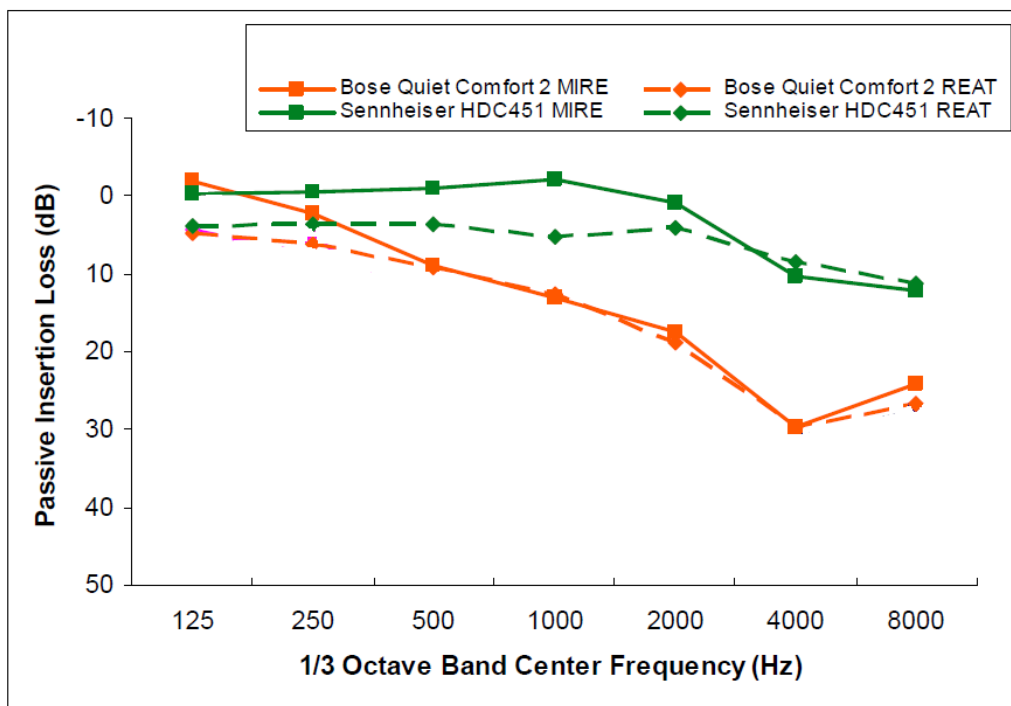
Figure 13. Measured Passive Noise Reduction of Headphones (Perala, 2009)
