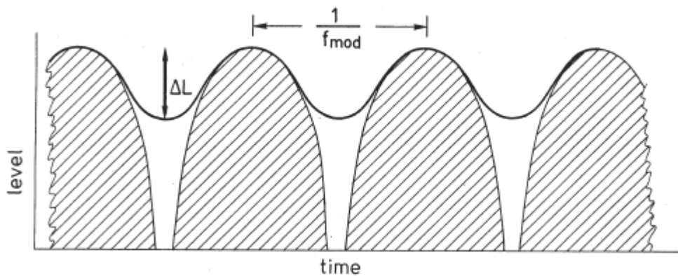
Figure 11. Depiction of Acoustic Roughness (Fastl, 2005)
