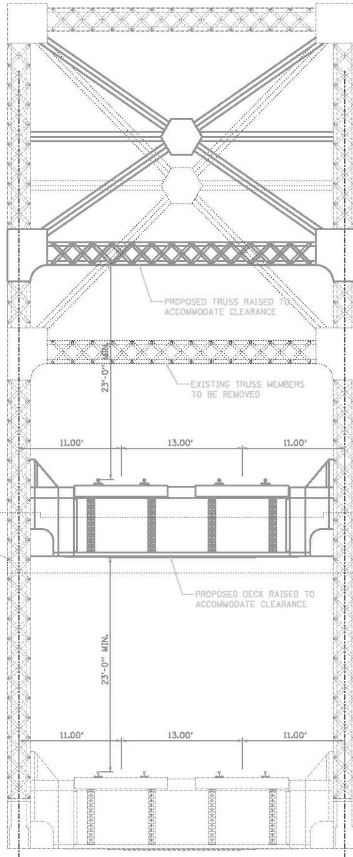
ALTERNATE 1 - DOUBLE DECKING EXISTING MACARTHUR BRIDGE
