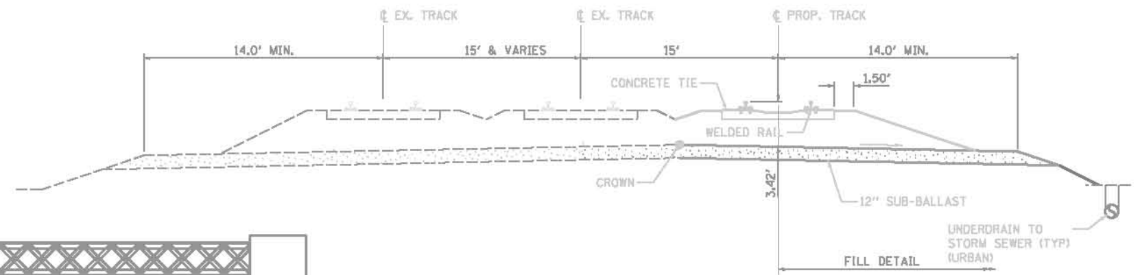
ADDITIONAL TRACK TO EXISTING 2-TRACK
