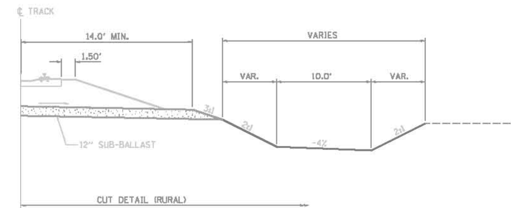
CONCEPT DRAWINGS ONLY
