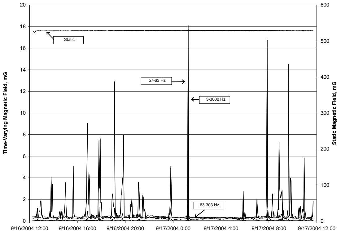
Figure C2. 24-Hour Fluctuation of Static and Time-Varying Magnetic Field Levels at the Westbrook SwS
