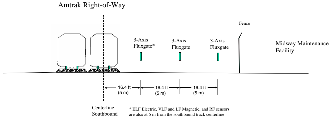
Figure 2. Sketch of ELF Magnetic Field Sensor (Three-Axis Fluxgate) Positions Used for the Train Pass Measurements, Looking West Toward New London
