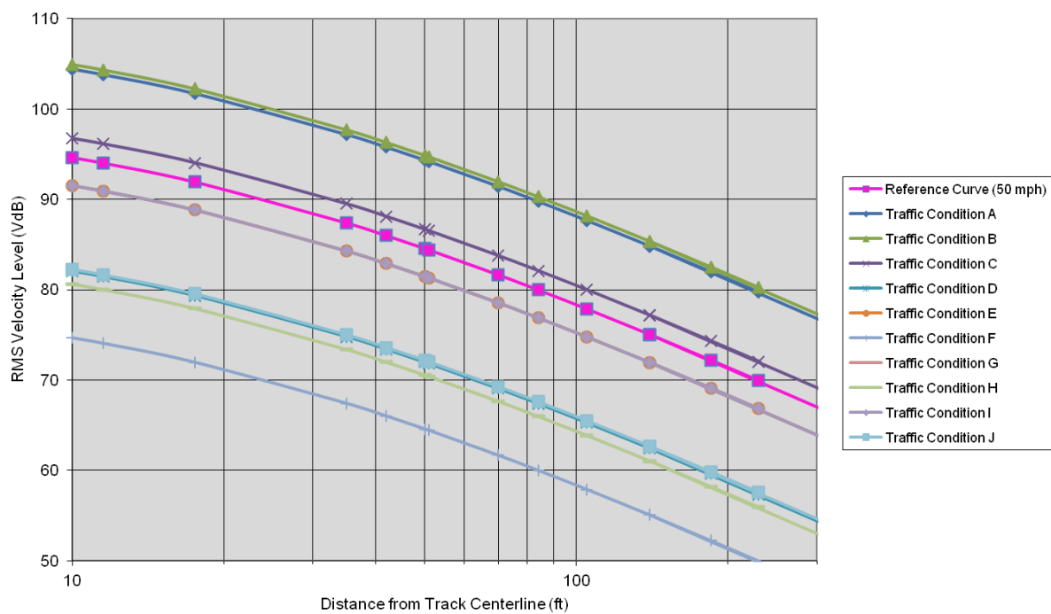
Chart 1 Ground Surface Vibration Curves - Existing Use
