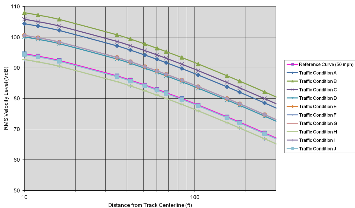
Chart 3 Ground Surface Vibration Curves - Future Build Condition
