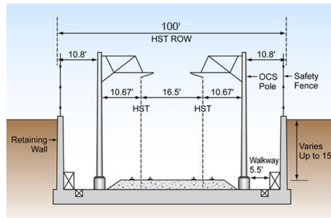
Figure 2-8 Retained-cut typical cross section
