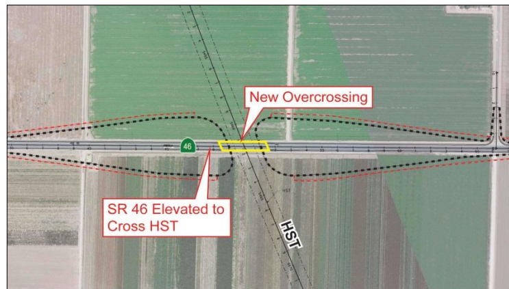
Figure 2-45 State Route 46 reconfiguration
