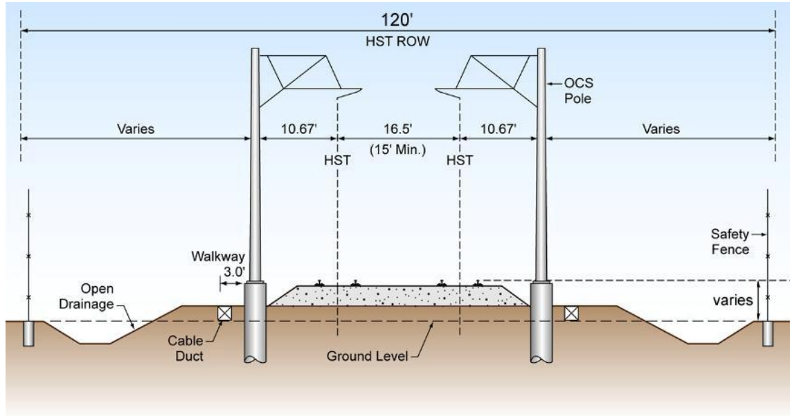
Figure 2-6 At-grade typical cross section
