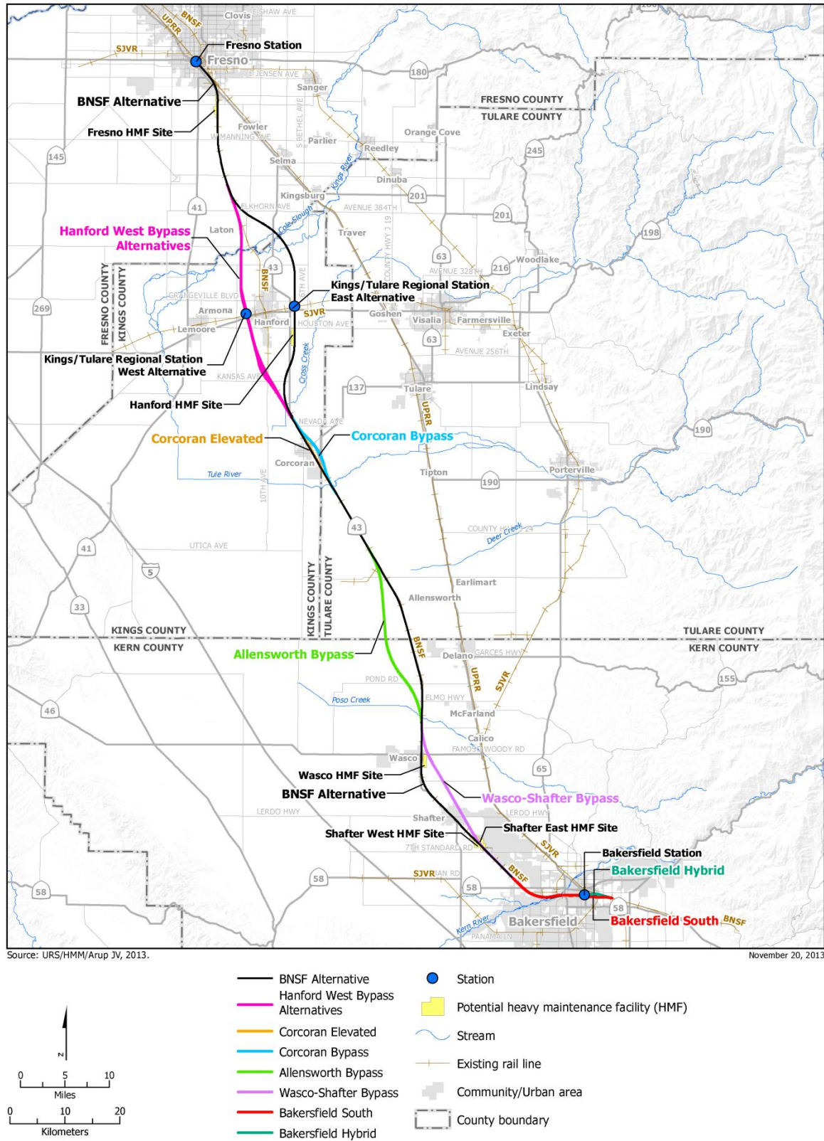
Figure 2-21 HST alternatives and HMF sites carried forward for further study
