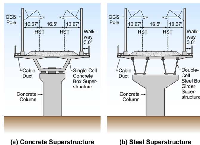
Figure 2-9 Elevated structure typical cross sections
