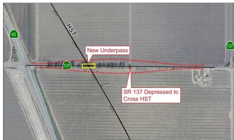
Figure 2-46 State Route 137 reconfiguration
