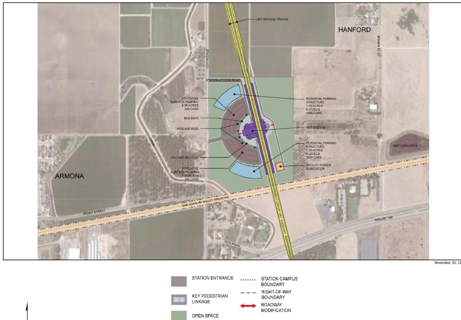
Figure 2-38 Kings/Tulare Regional Station–West Alternative (at-grade)
