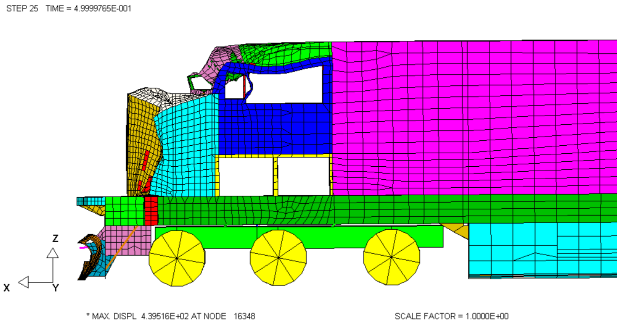
Figure 35. Lateral view of the deformed locomotive at the end of simulation (0.5 second) for the 50 mph collision
