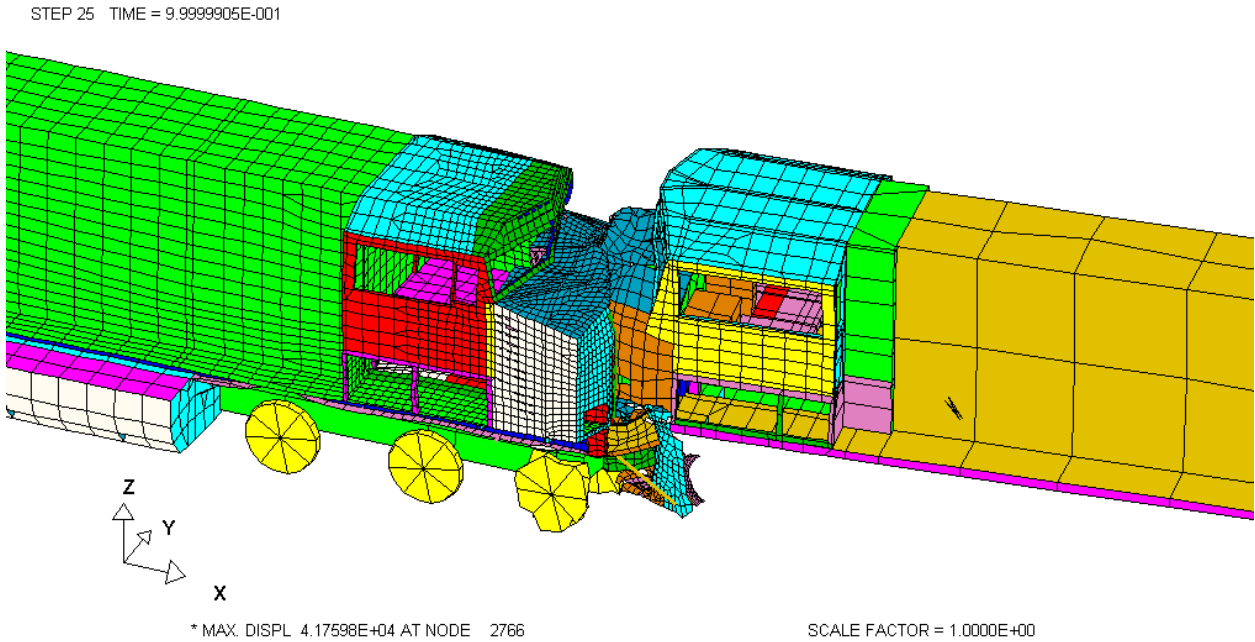
Figure 37. Close-up of the deformations of both locomotives at the end of simulation (1 second) for the 50 mph collision
