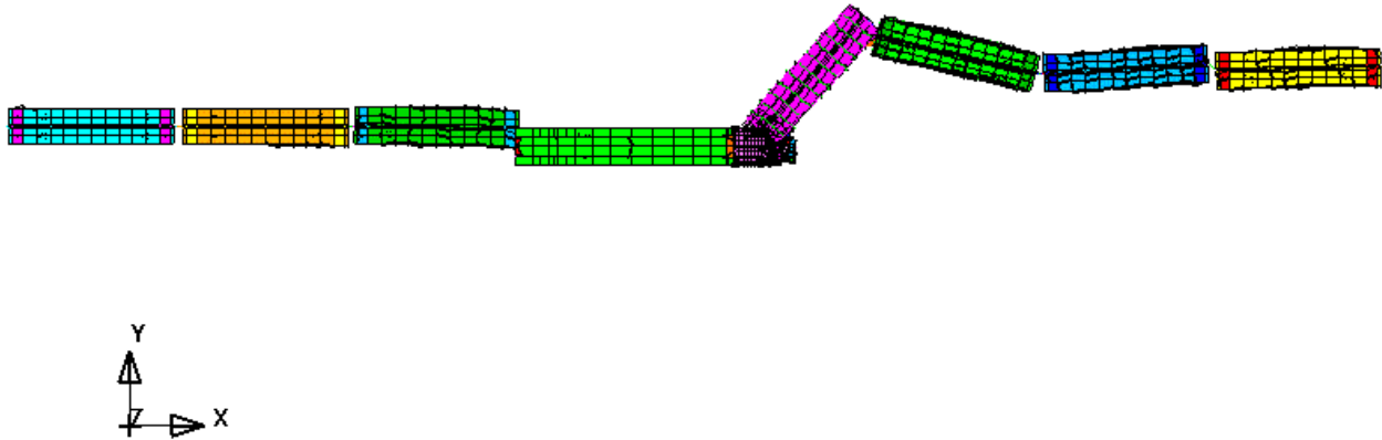
Figure 39. Top view of the locomotive and hopper consists at t = 1 second for the 30 mph case
